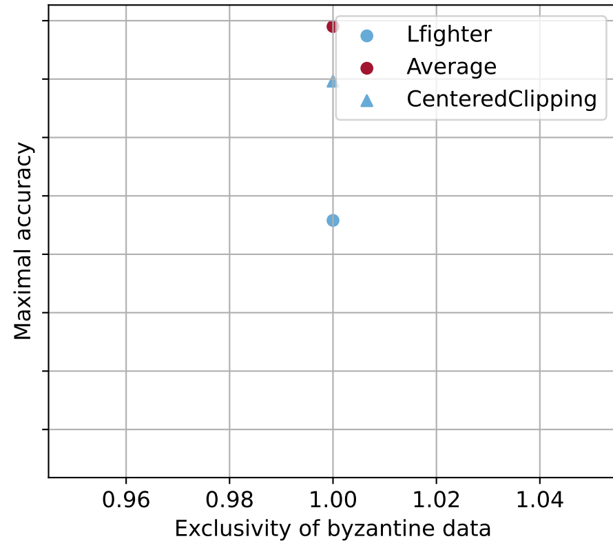
NoAttack attack
