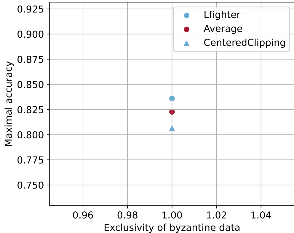
StaticLabelFlipping attack
