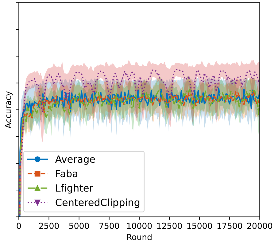
DynamicLabelFlipping attack
