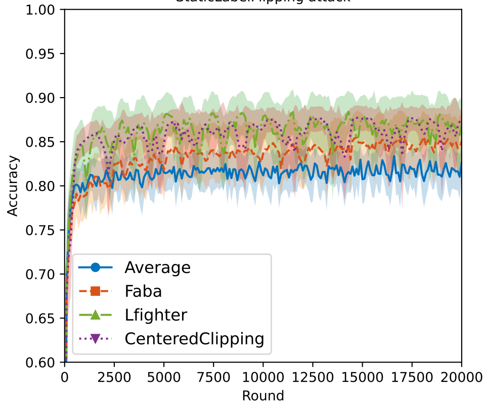
StaticLabelFlipping attack
