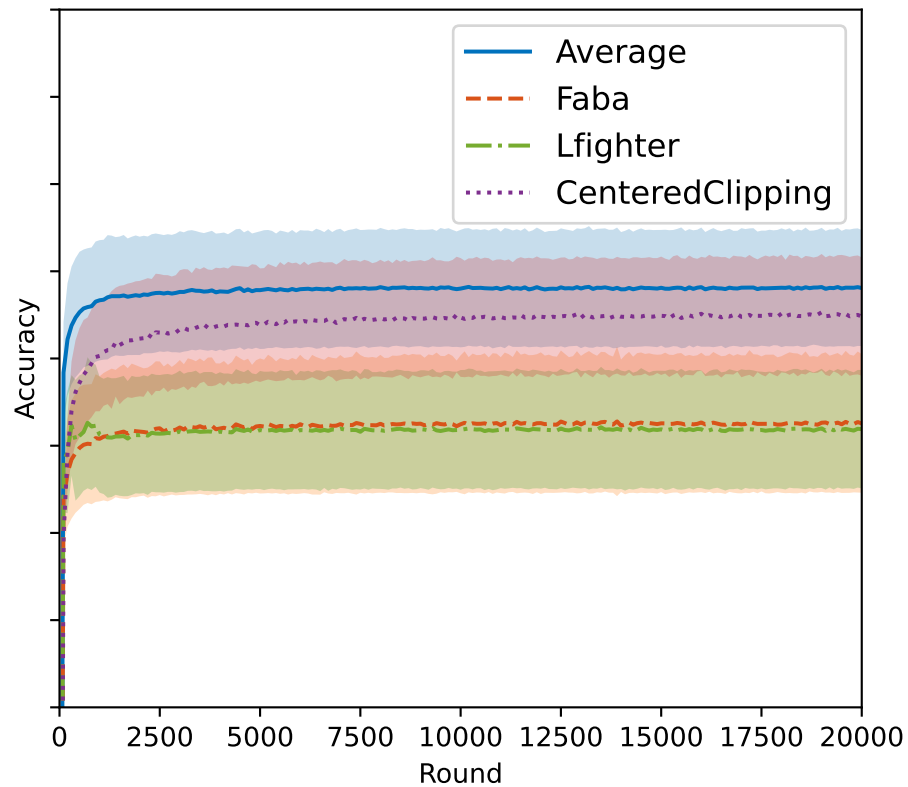
DynamicLabelFlipping attack
