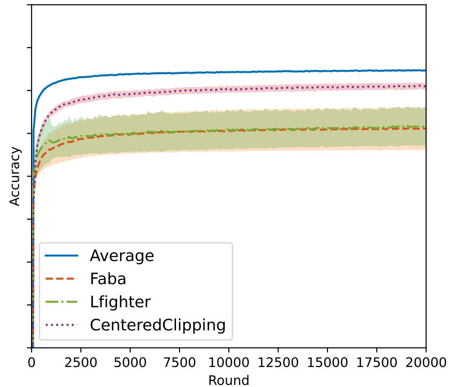
NoAttack attack
