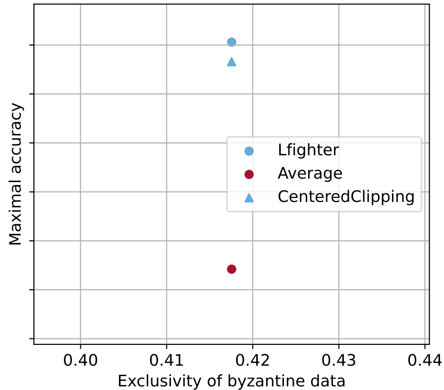
DynamicLabelFlipping attack
