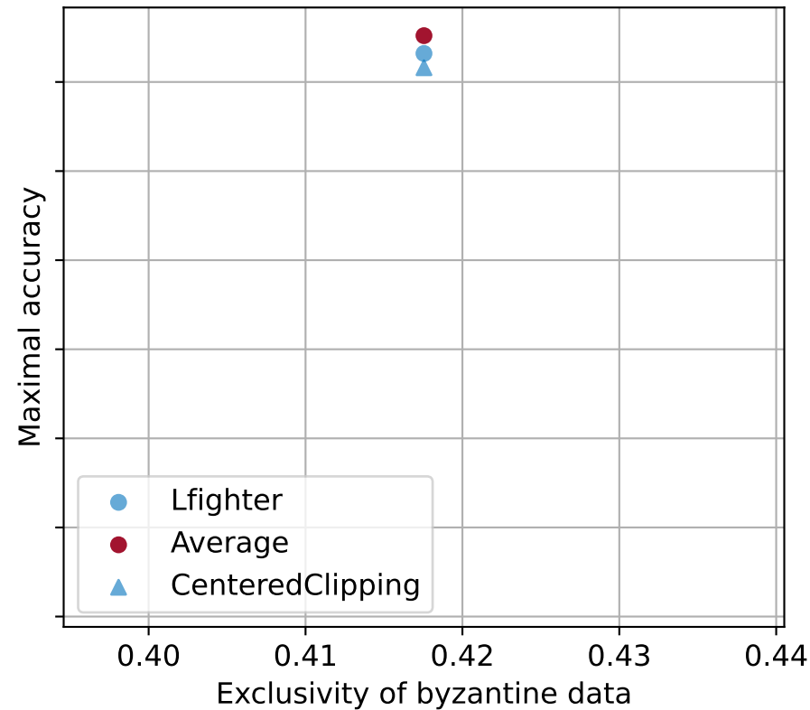
NoAttack attack
