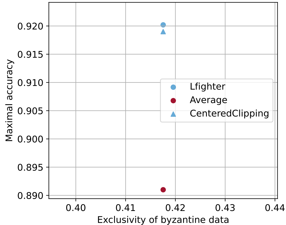
StaticLabelFlipping attack
