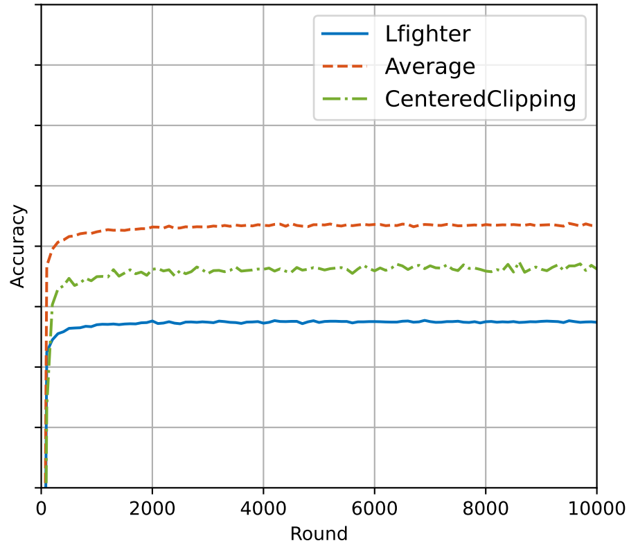
DynamicLabelFlipping attack
