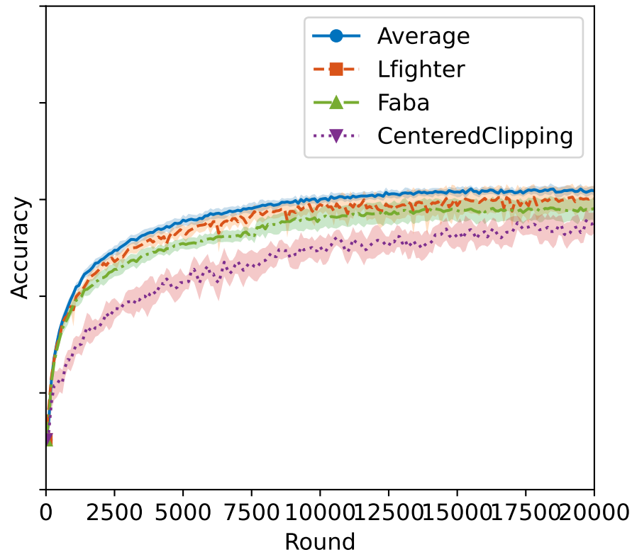
StaticLabelFlipping attack
