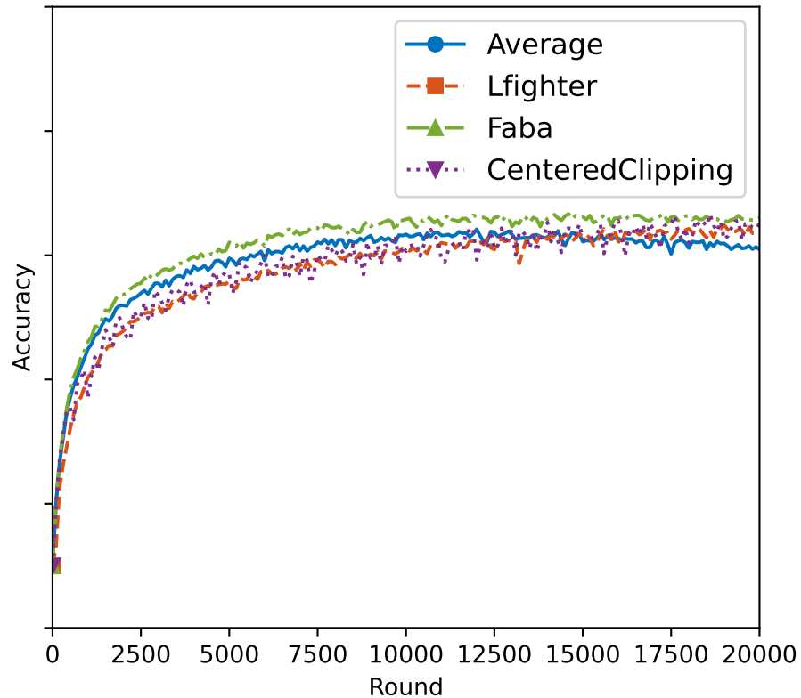
StaticLabelFlipping attack
