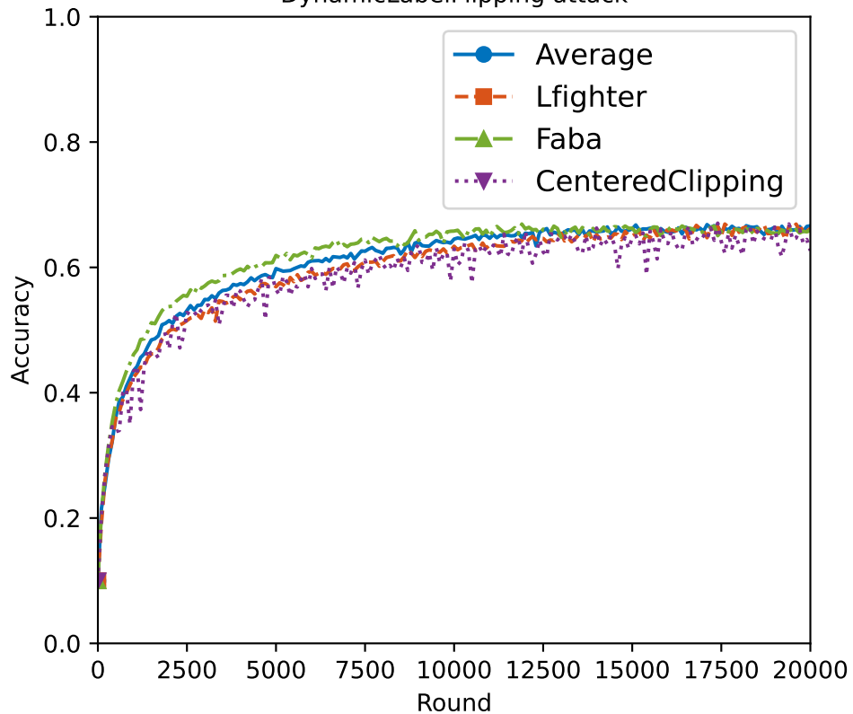
DynamicLabelFlipping attack
