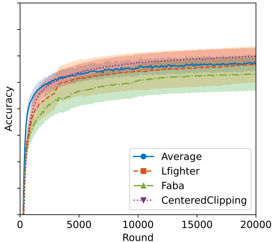
StaticLabelFlipping attack
