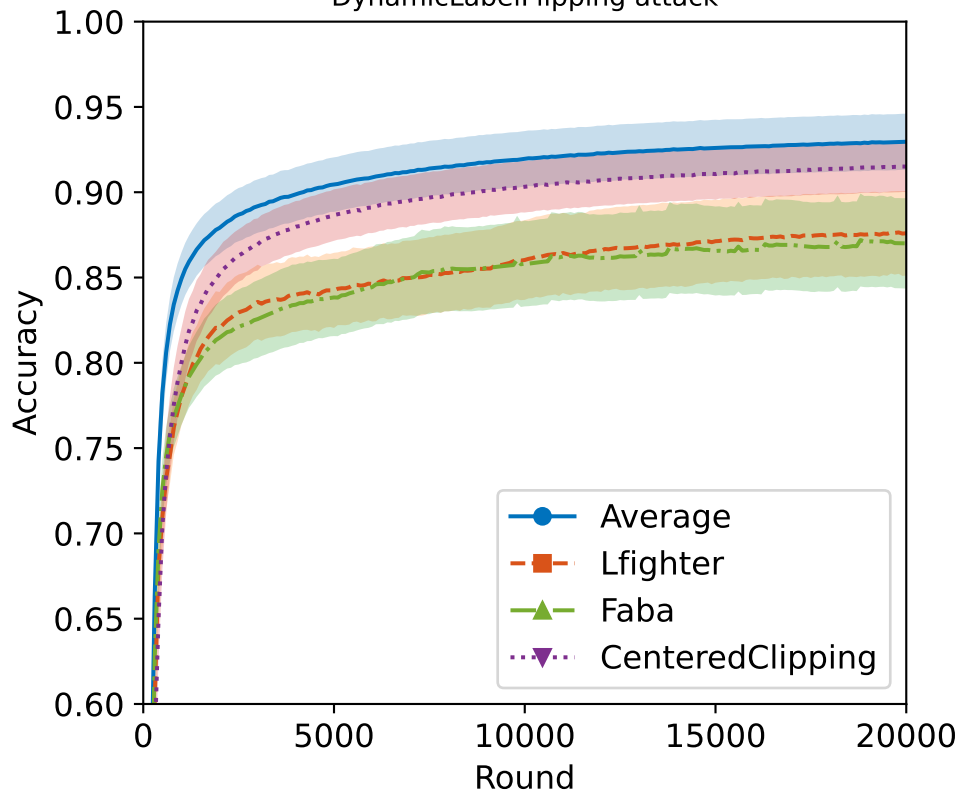
DynamicLabelFlipping attack
