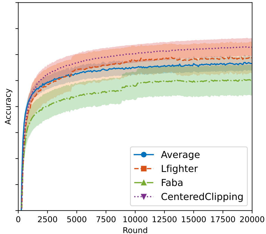
StaticLabelFlipping attack
