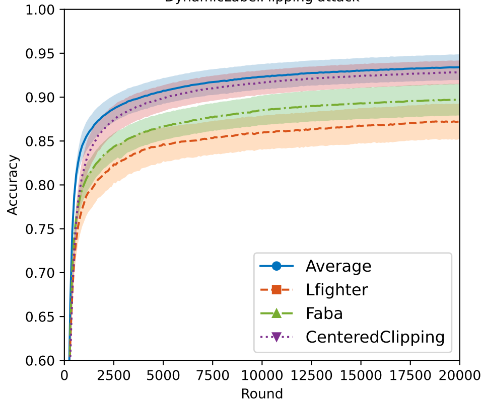
DynamicLabelFlipping attack
