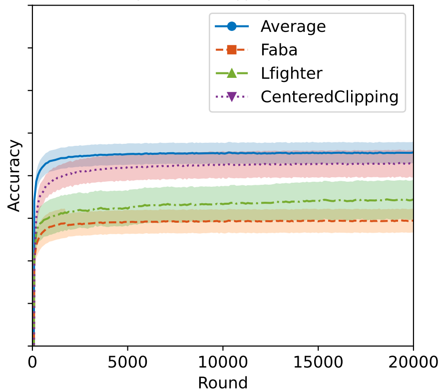
DynamicLabelFlipping attack
