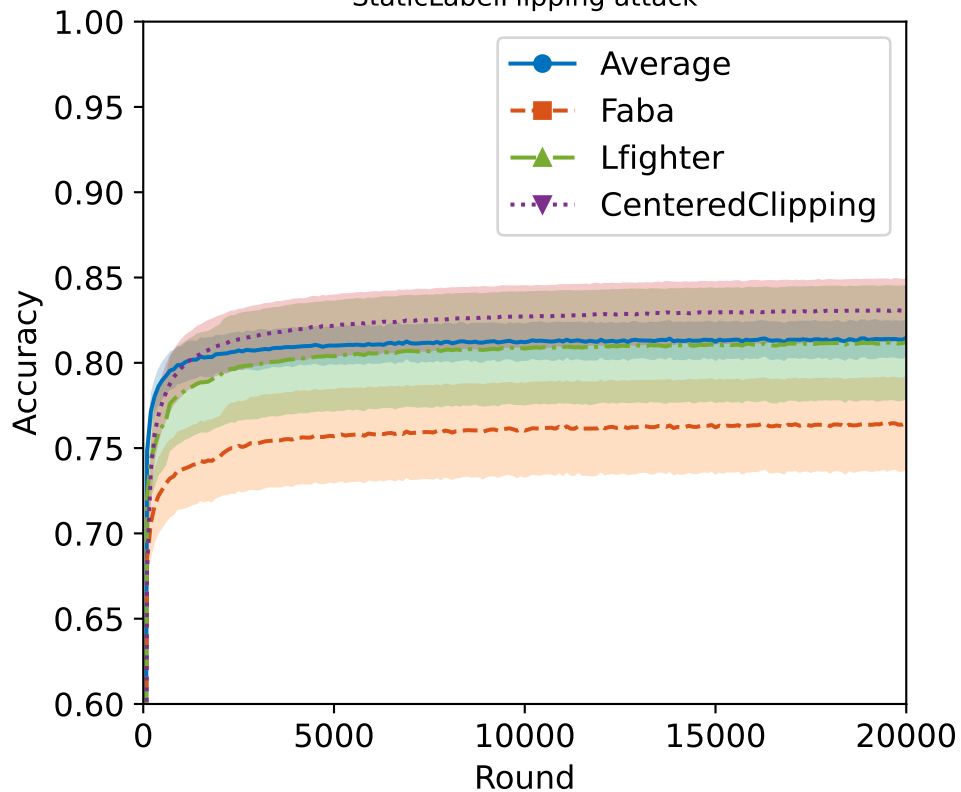
StaticLabelFlipping attack
