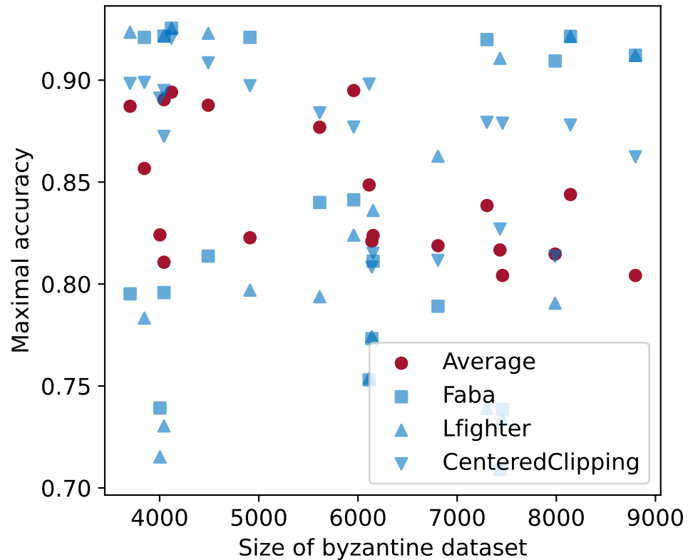
StaticLabelFlipping attack
