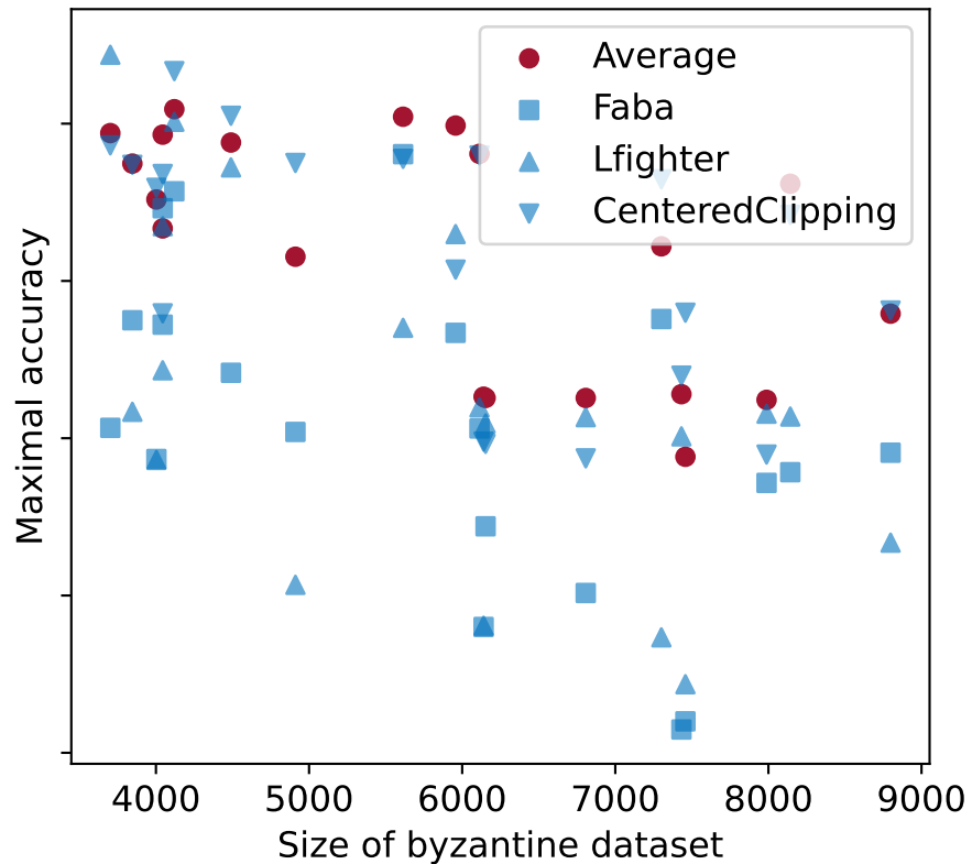
DynamicLabelFlipping attack
