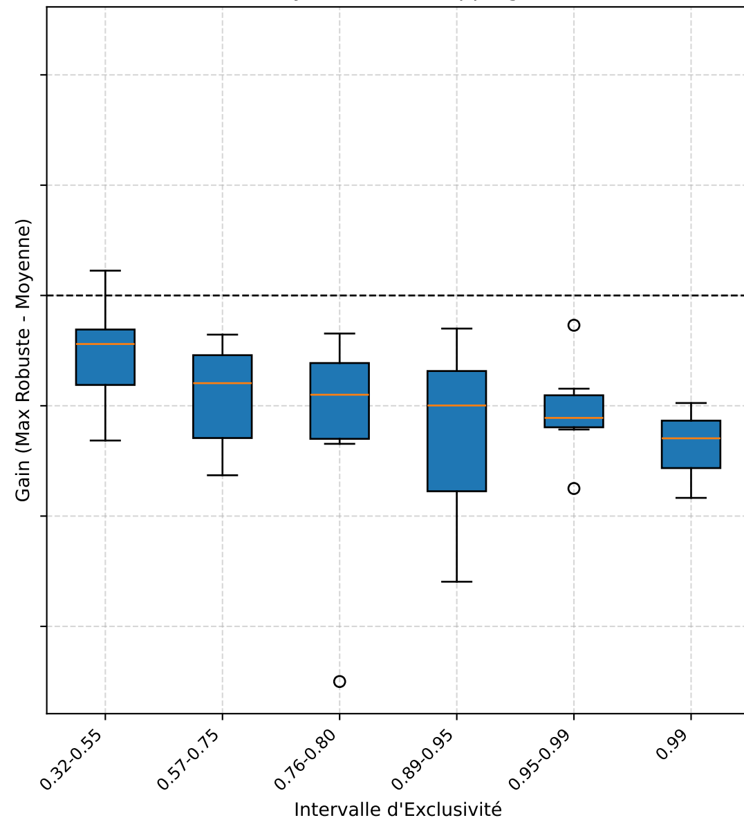
DynamicLabelFlipping
