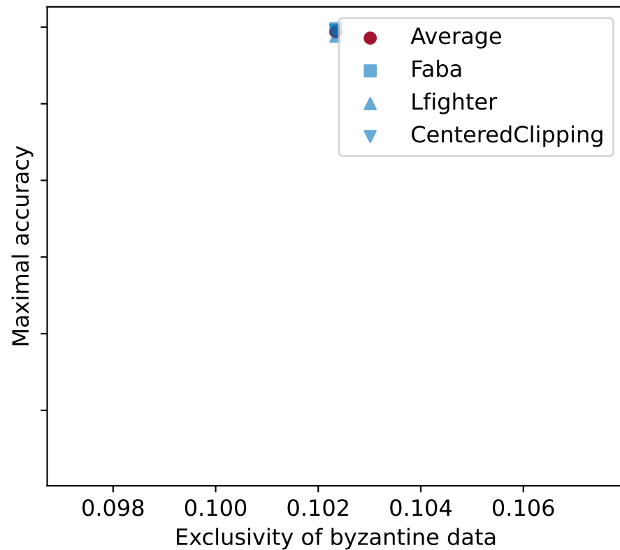
NoAttack attack
