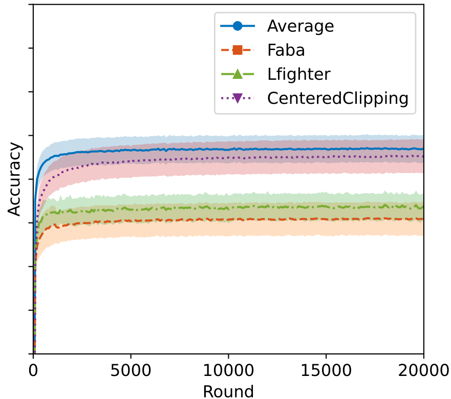
DynamicLabelFlipping attack
