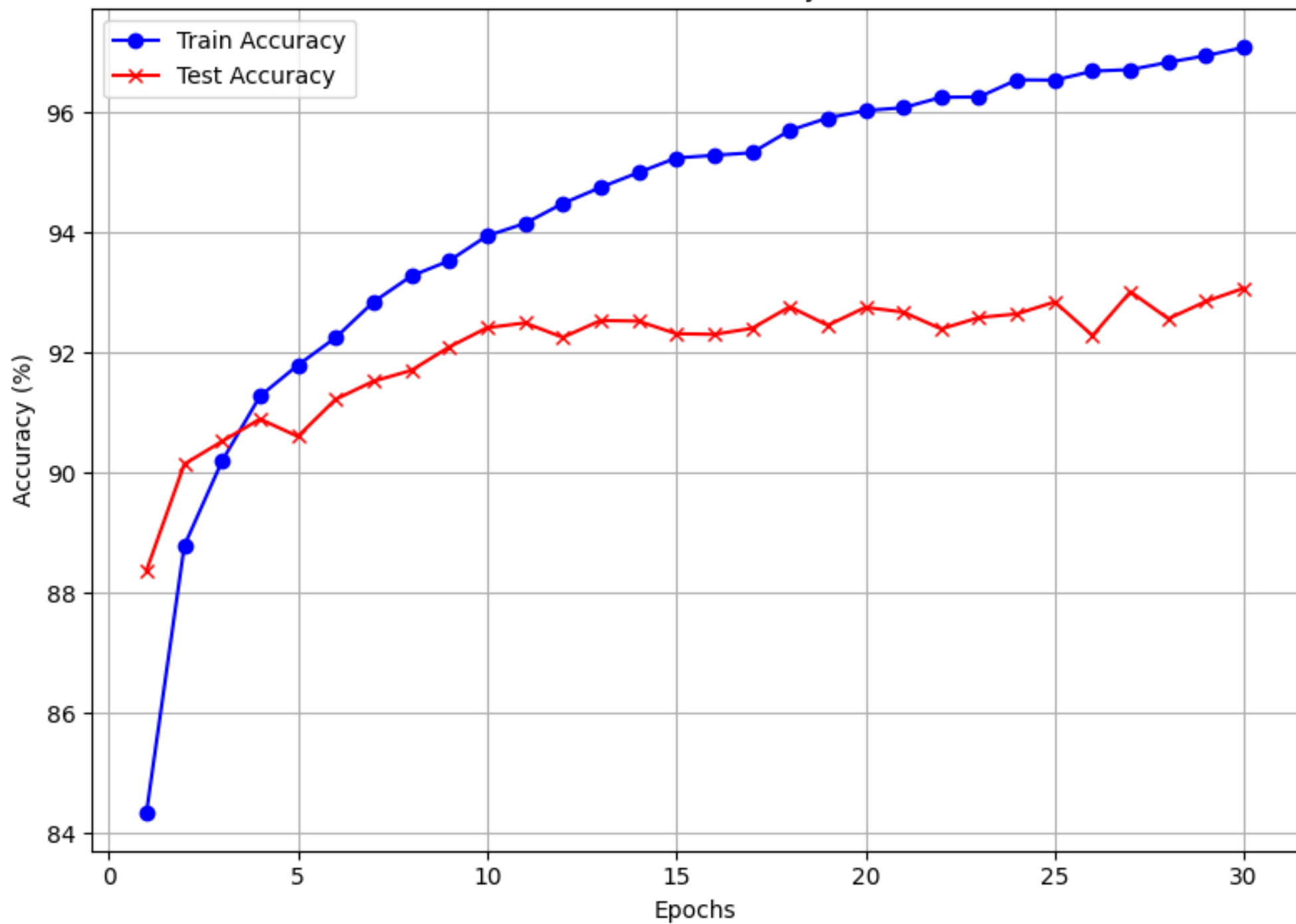
Fashion MNIST Accuracy Trend
