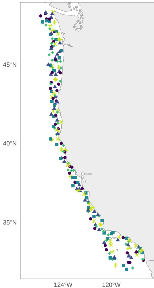
Dispersed, n = 200 random 5 fold
