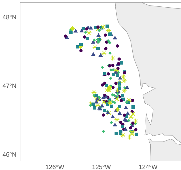
Clustered, n = 200 random 5 fold
