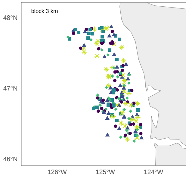
Clustered, n = 200 spatial block 5 fold
