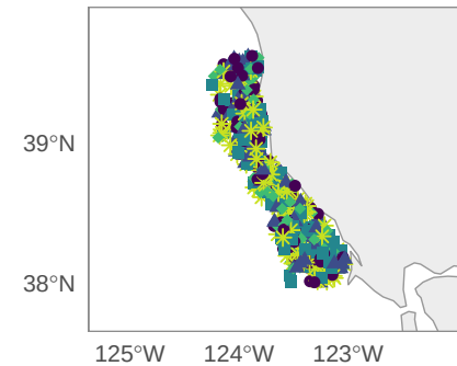
n = 500: random
