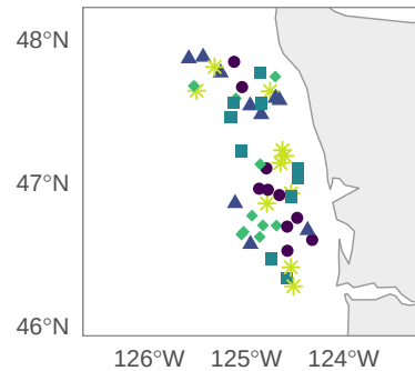
n = 50: random
