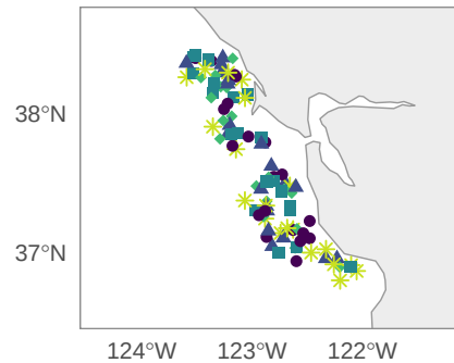
n = 100: random
