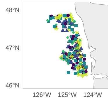
n = 200: random
