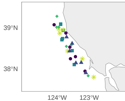
n = 30: random
