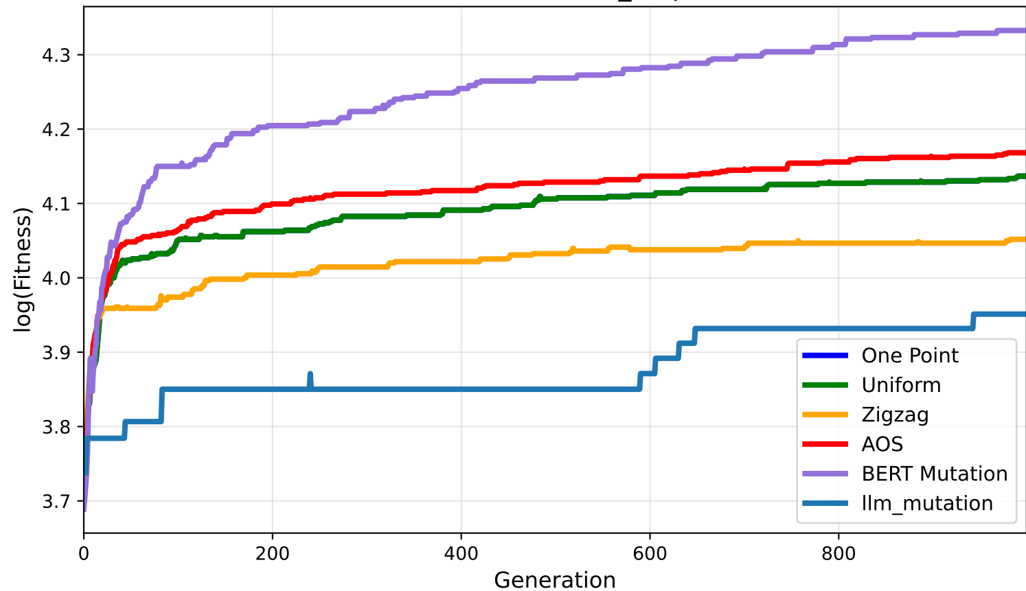
Artificial Ant (aux_map1)
