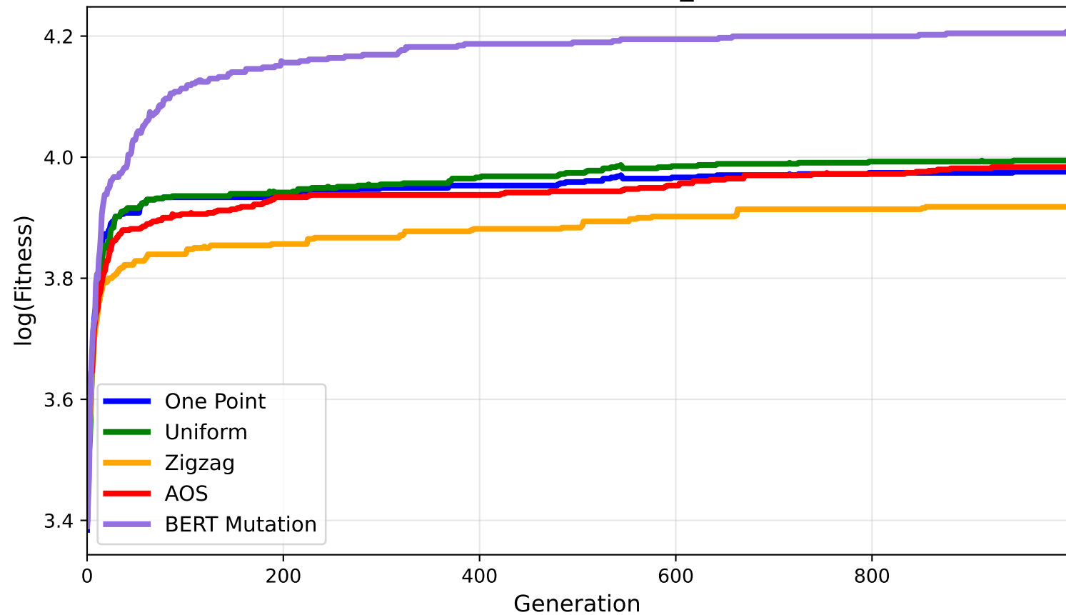
Artificial Ant (santafe_trail)
