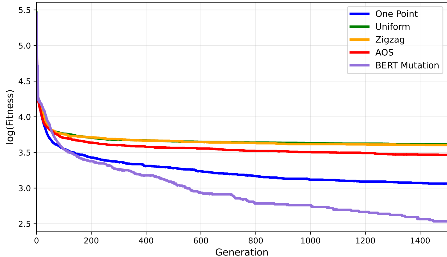
Graph Coloring (instances_games120)
