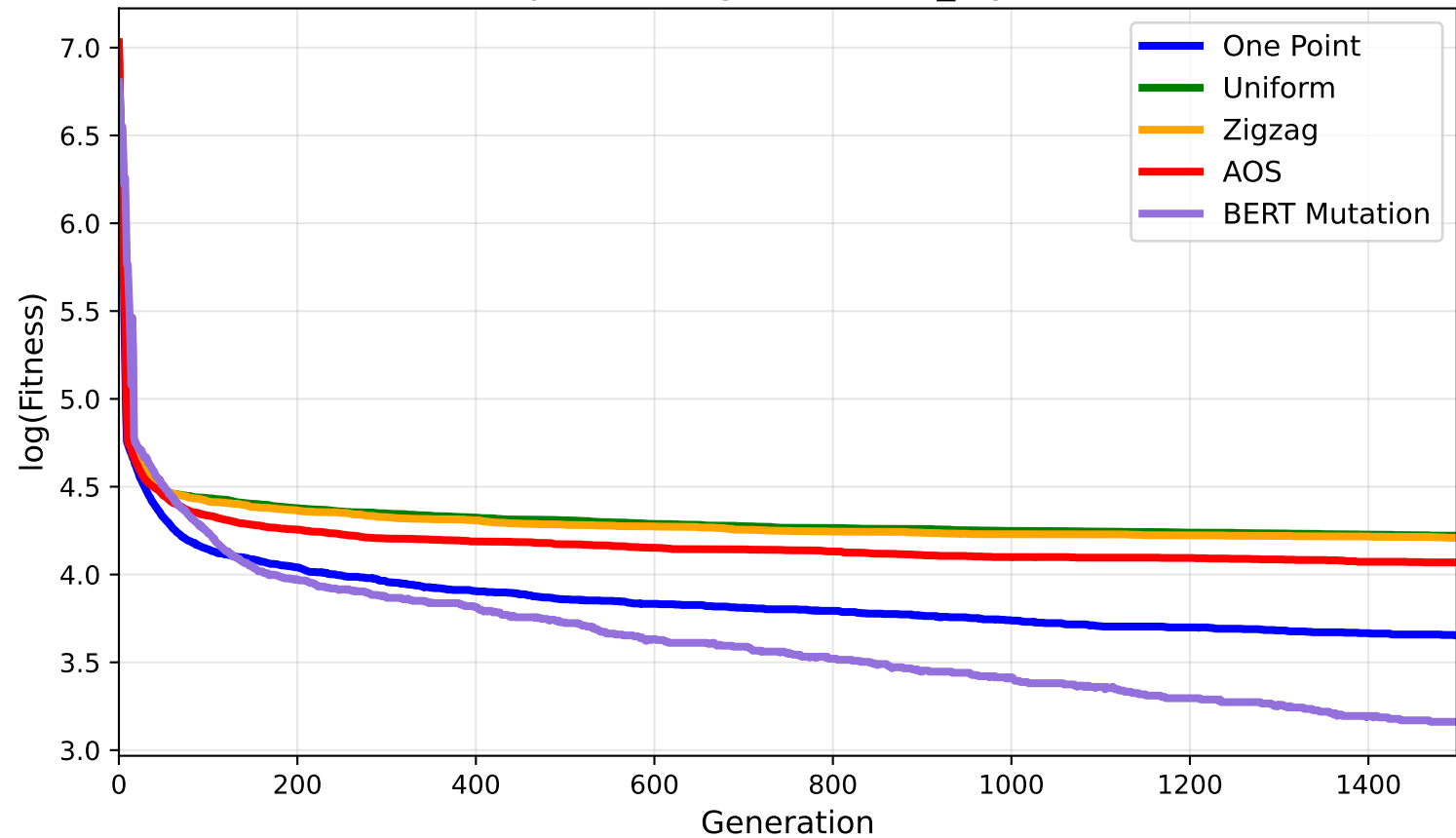
Graph Coloring (instances_myciel7)
