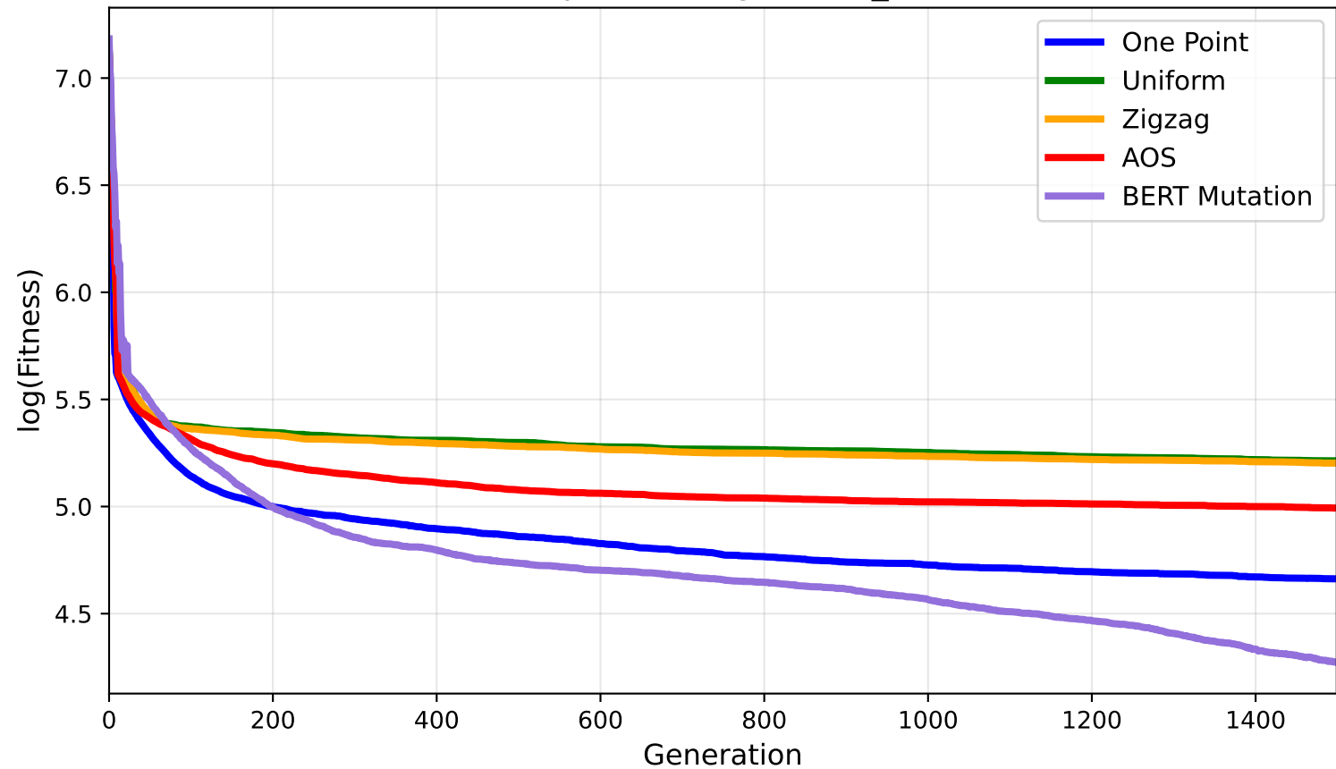
Graph Coloring (le450_5a)
