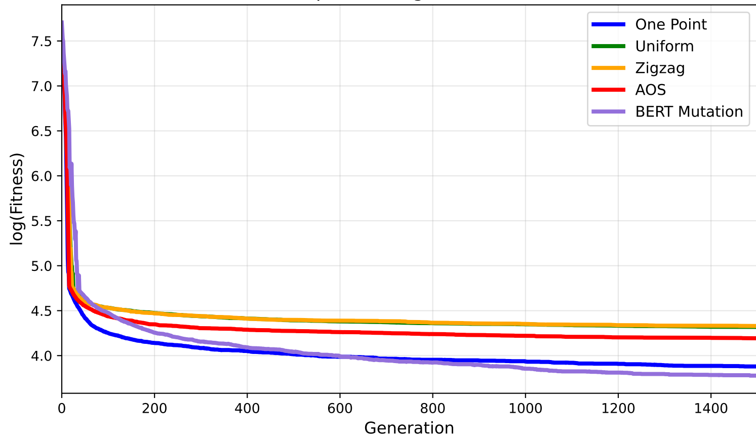
Graph Coloring (mulsol.i.2)
