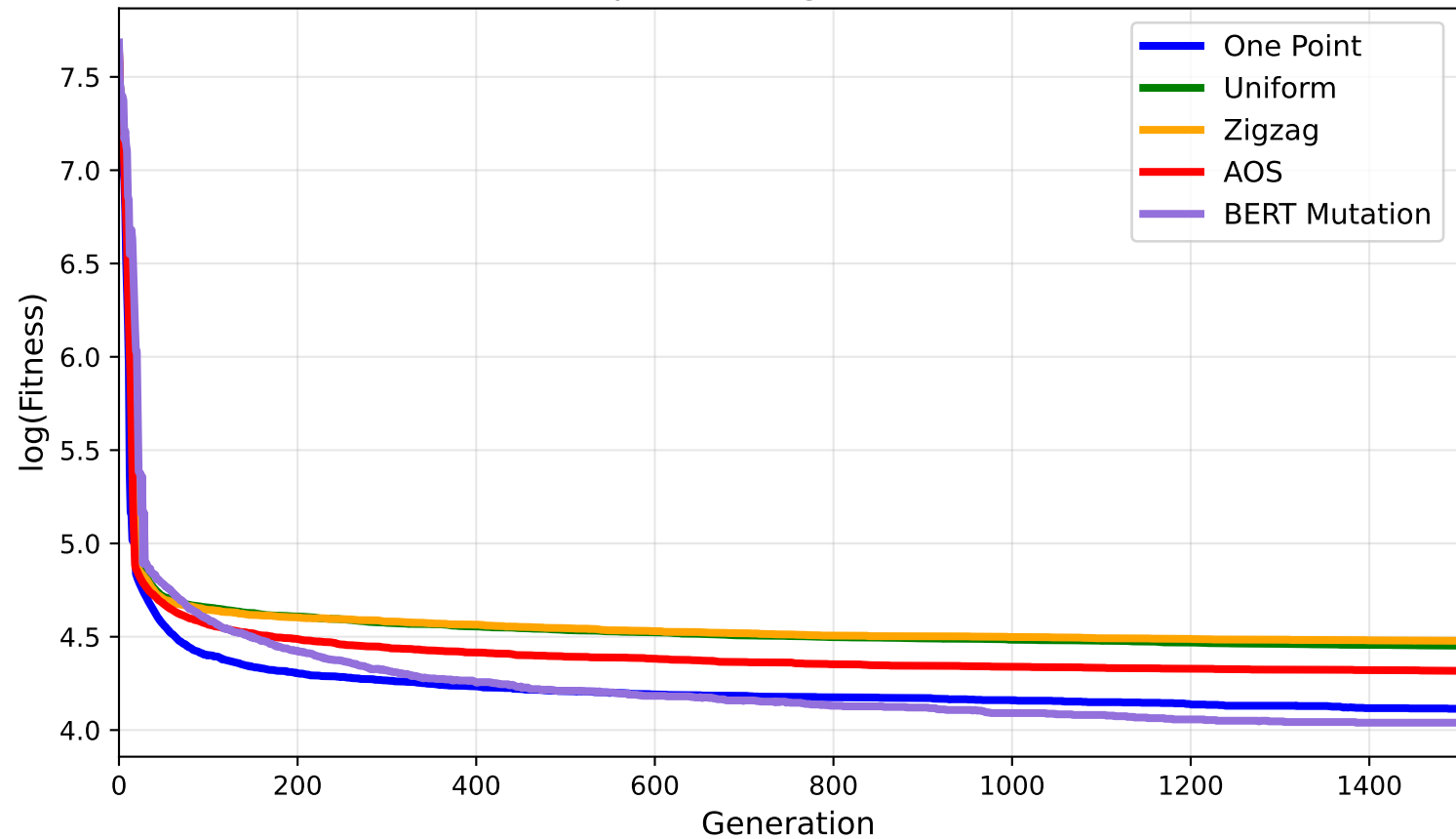
Graph Coloring (zeroin.i.1)
