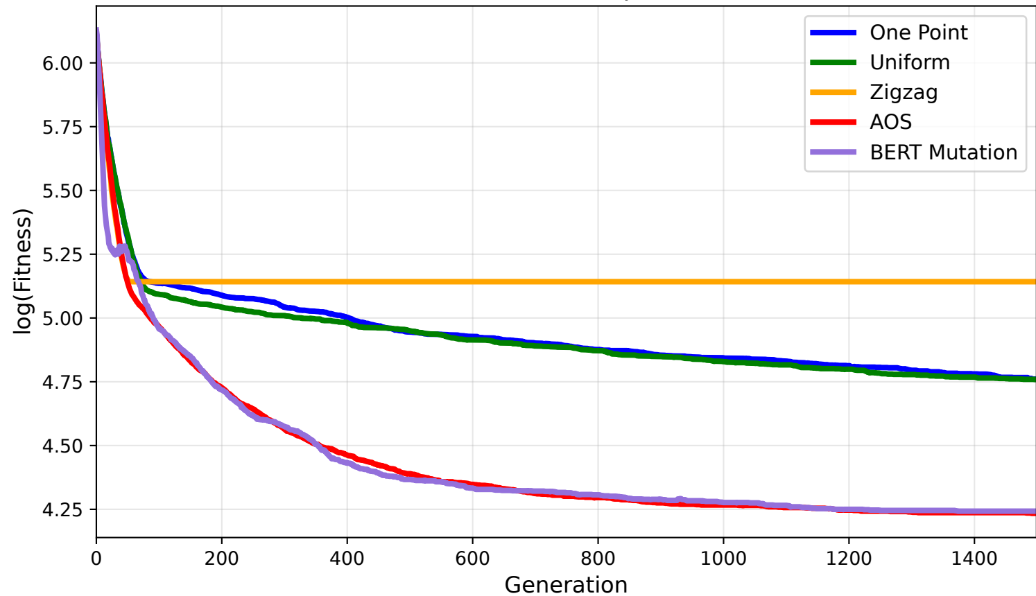
Set Cover (scp41)
