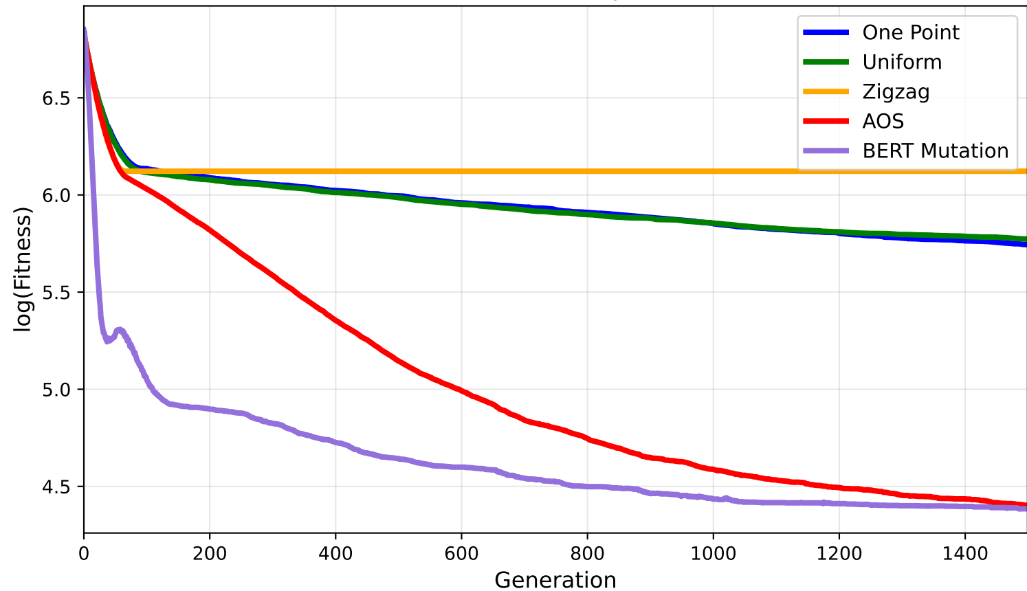
Set Cover (scp51)
