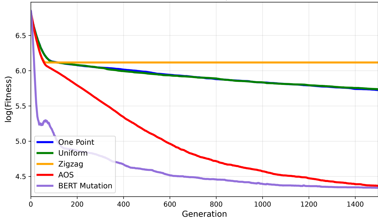
Set Cover (scp53)
