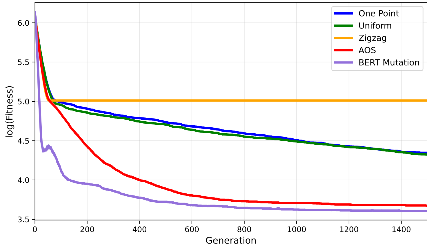
Set Cover (scp64)
