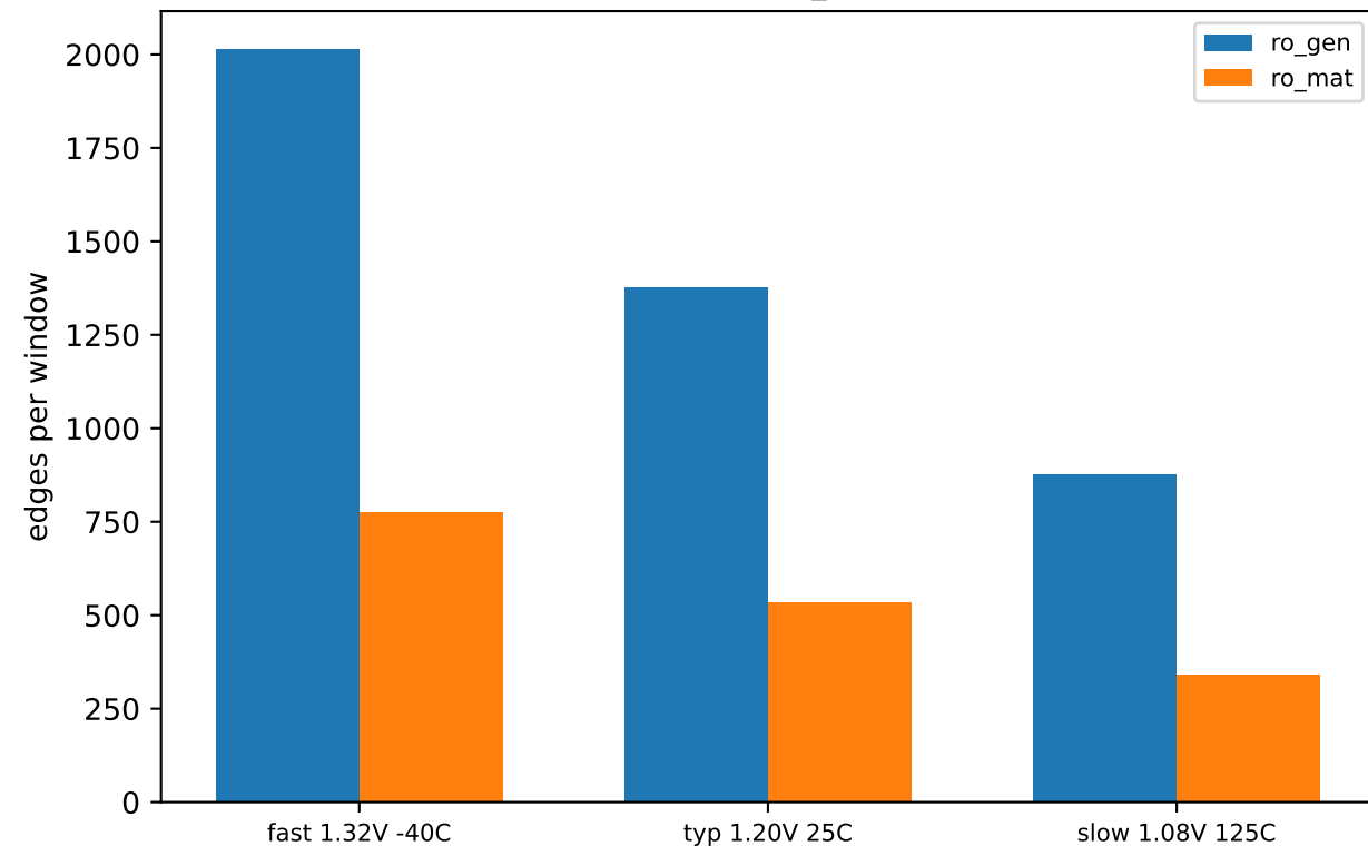
Canary counts (can_sel=3, win0)
