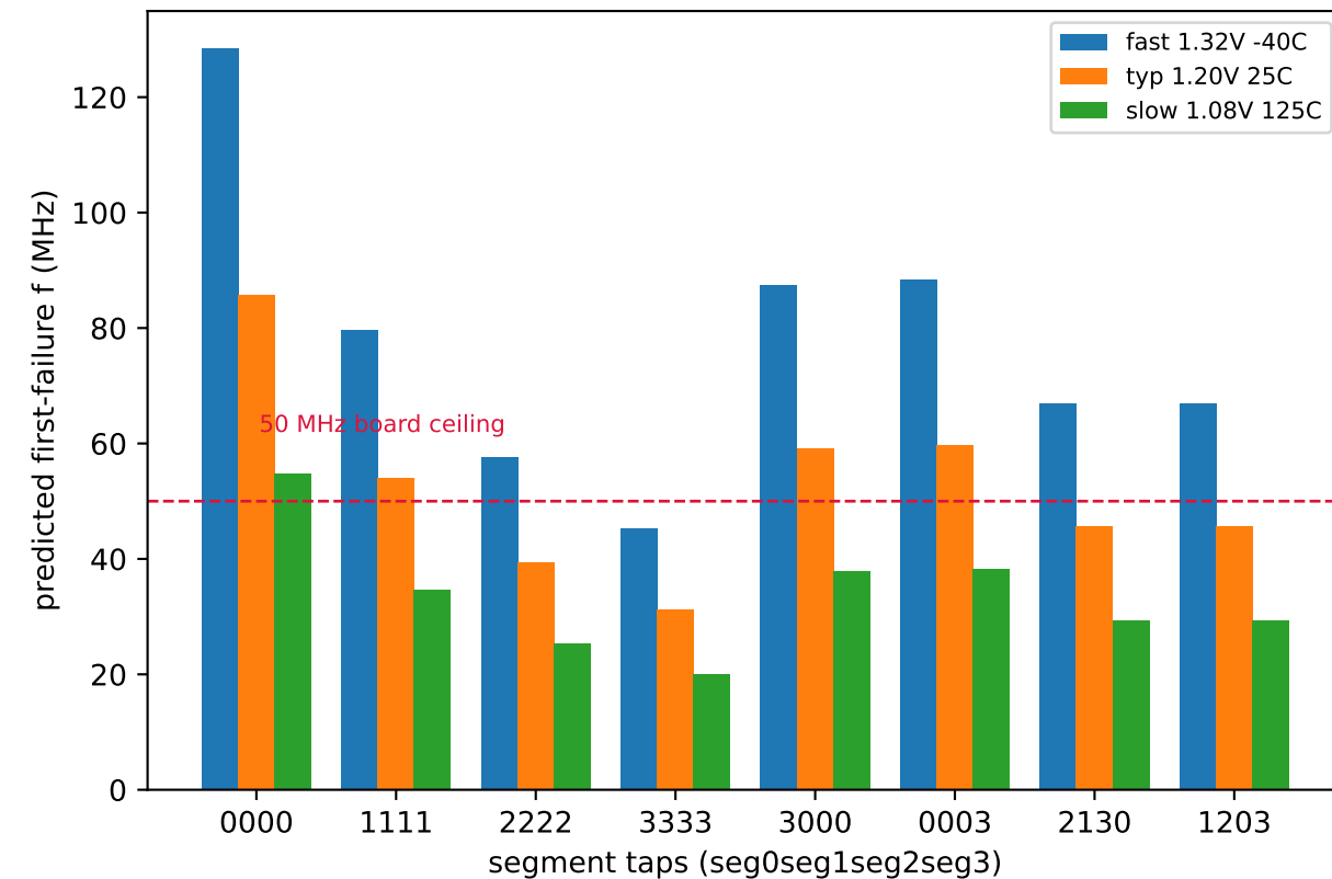
STA-predicted knee ladder (pattern = worst)
