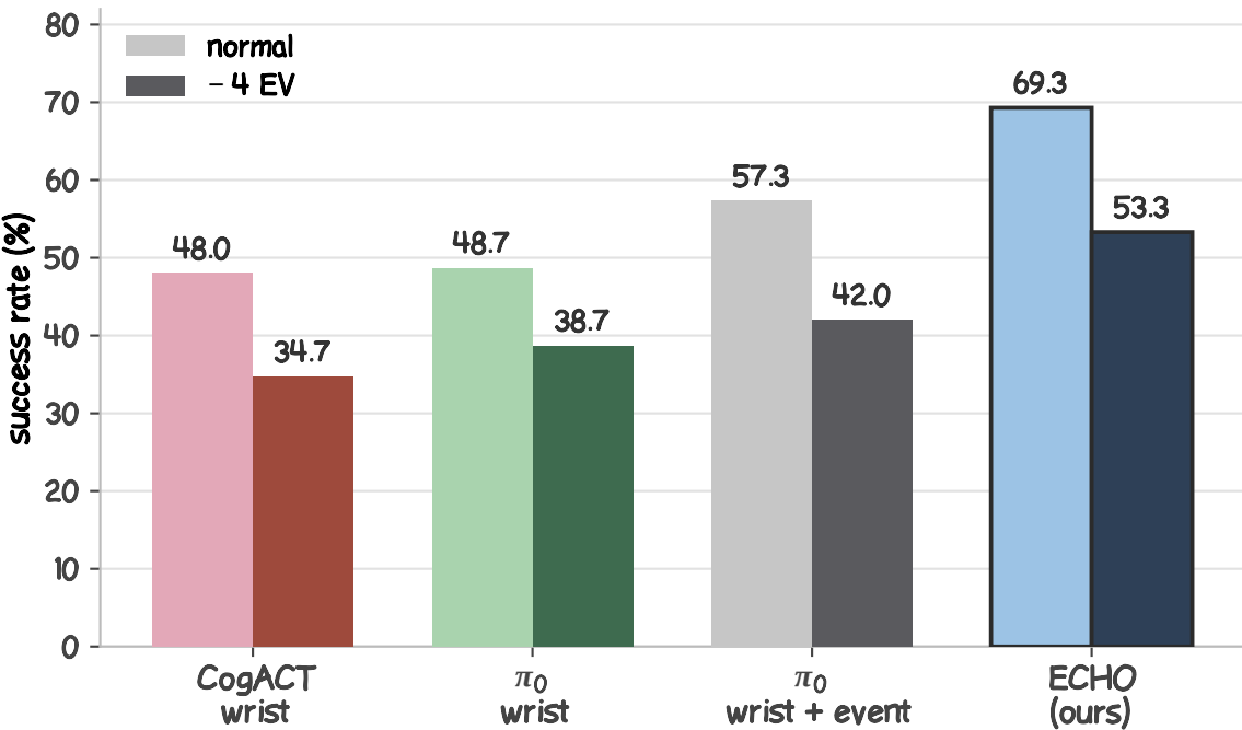
wrist-only success rates (simulation)
