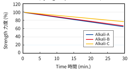
Dependency of Steaming Time 蒸處時間依存性 (PD/PS) (Saturated steam at 102°C)
