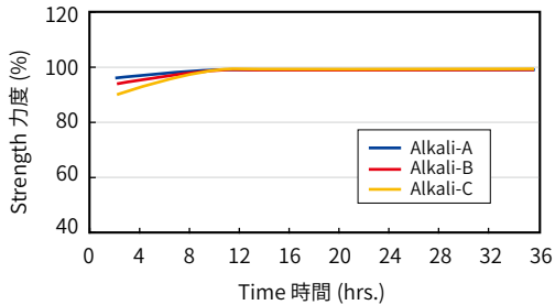
Stability of Padding Liquor 染液安定性 (CPB) (Dyeing temperature at 25°C)
