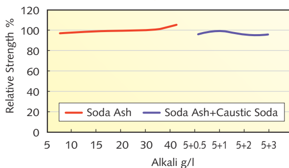
鹼依存性 Dependency on Alkali
