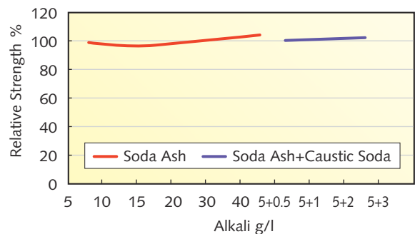
鹼依存性 Dependency on Alkali
