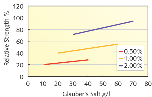
芒硝依存性 Dependency on Glauber's Salt
