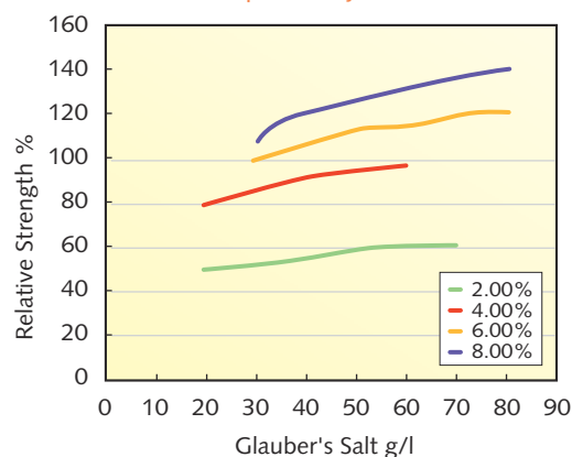
芒硝依存性 Dependency on Glauber's Salt
