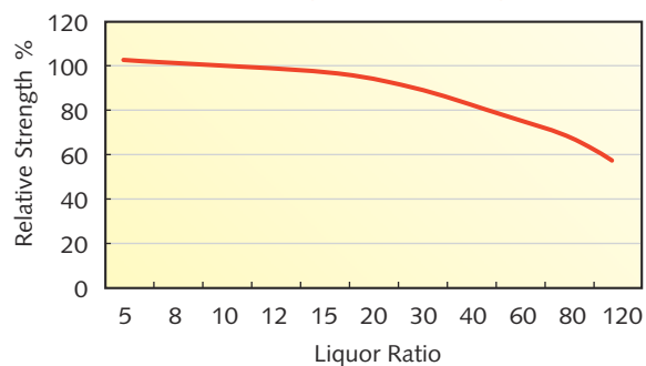
浴比依存性 Dependency on Liquor Ratio
