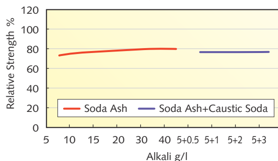
鹼依存性 Dependency on Alkali
