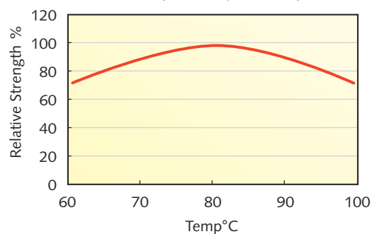
溫度依存性 Dependency on Temperature
