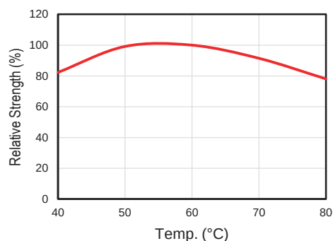
溫度依存性 Dependency on Temperature
