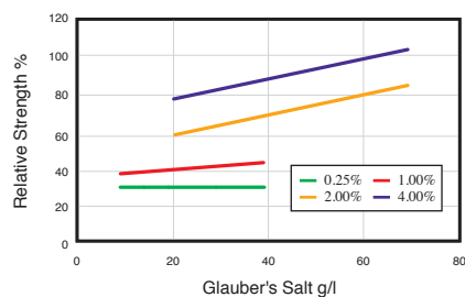
芒硝依存性 Dependency on Glauber's salt
