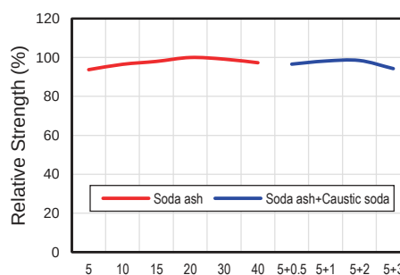
鹼依存性 Dependency on Alkali
