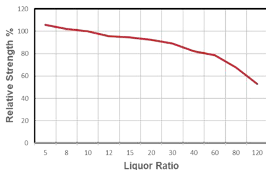
浴比依存性 Dependency on Liquor ratio
