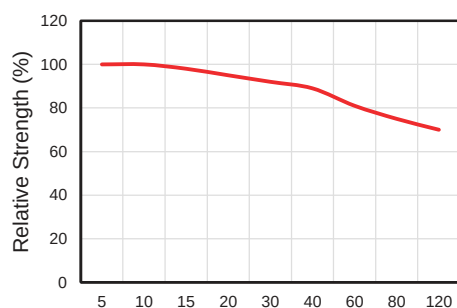
浴比依存性 Dependency on Liquor ratio
