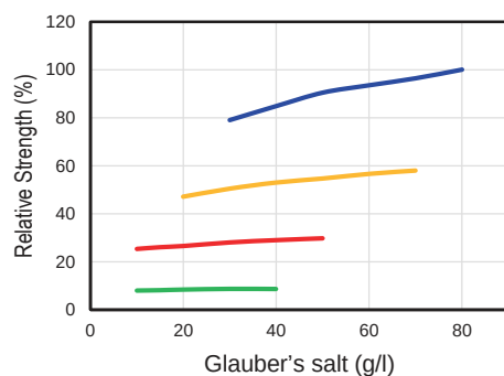
芒硝依存性 Dependency on Glauber's salt
