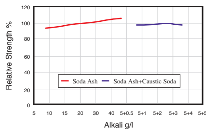
鹼依存性 Dependency on alkali
