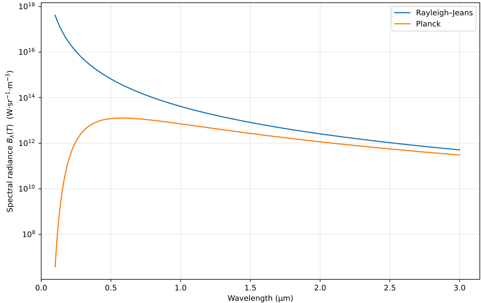
Blackbody Radiation Laws at T = 5000\text{ K}
