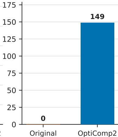
Automated tests
