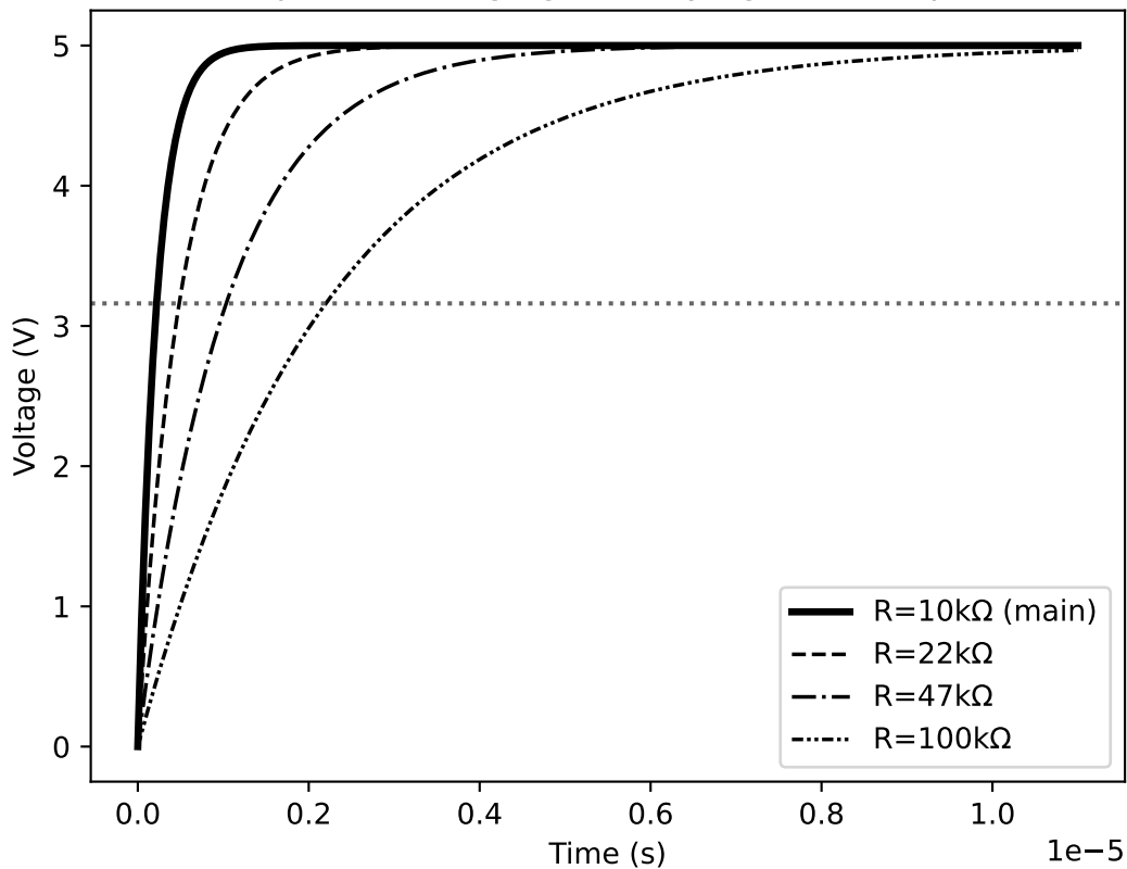
Capacitor charging for varying R (C=22 pF)
