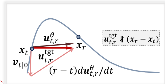
(e) practical learning of CTSC
