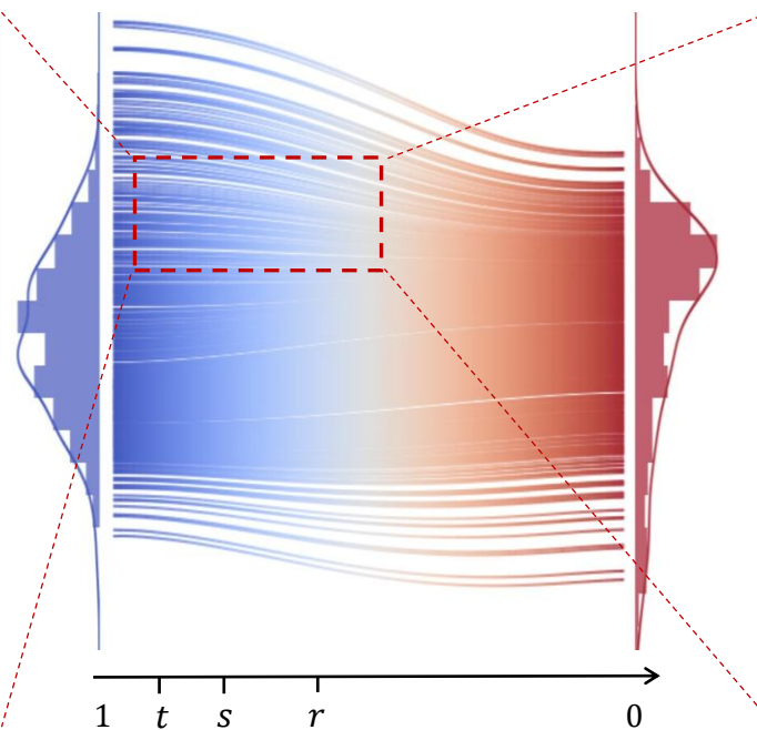
(a) marginal velocity field
