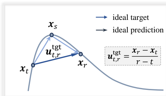
(b) ideal learning of DTSC
