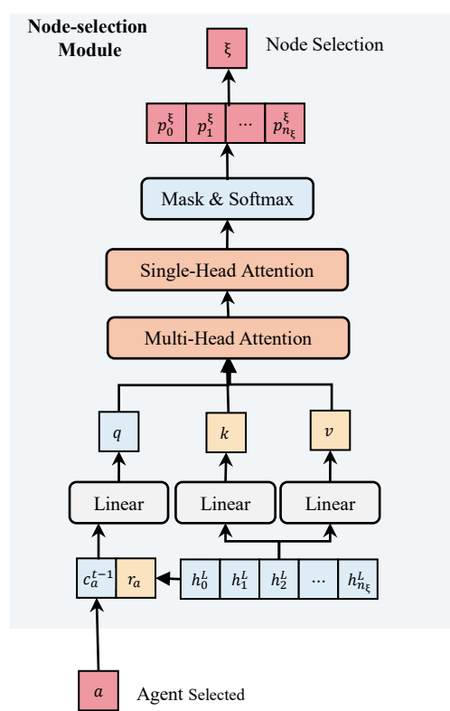
Collaborative Decoder
