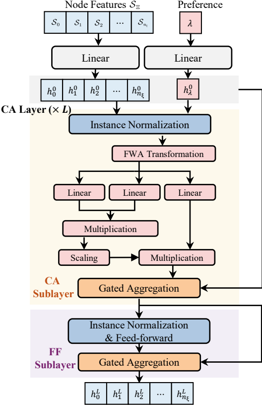
Conditional Encoder
