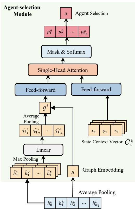
Collaborative Decoder
