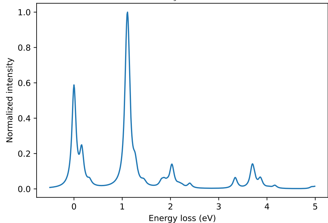
RIXS at E_{L_3} = 853.31 eV
