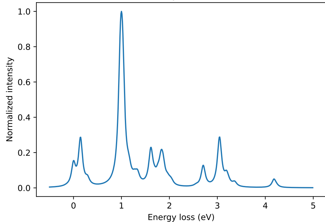
RIXS at E_{L_3} = 853.25 eV
