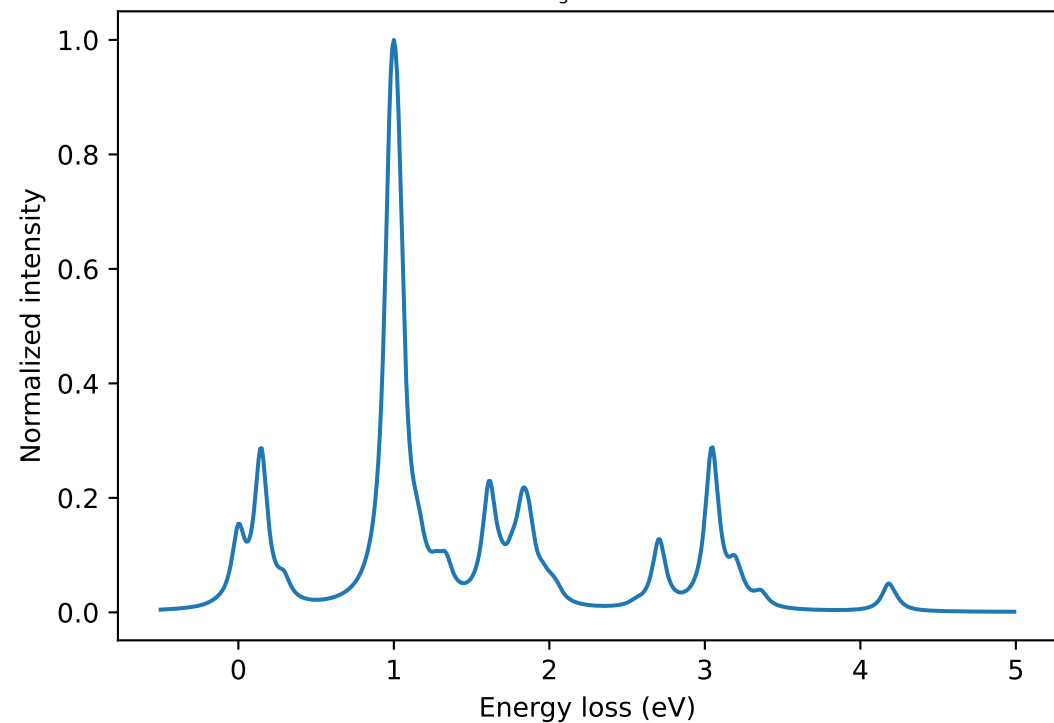
RIXS at E_{L_3} = 853.25 eV
