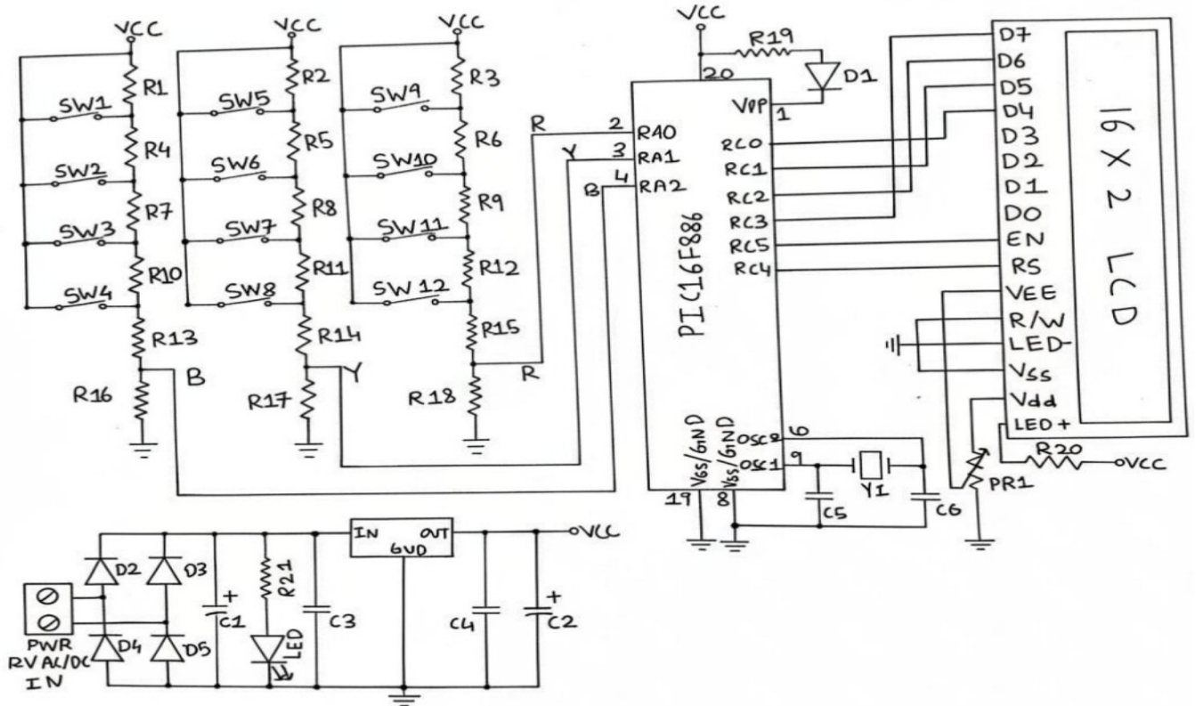
Figure 1: Original Hand-Drawn Circuit Diagram
