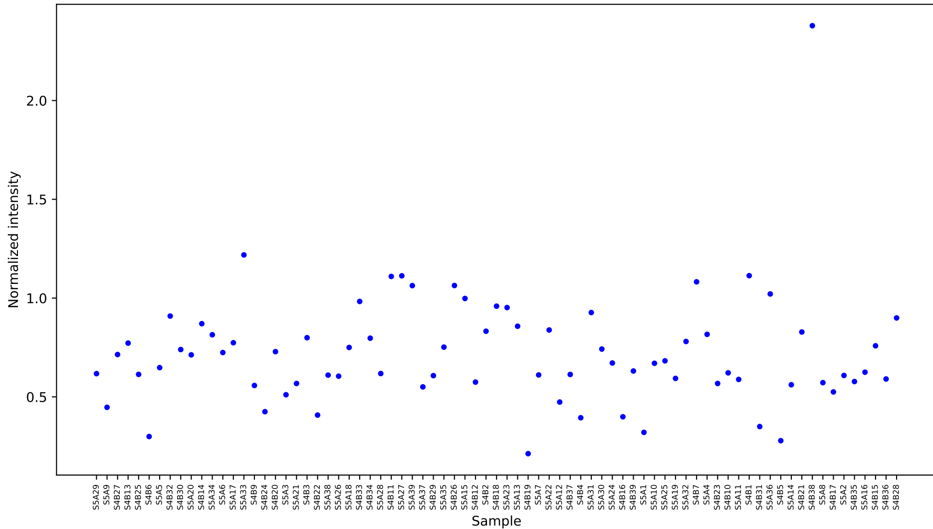
[7427] D-(+) trehalose [24.752] Results
