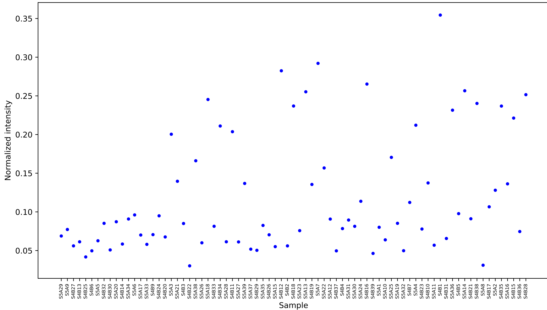
[135] 4-hydroxybenzoic acid [14.505] Results
