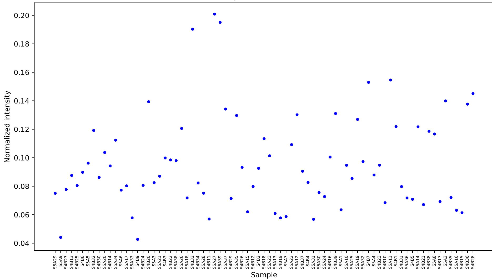
[338] salicylic acid [13.075] Results
