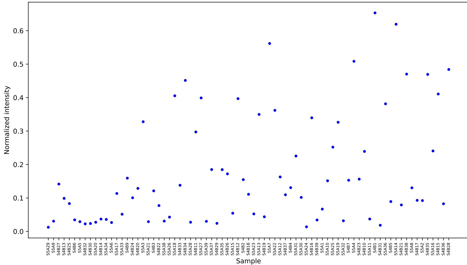
[835] dehydroascorbic acid 1 [16.863] Results
