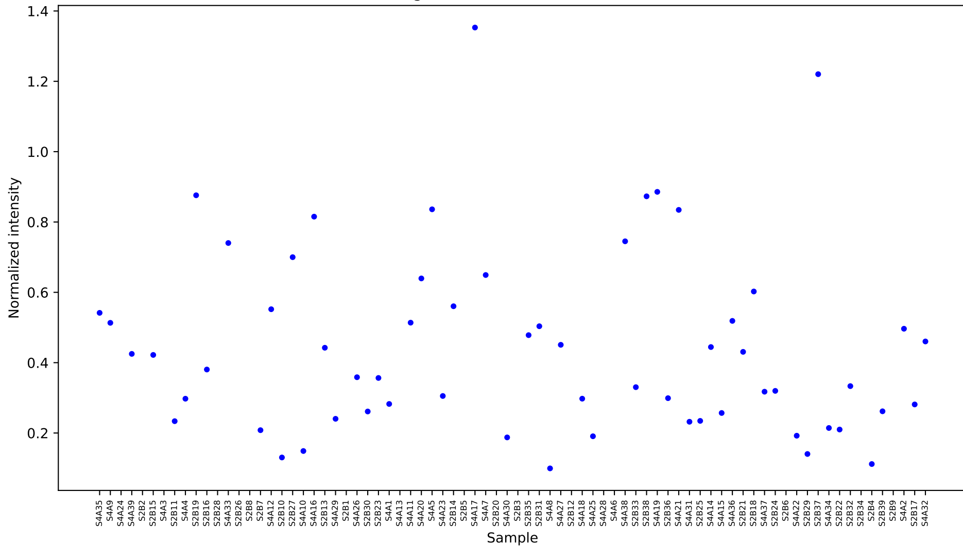
[128869] galactonic acid 2 [18.504] Results
