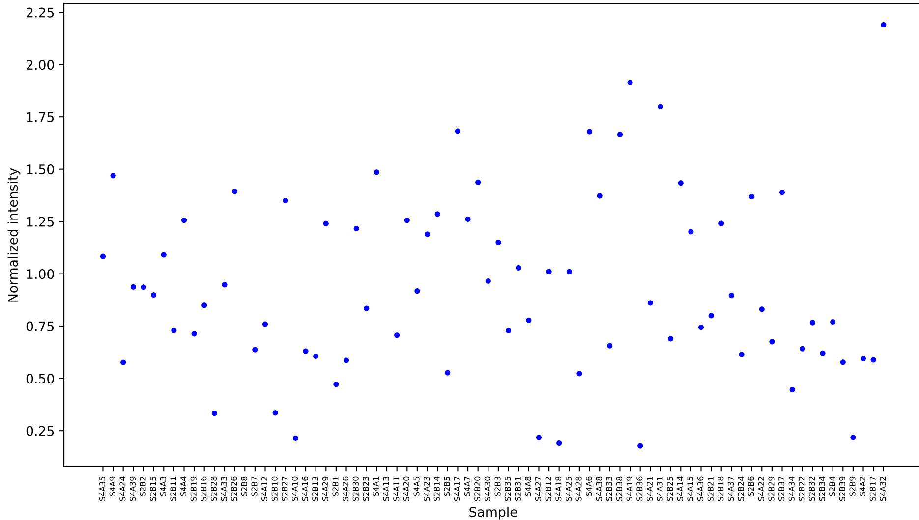
[6255] maltose 1 [24.702] Results
