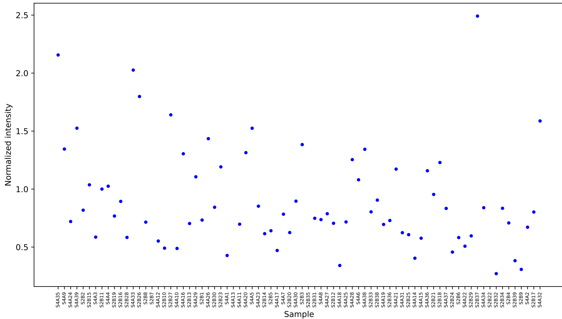
[6251] D-mannitol [17.81] Results
