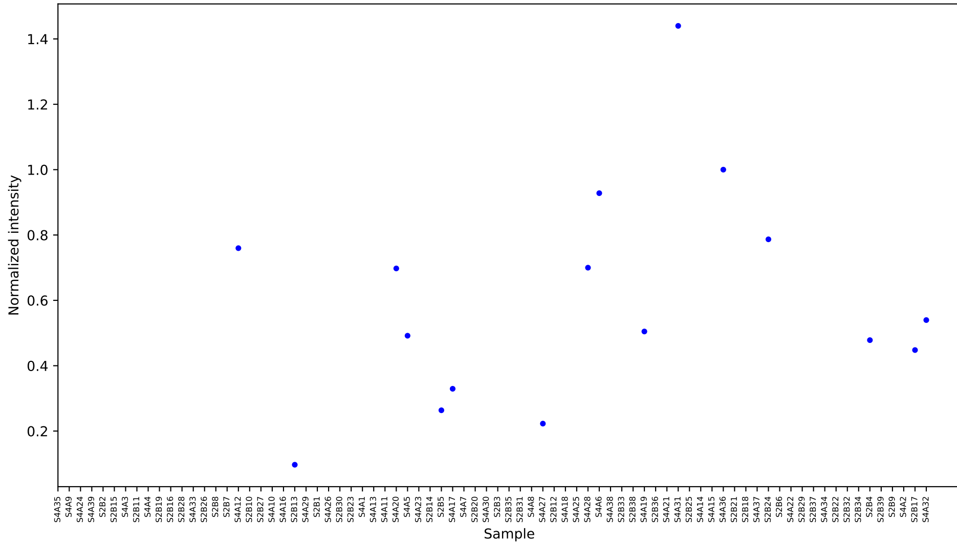
[750] glycine [10.456] Results
