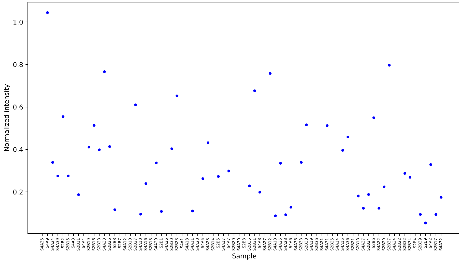
[51] alpha ketoglutaric acid [13.859] Results
