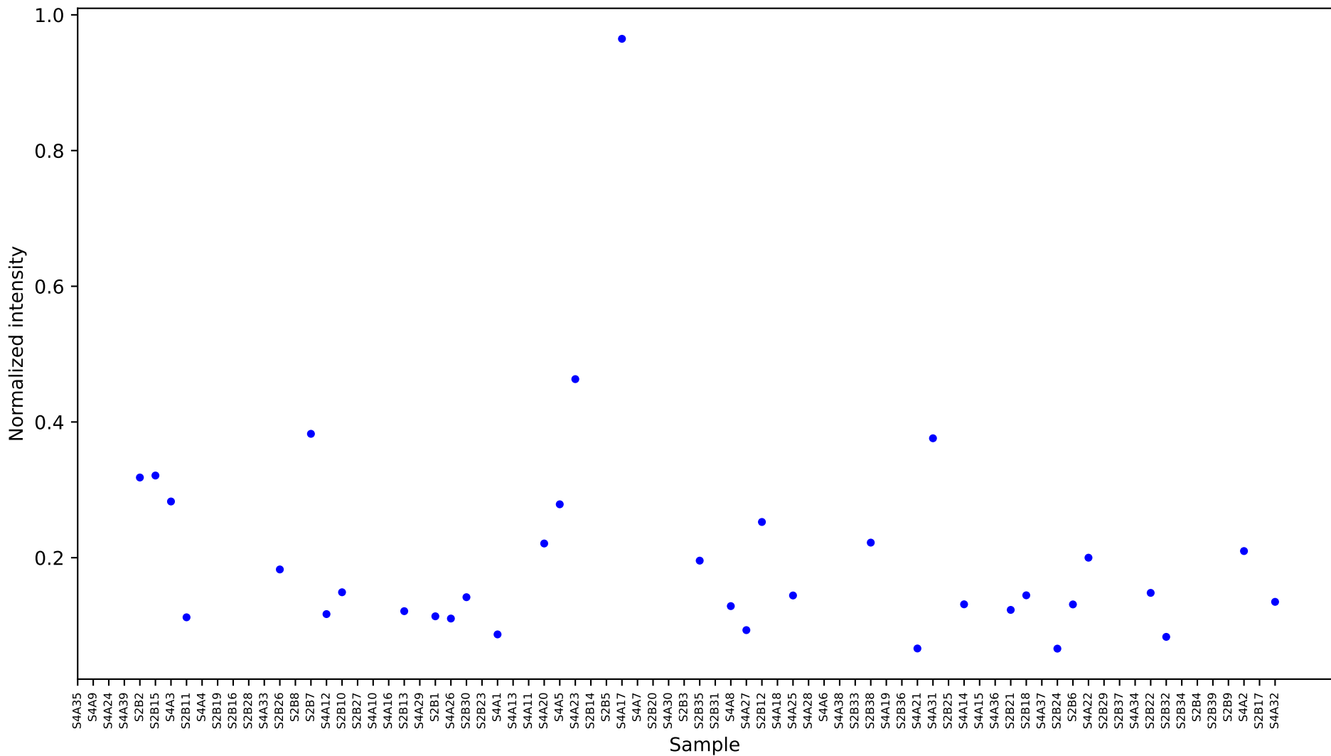
[12647] L-homoserine 2 [12.359] Results
