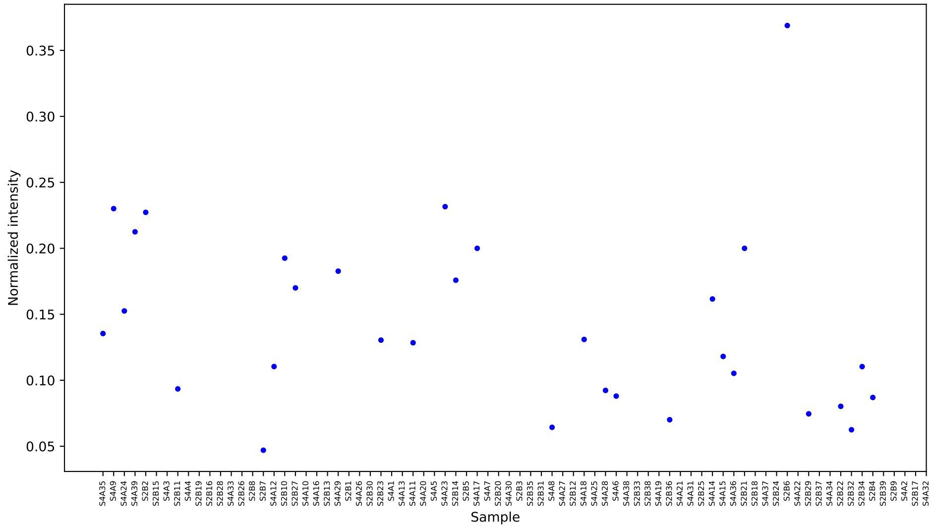
[145742] L-proline 2 [10.321] Results
