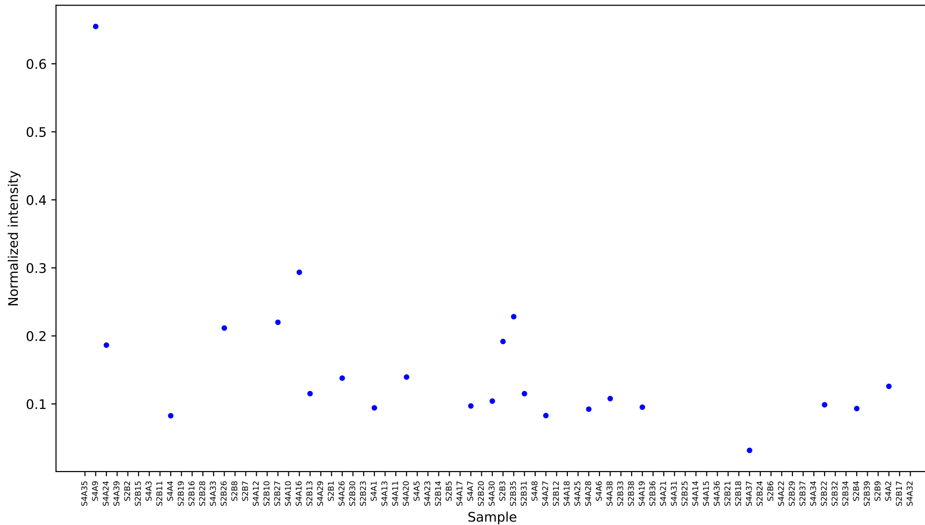
[6287] L-valine 2 [9.151] Results
