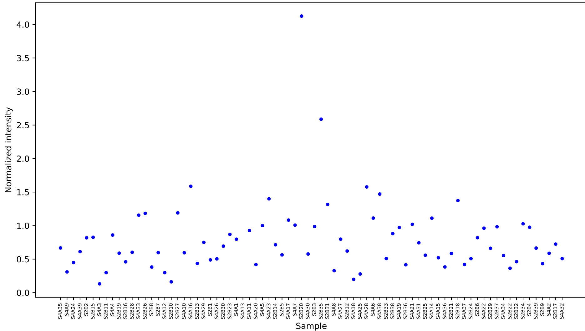
[5281] stearic acid [20.675] Results
