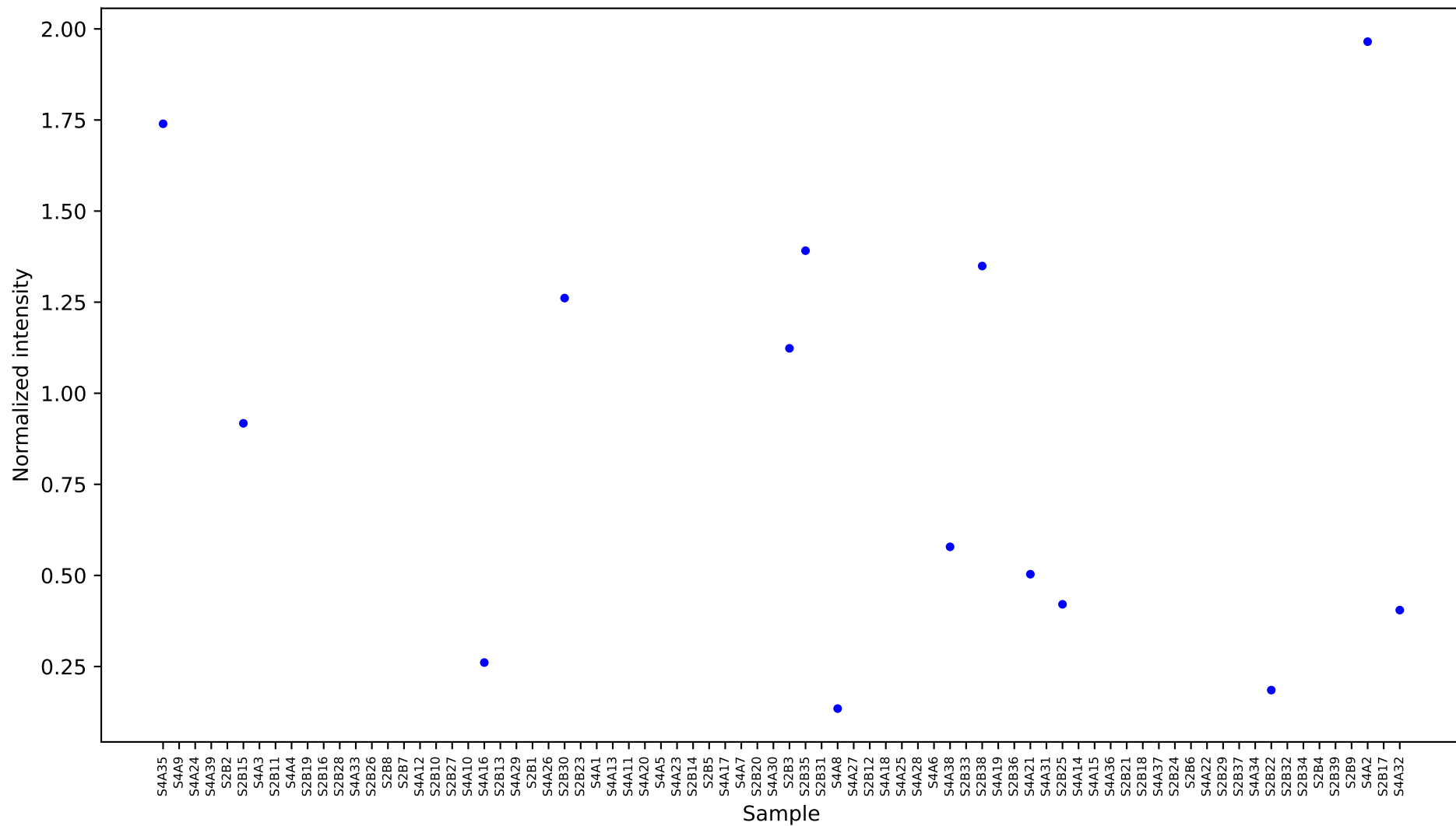
[971] oxalic acid [7.883] Results
