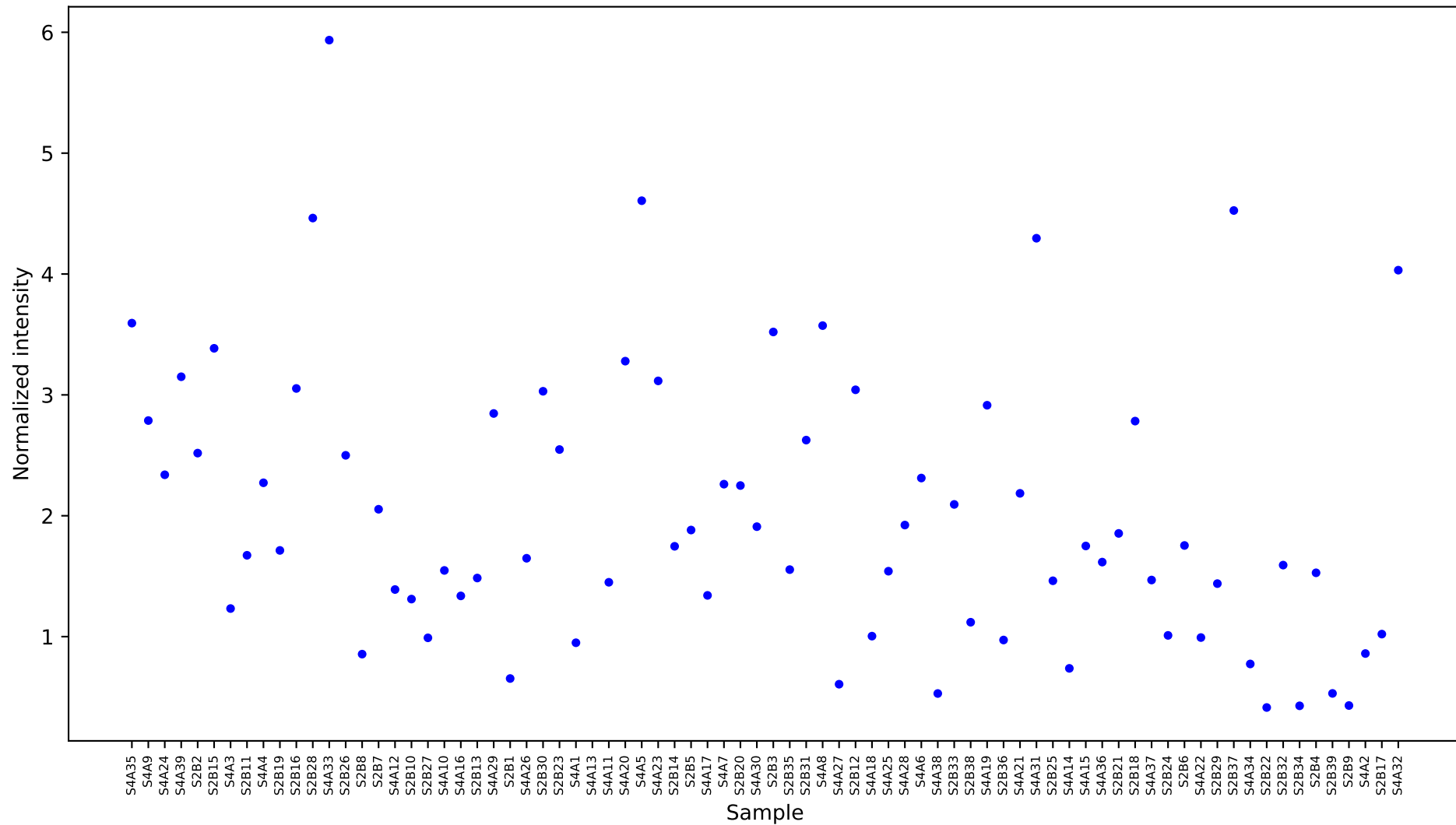
[92824] D-malic acid [12.794] Results
