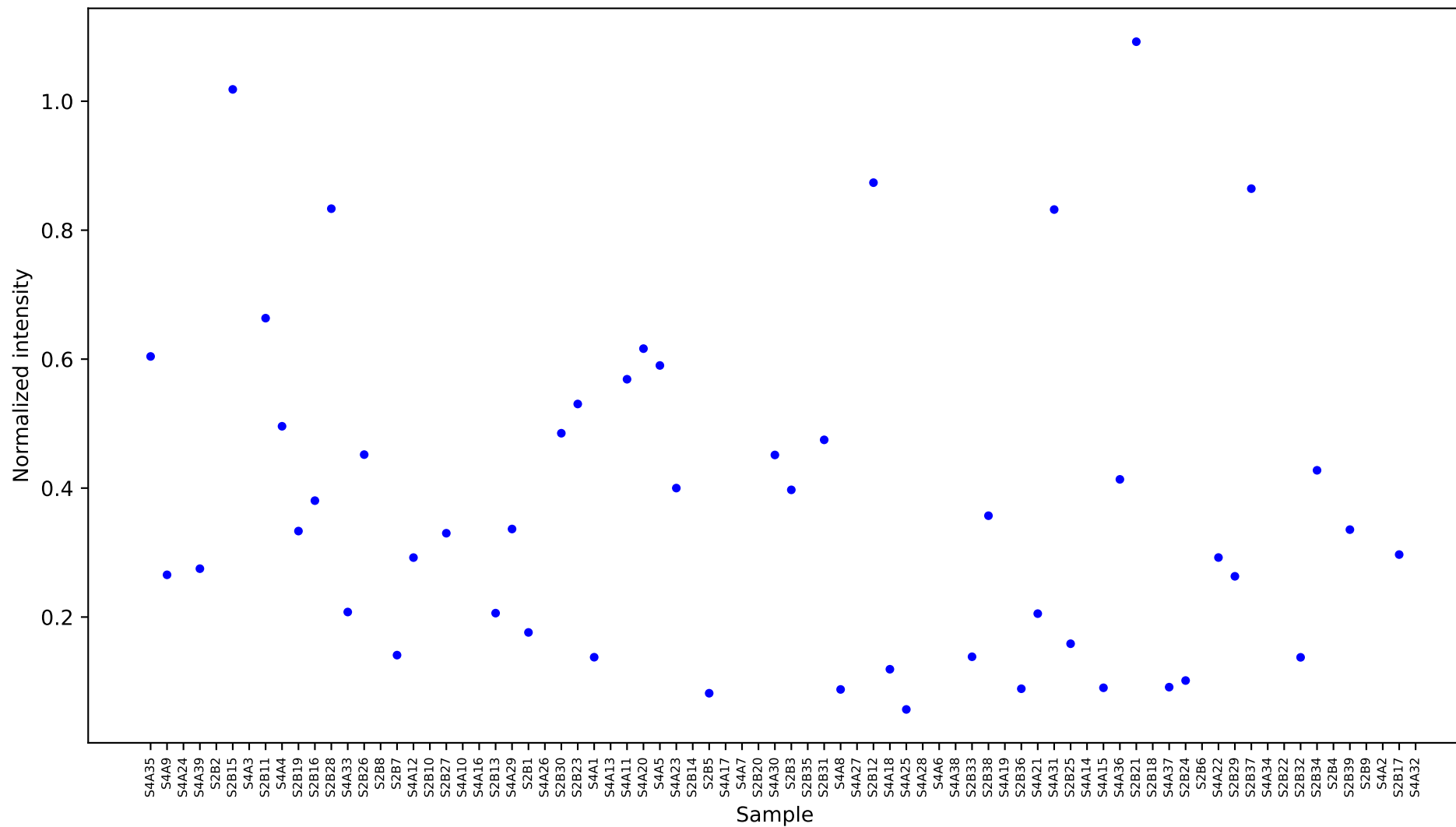
[5951] L-serine 2 [11.174] Results
