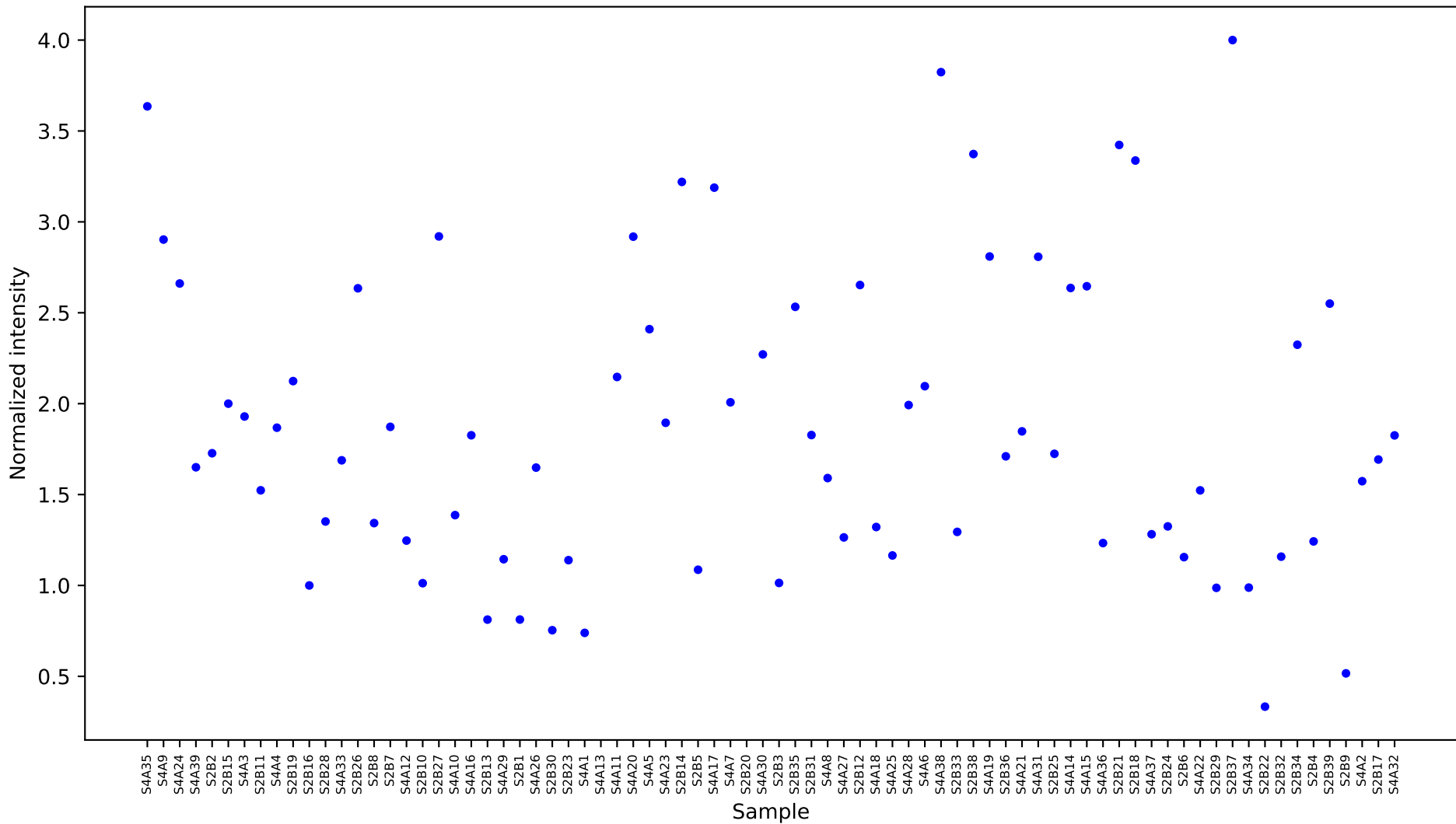
[892] myo-inositol [19.354] Results
