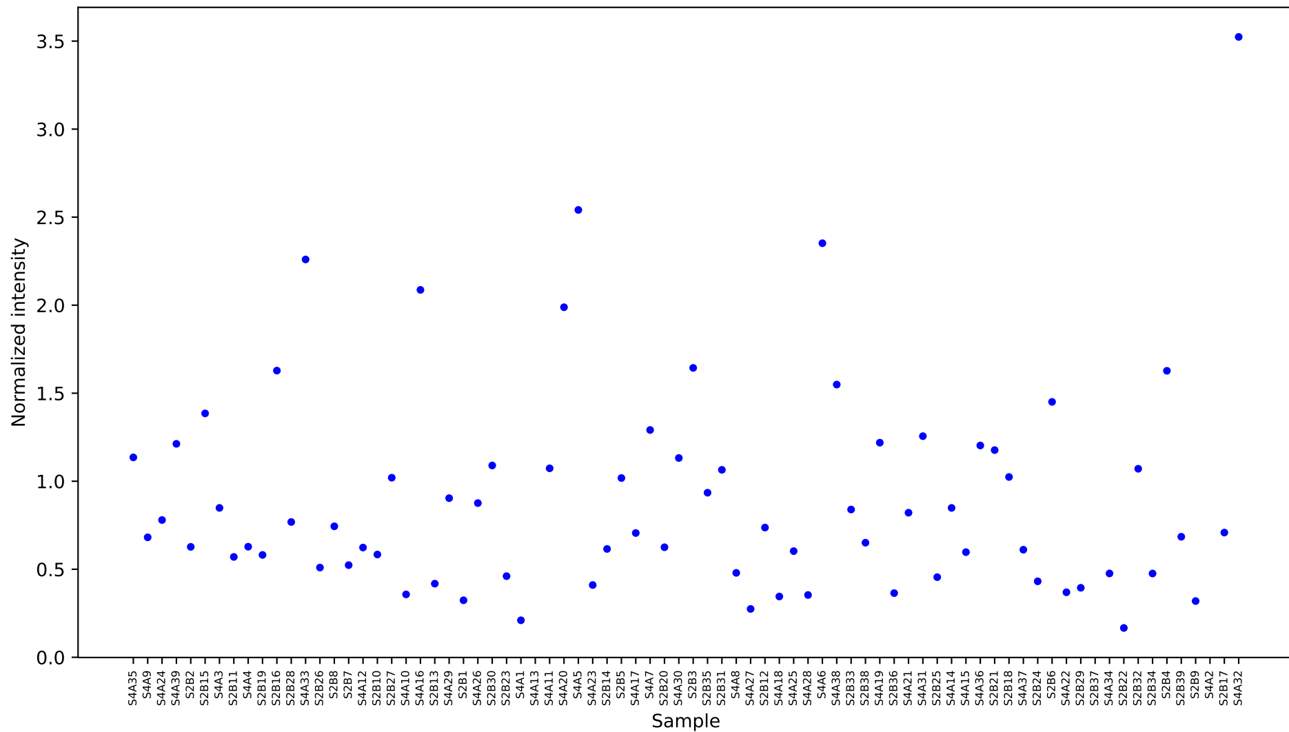
[5984] fructose 2 [17.288] Results
