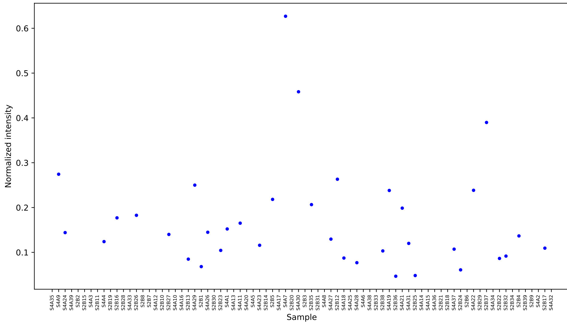
[5951] L-serine 1 [9.706] Results
