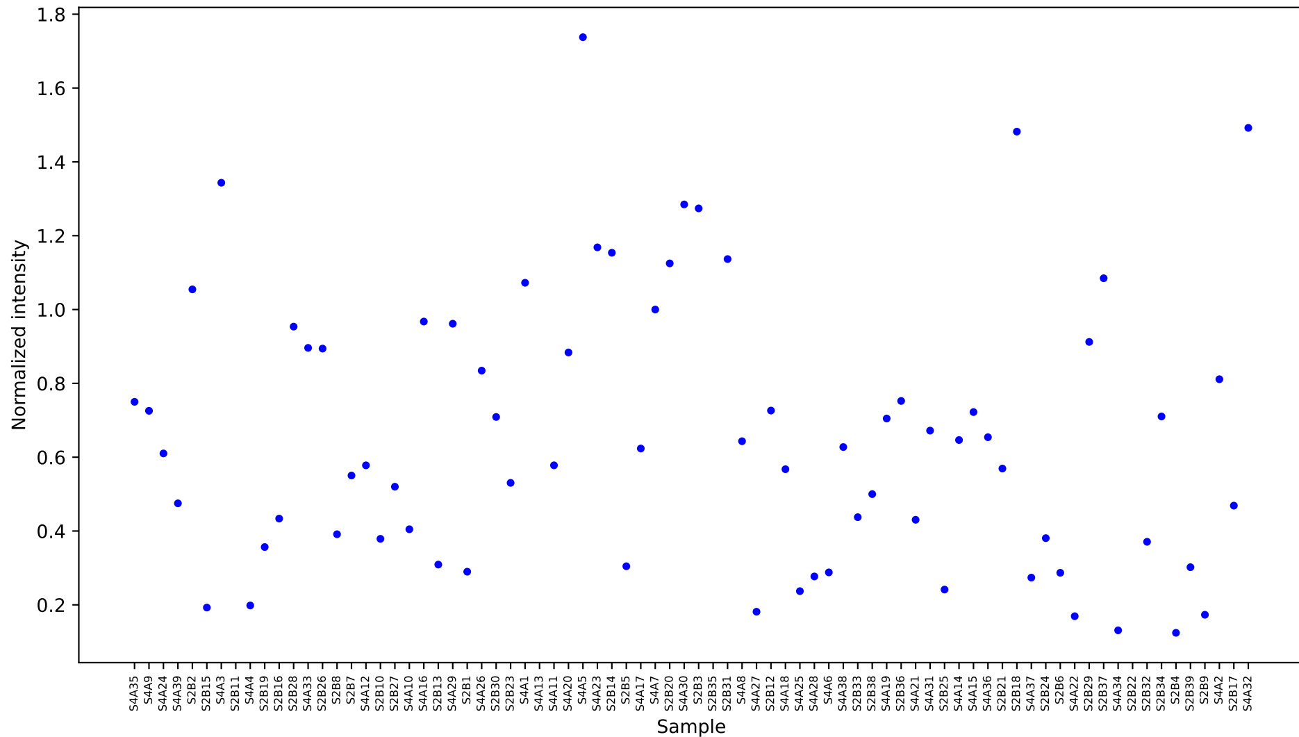
[60961] adenosine [23.825] Results
