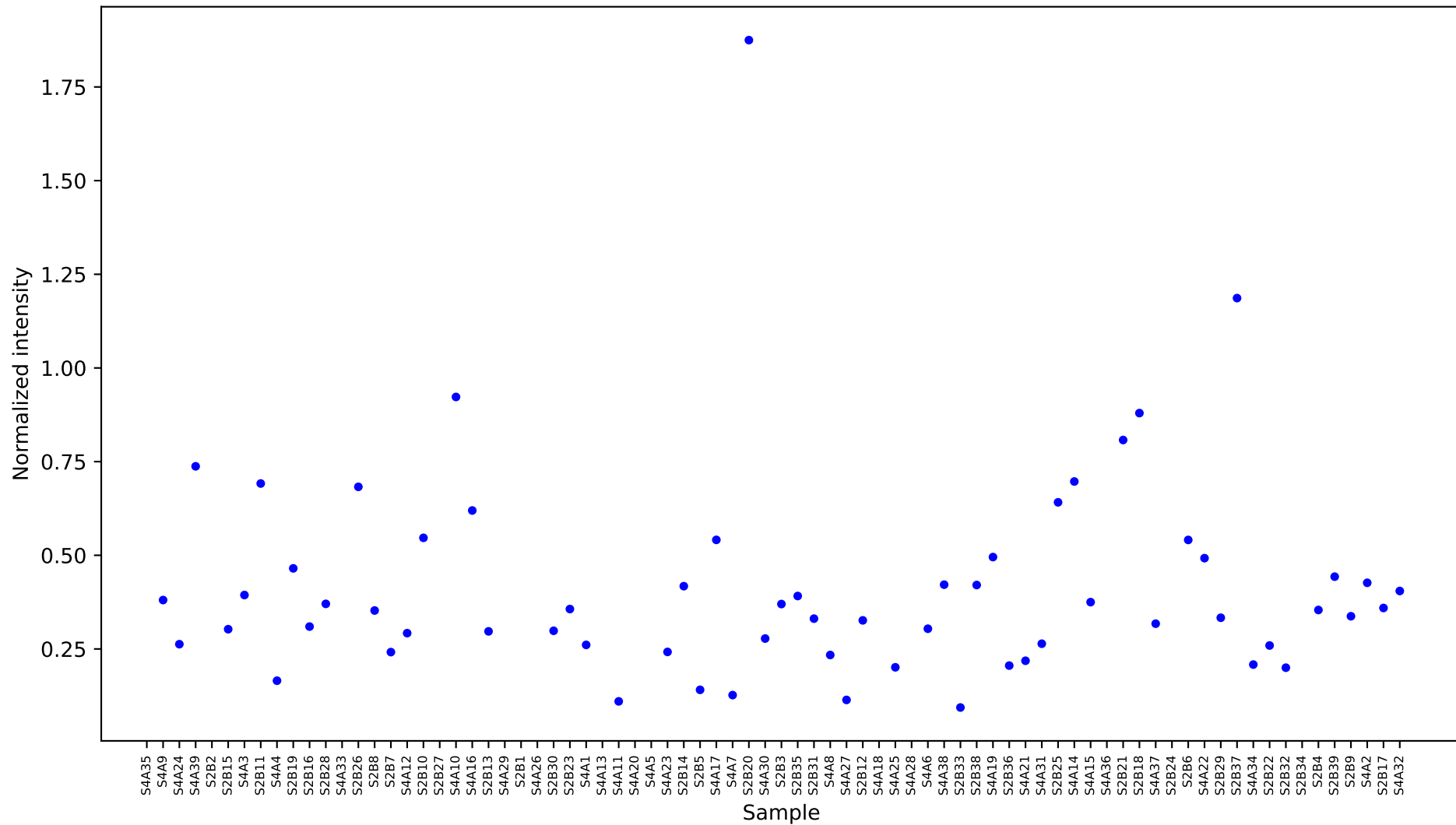
[16219560] lactobionic acid 1 [24.583] Results
