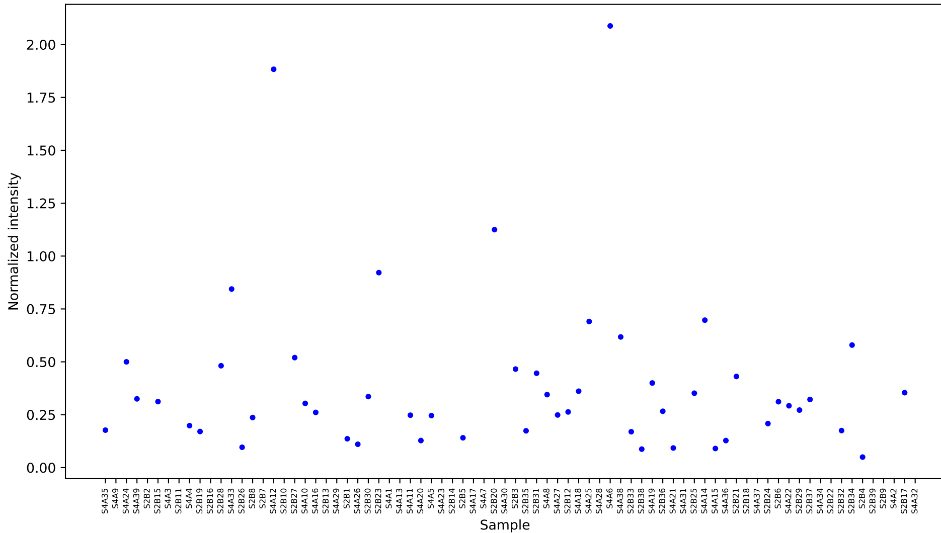
[119] gamma-aminobutyric acid (GABA) [13.326] Results
