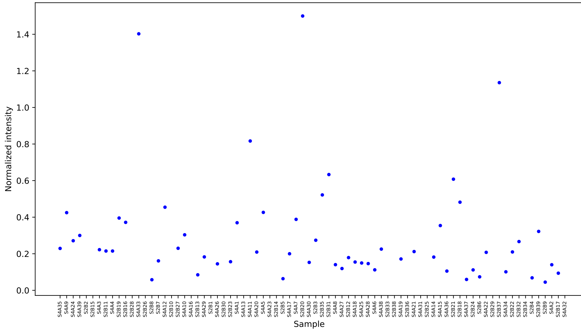
[5202] serotonin 2 [22.767] Results
