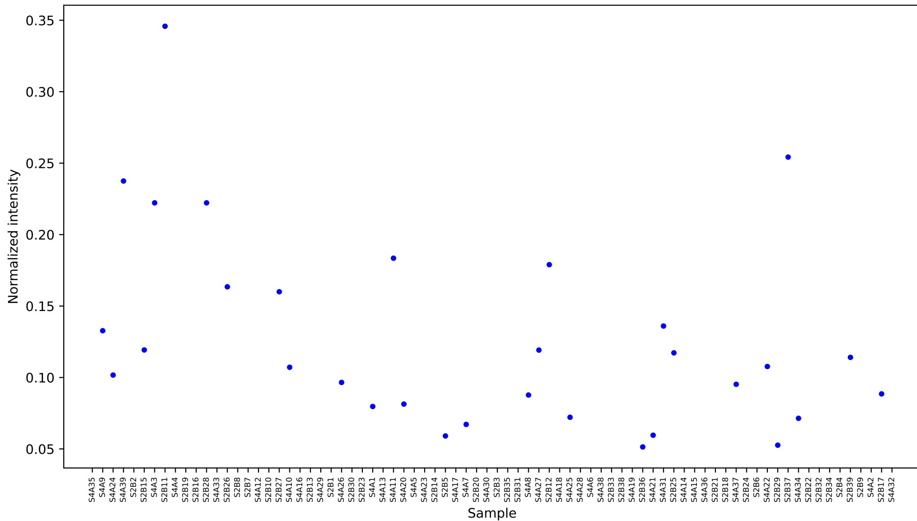
[791] DL-isoleucine 2 [10.225] Results
