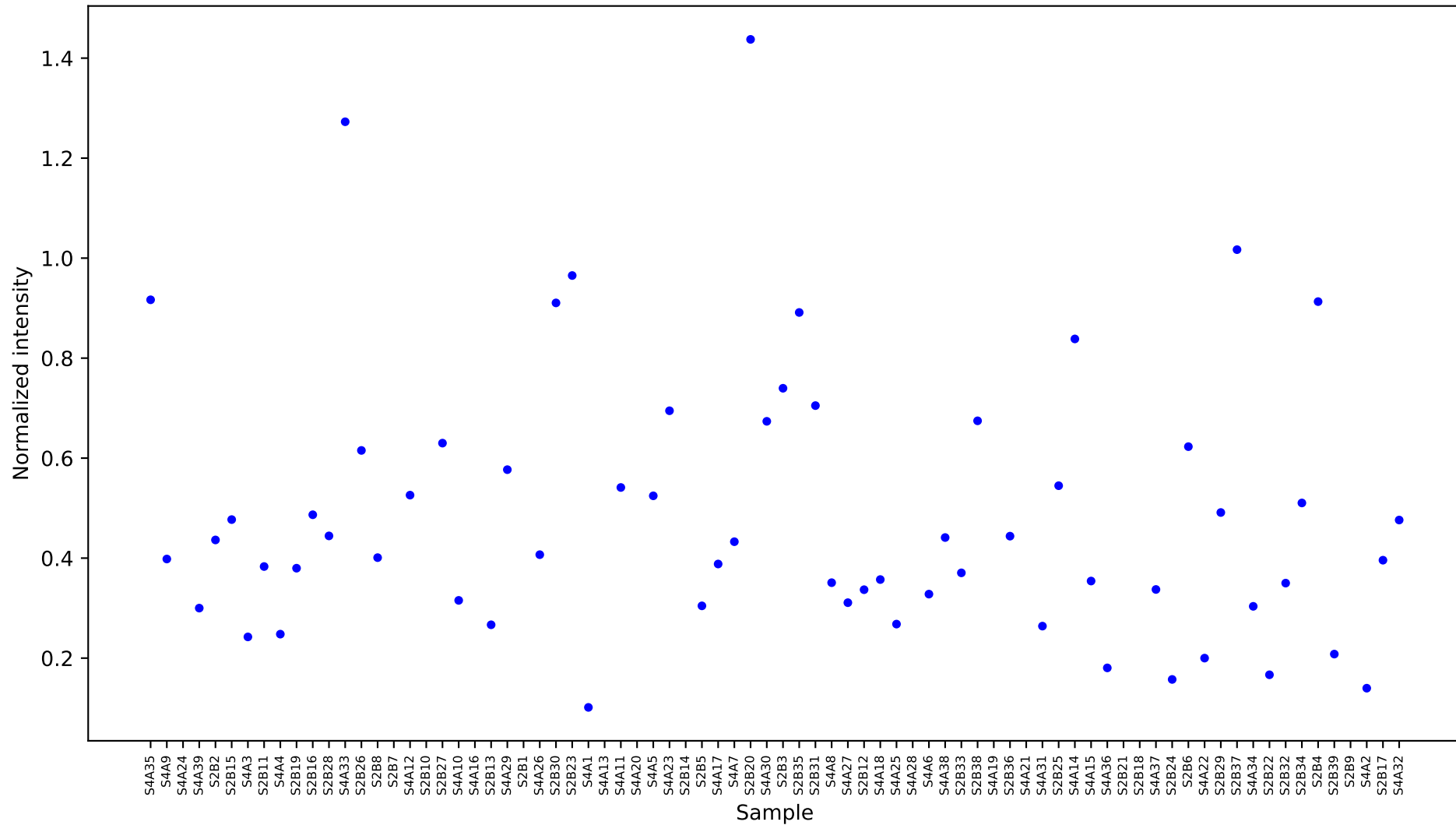
[94214] methyl-beta-D-galactopyranoside [16.935] Results
