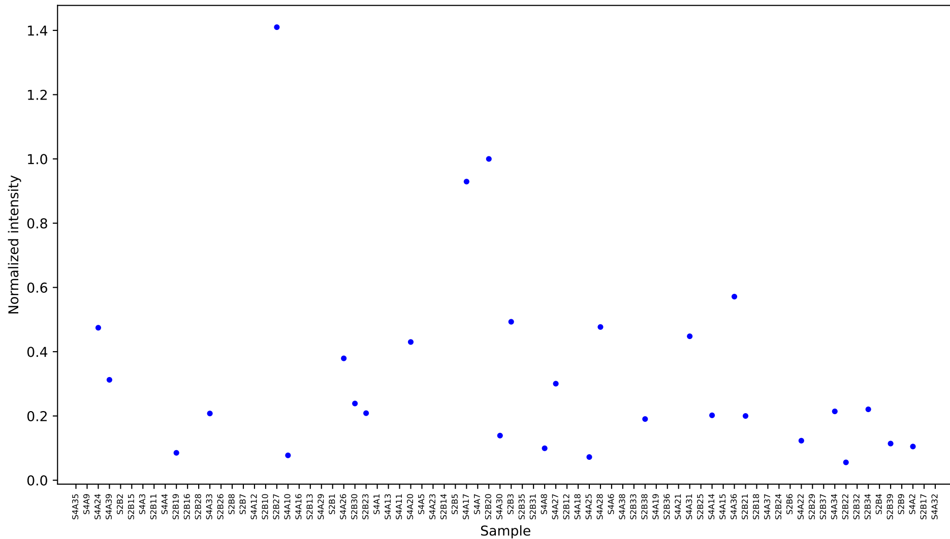
[5950] L-alanine 1 [7.4748] Results
