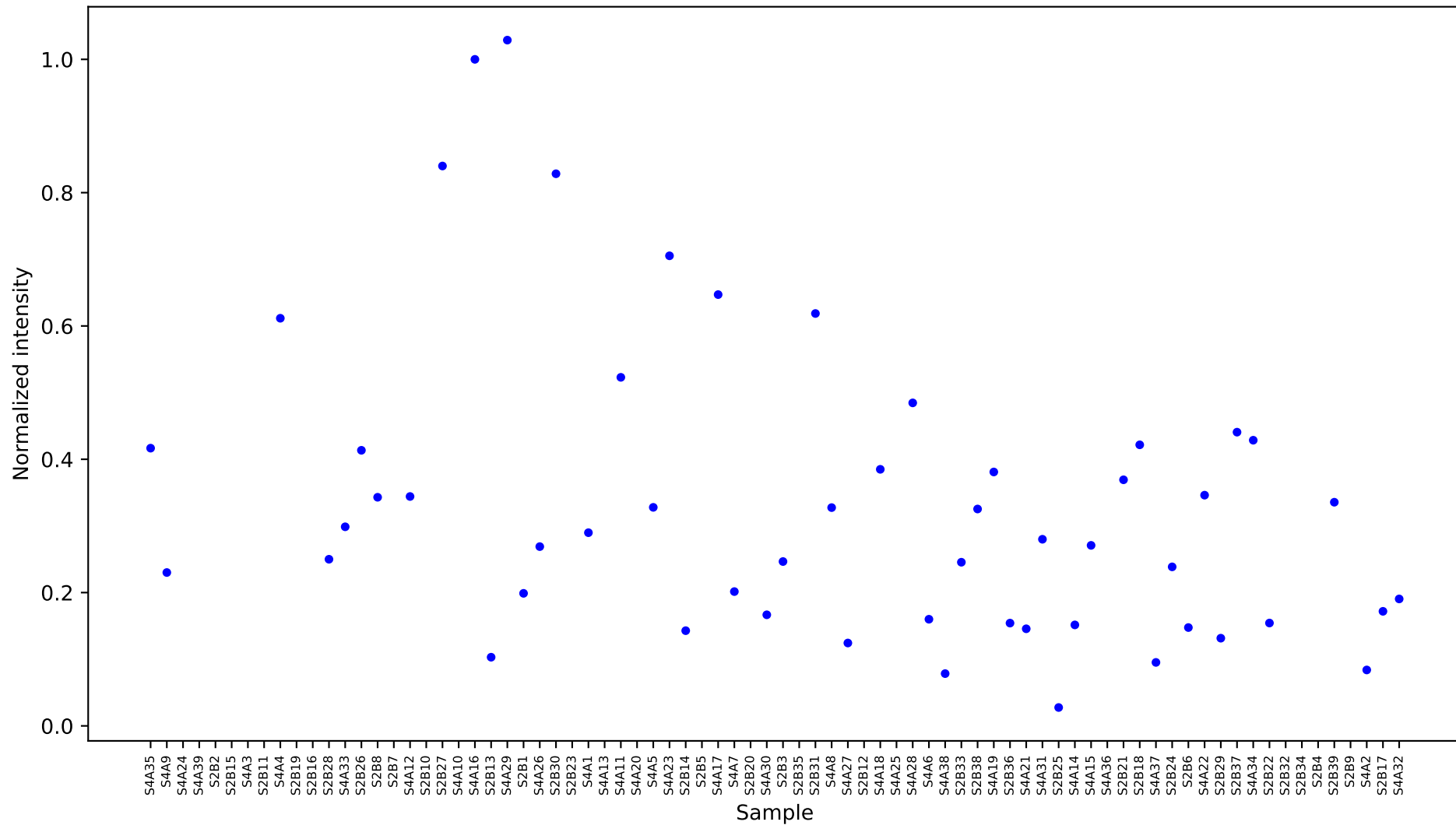
[5962] L-lysine 2 [17.643] Results
