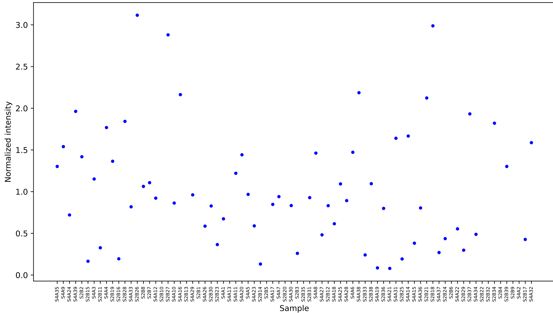
[236] L-asparagine 1 [14.496] Results
