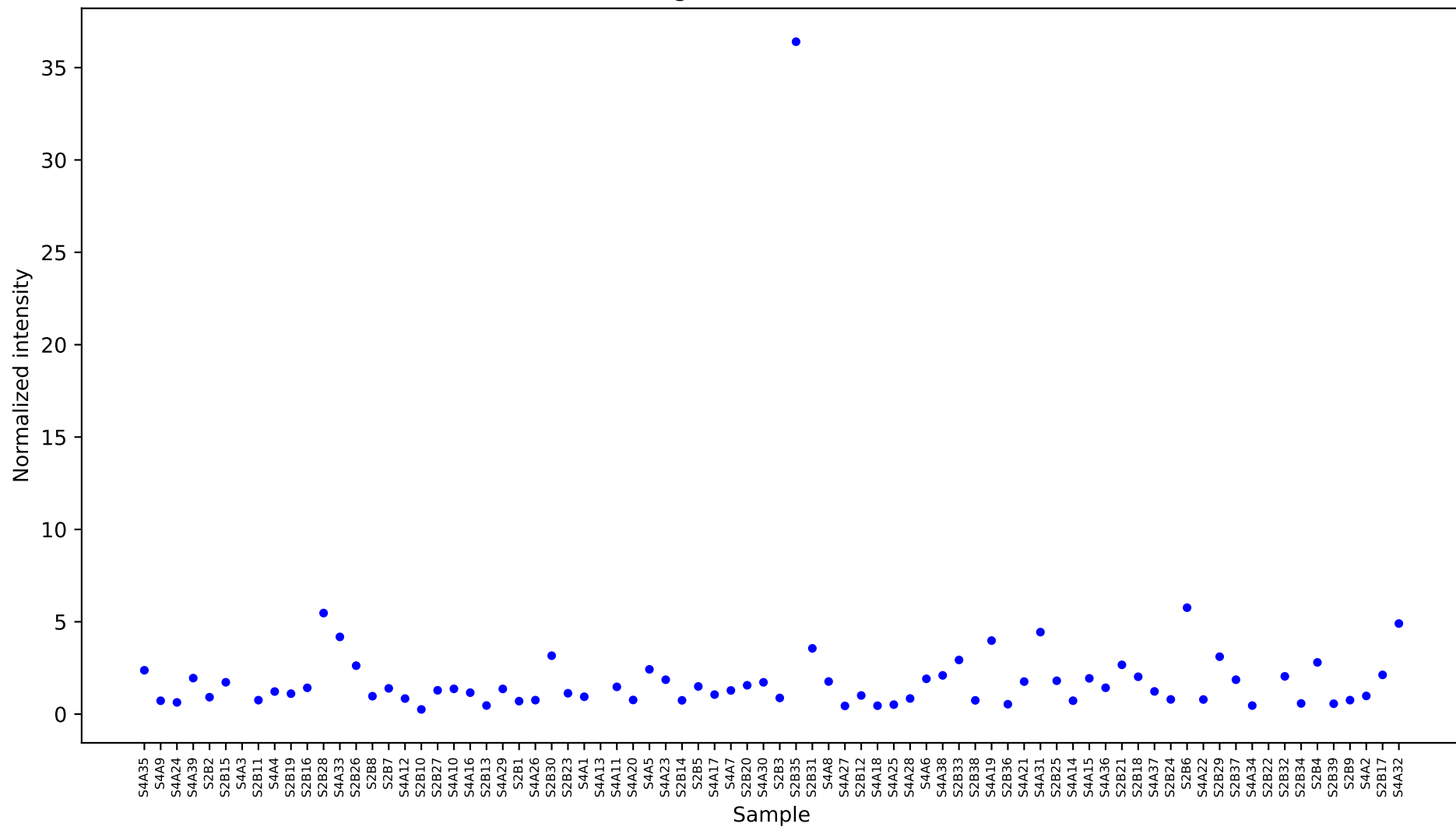
[24749] D-glucose 1 [17.426] Results
