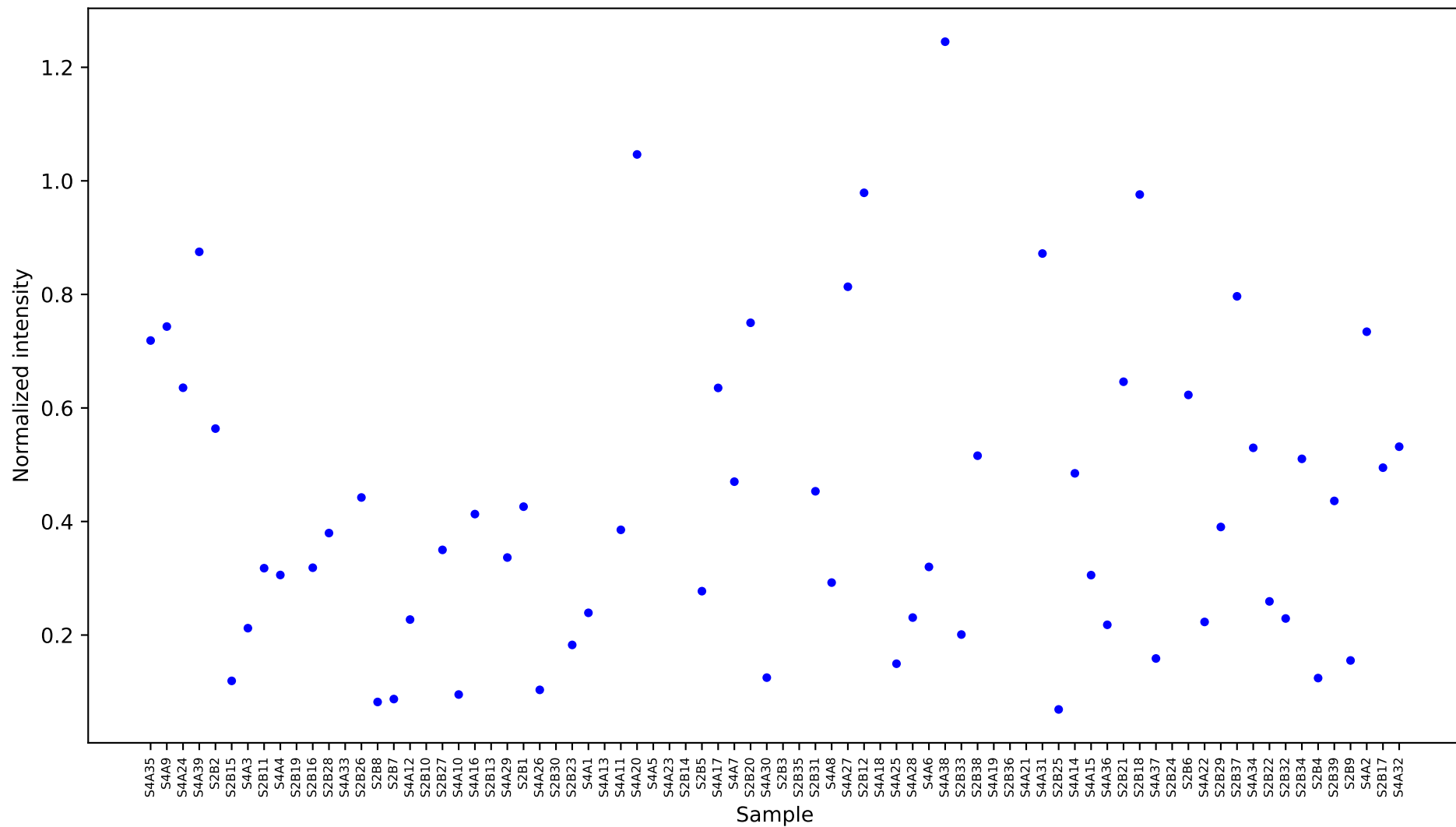
[5202] serotonin 1 [22.532] Results
