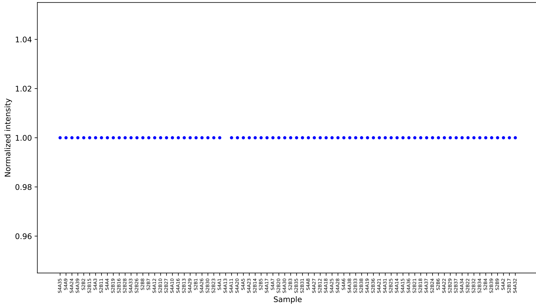
[827] ribitol [15.66] Results
