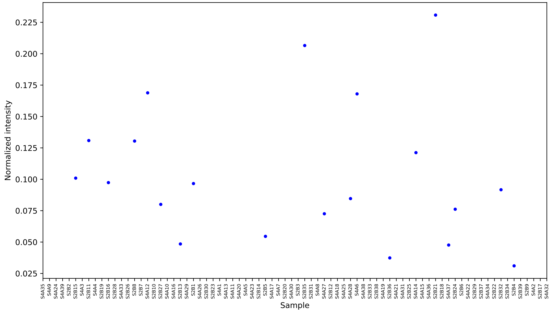
[8871] 2-hydroxypyridine [6.519] Results
