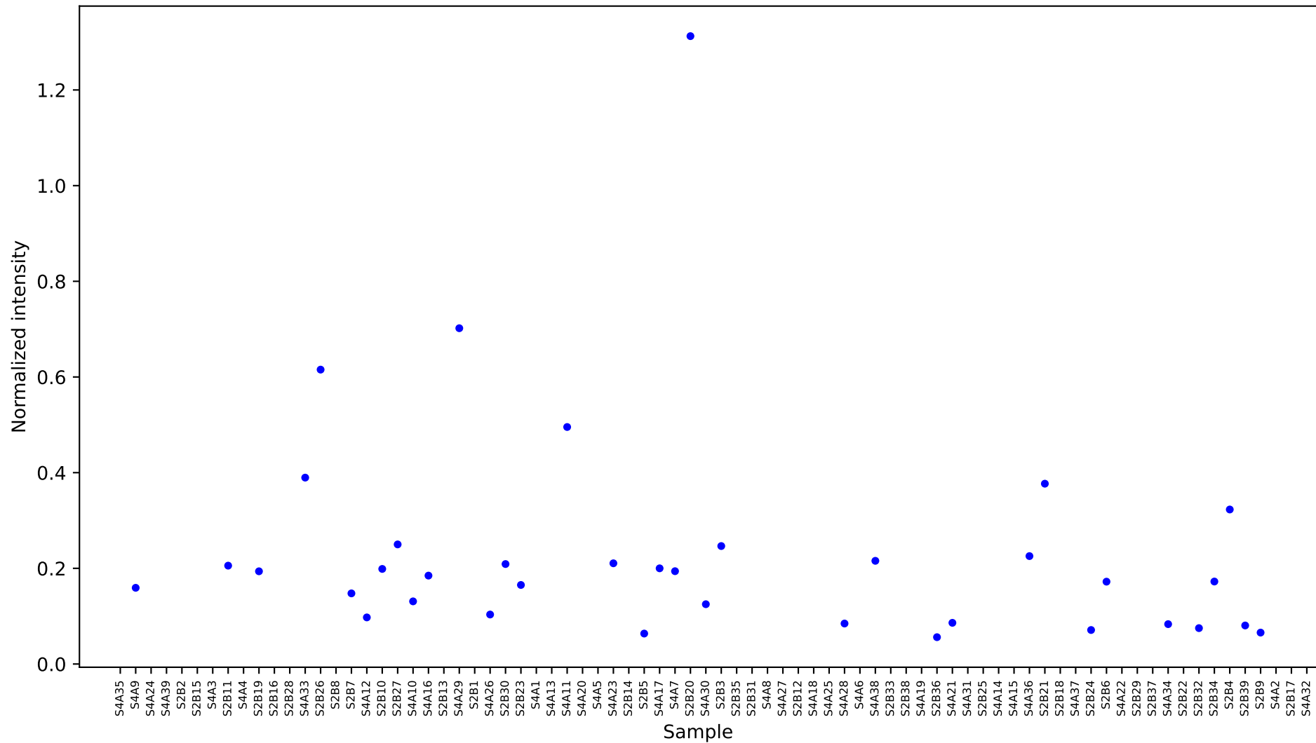
[738] L-glutamine 3 [16.092] Results
