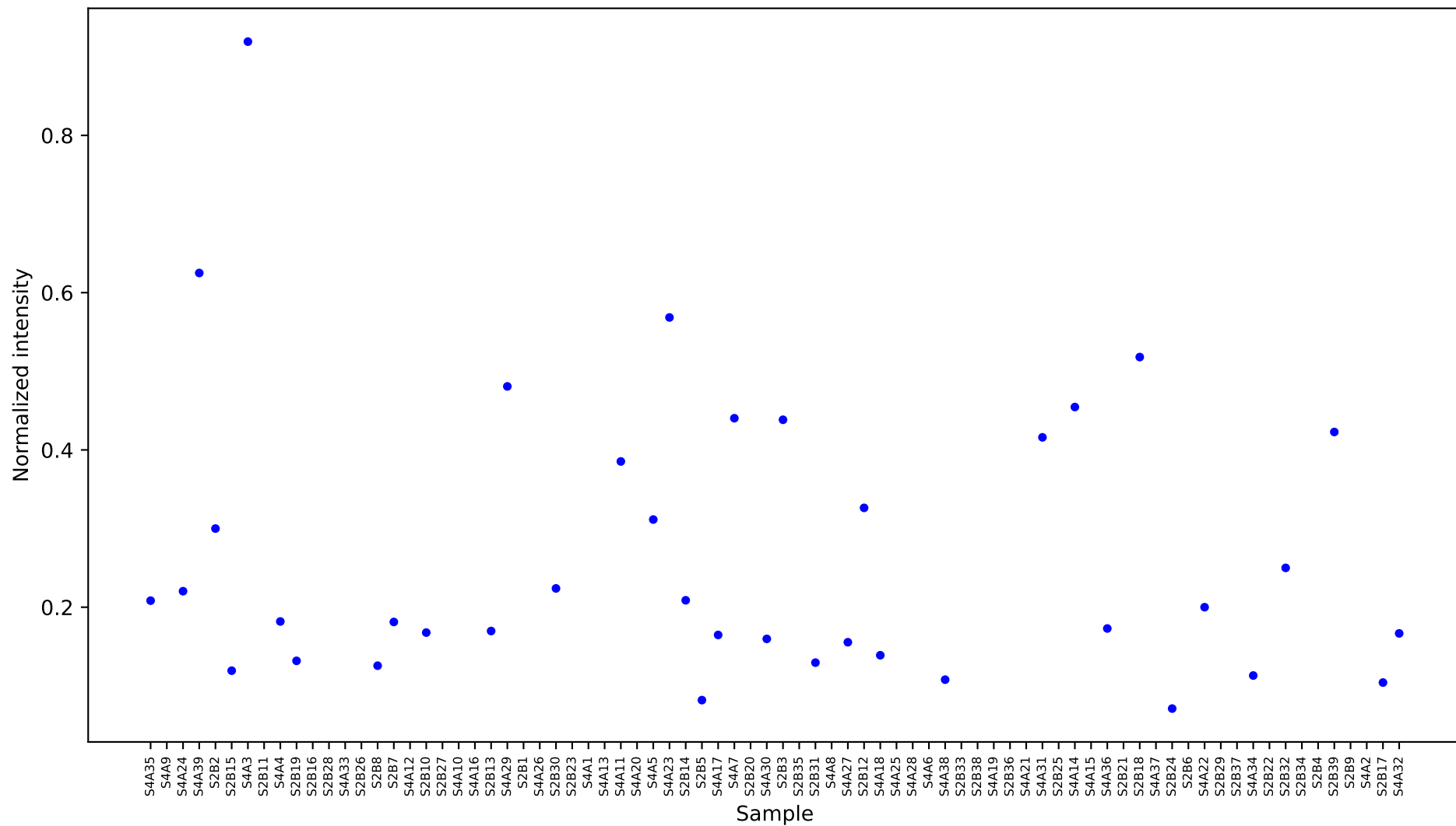
[6288] L-threonine 2 [11.464] Results
