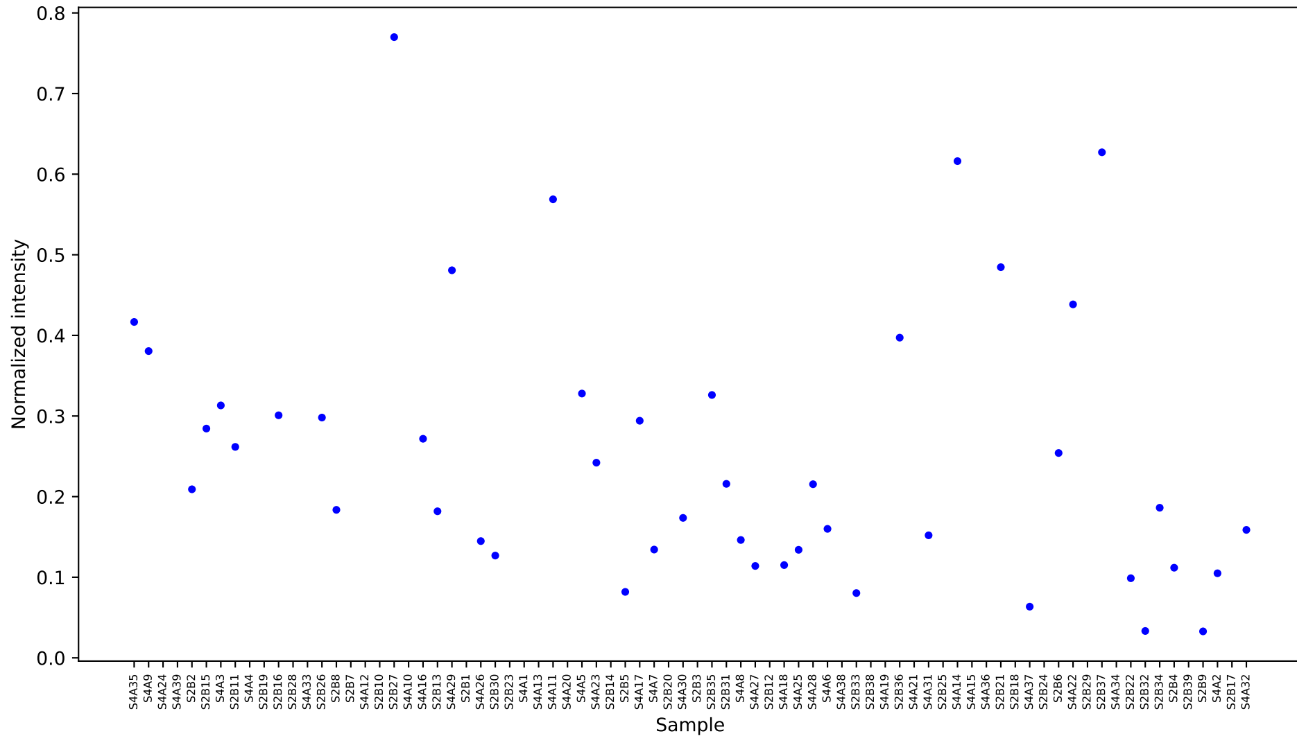
[204] allantoin 3 [19.167] Results
