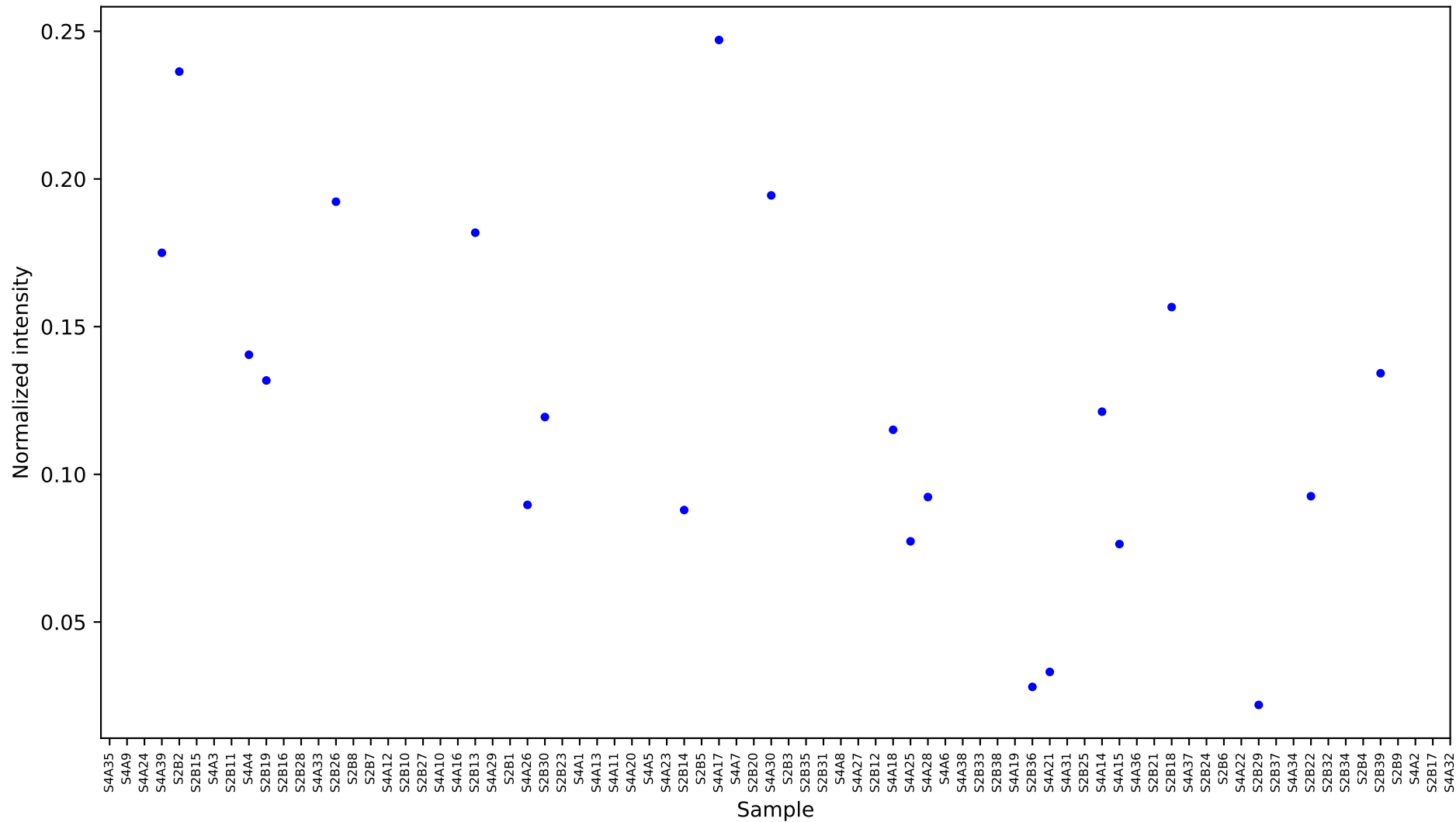
[757] glycolic acid [7.049] Results
