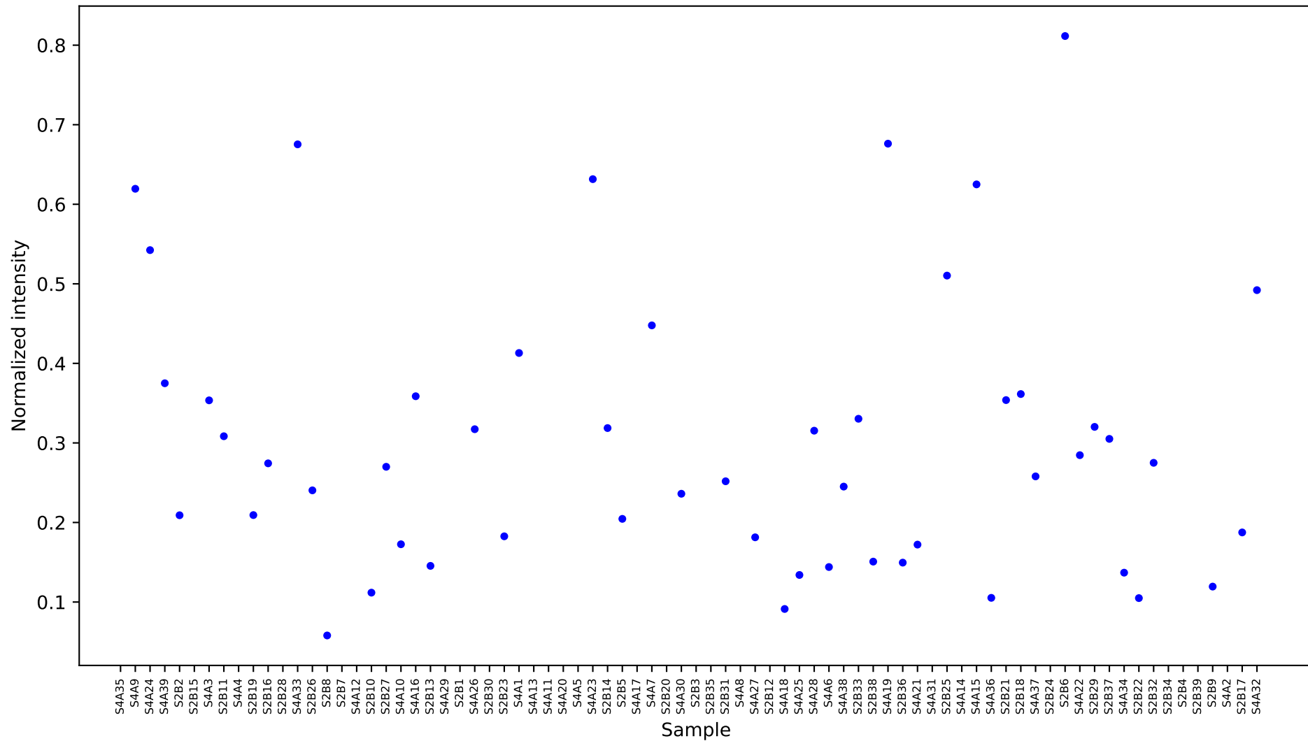
[445858] ferulic acid [19.312] Results
