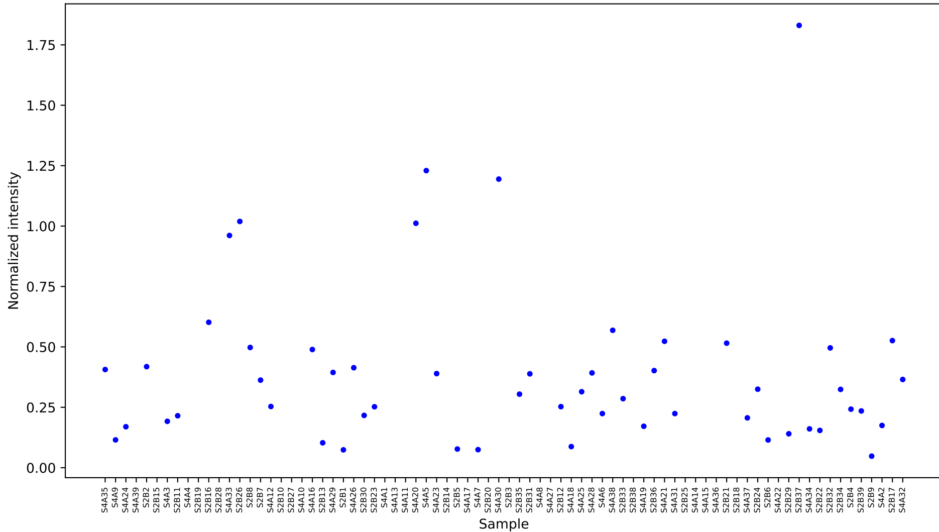
[428] 1,3-diaminopropane 1 [14.708] Results
