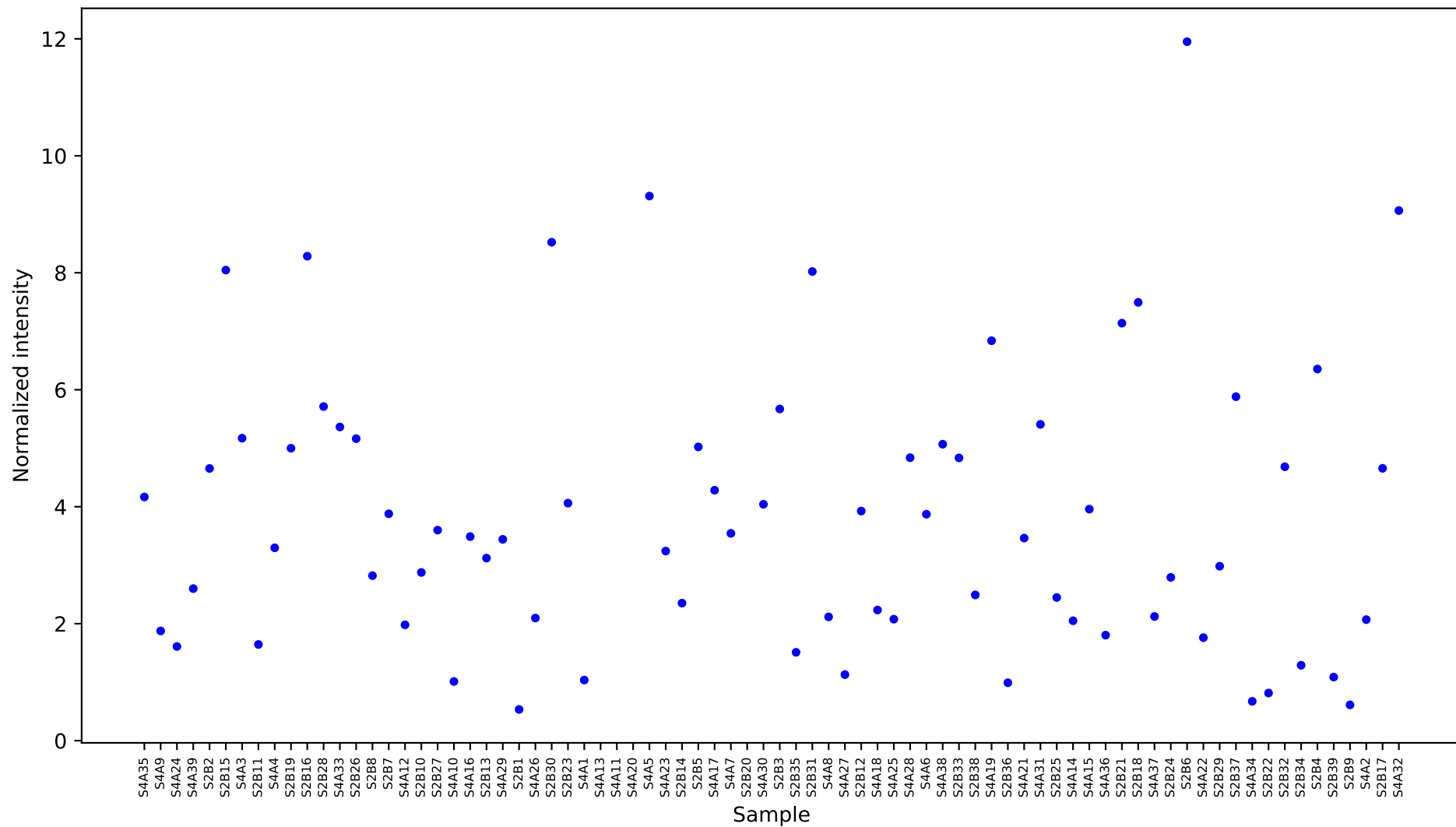
[5950] L-alanine 2 [11.182] Results
