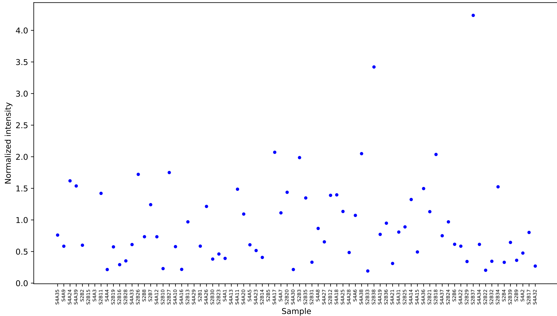
[6508] quinic acid [17.076] Results
