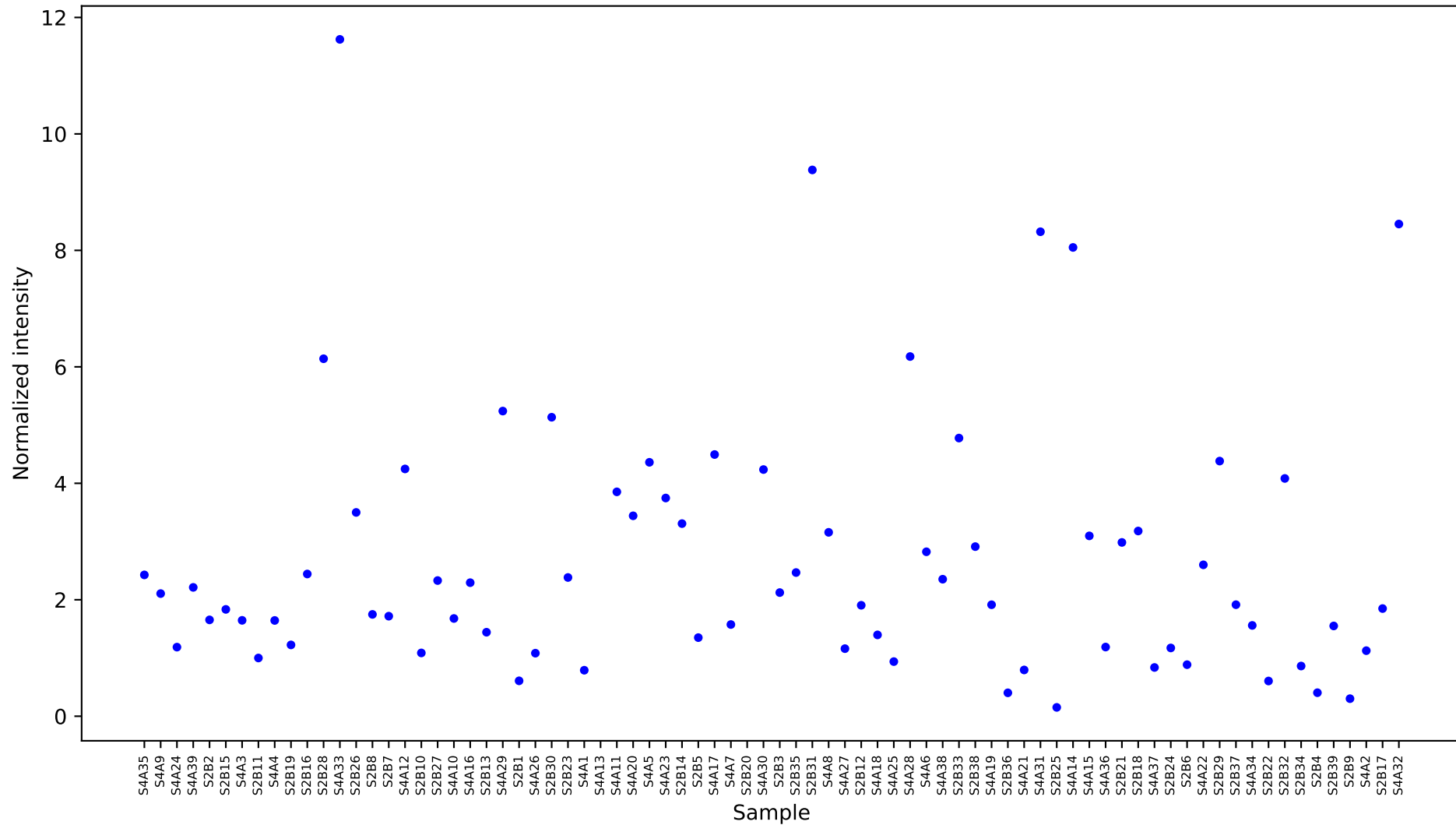
[311] citric acid [16.615] Results
