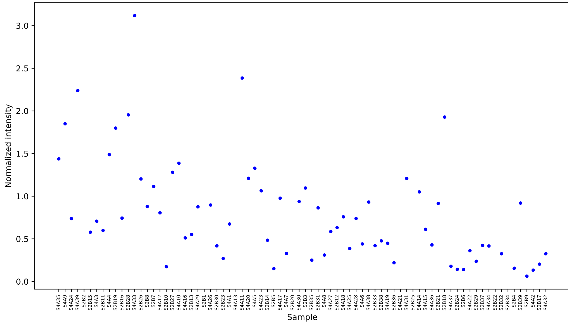
[33032] L-glutamic acid 2 [14.398] Results
