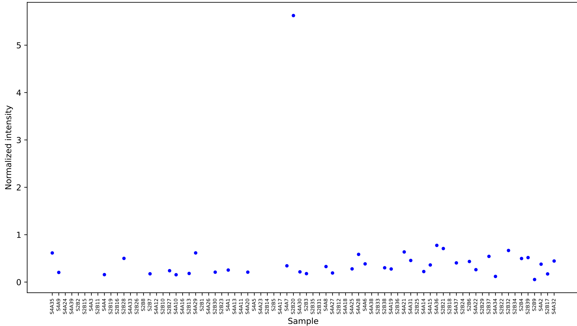
[444972] fumaric acid [10.94] Results
