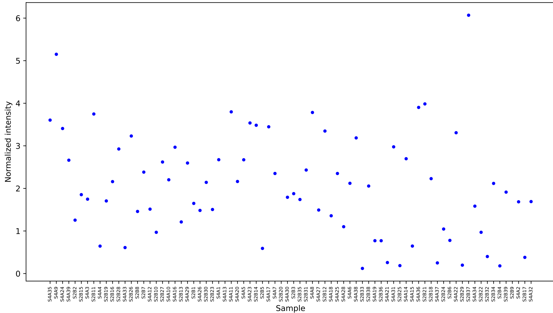
[5960] aspartic acid 2 [13.207] Results
