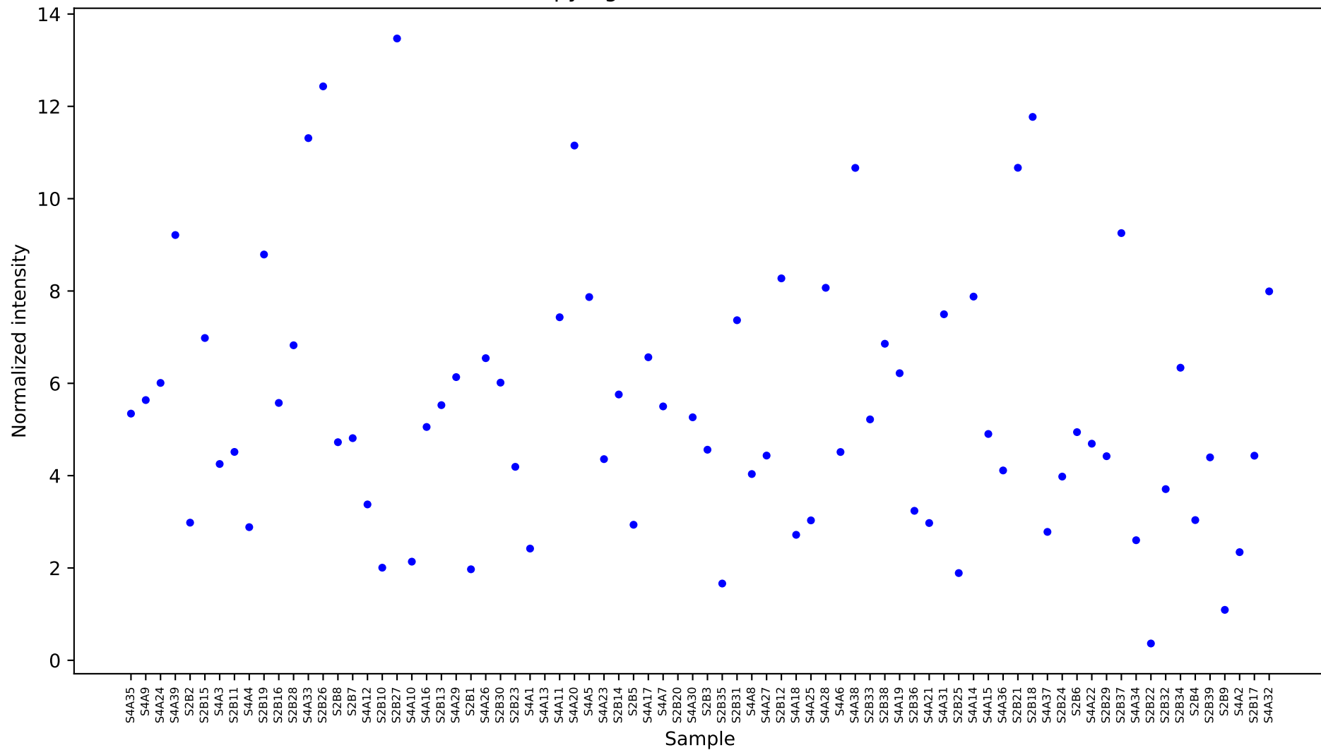
[7405] L-pyroglutamic acid [13.218] Results
