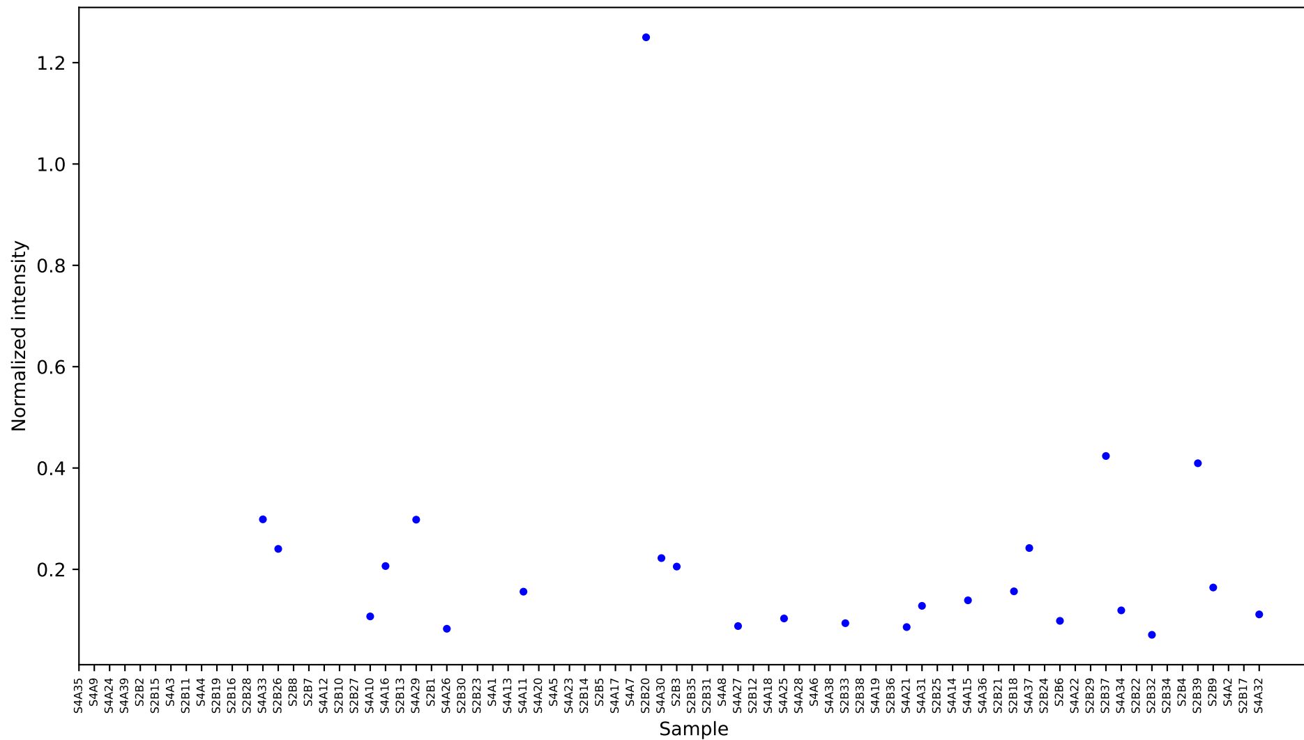
[6106] L-leucine 2 [9.945] Results
