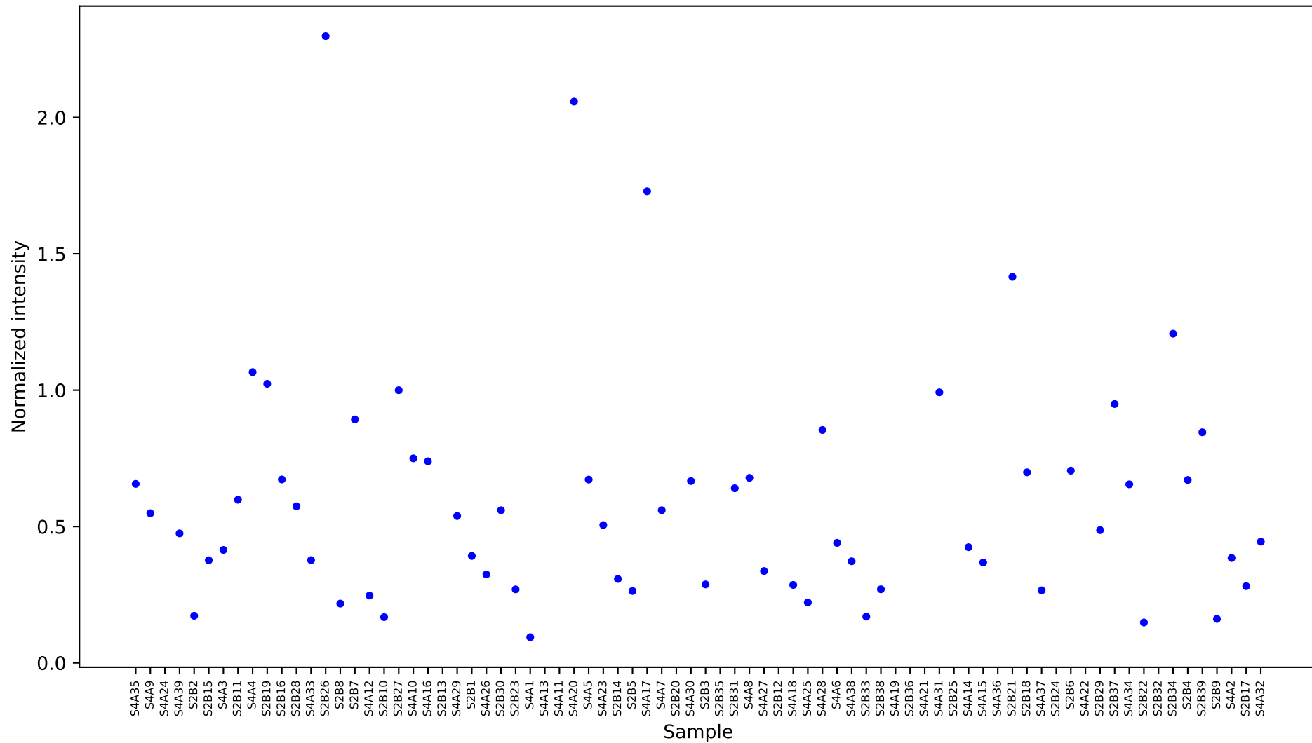
[6057] tyrosine 2 [17.871] Results
