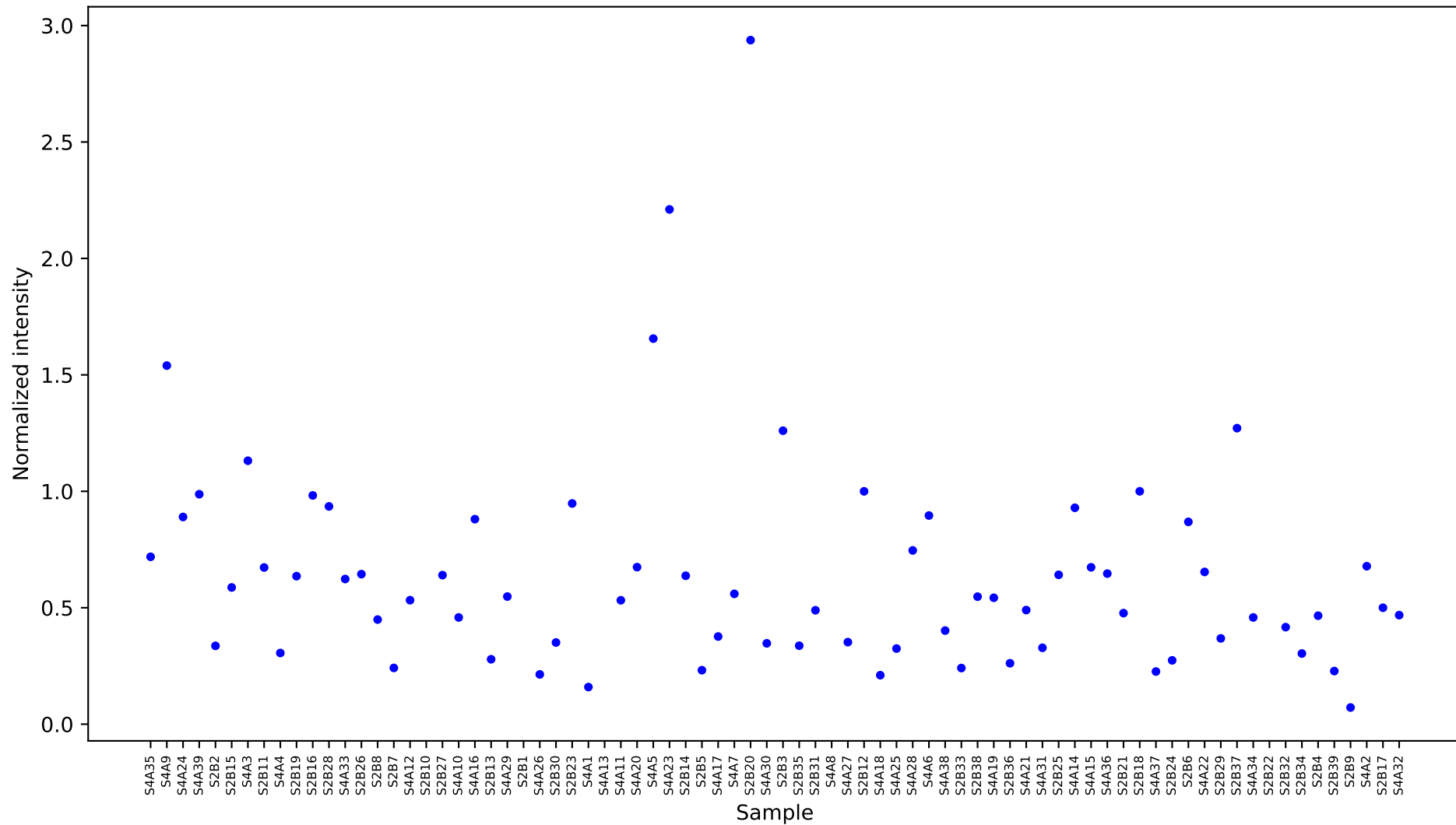
[101713] glucoheptonic acid 2 [19.615] Results
