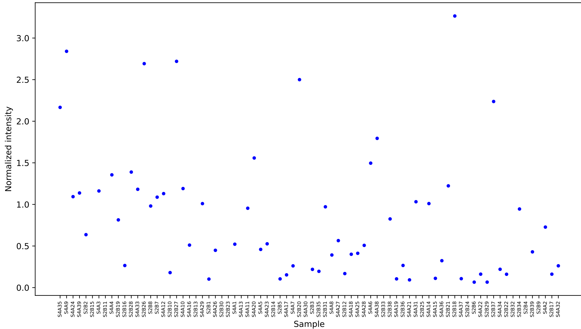
[236] L-asparagine 2 [14.984] Results
