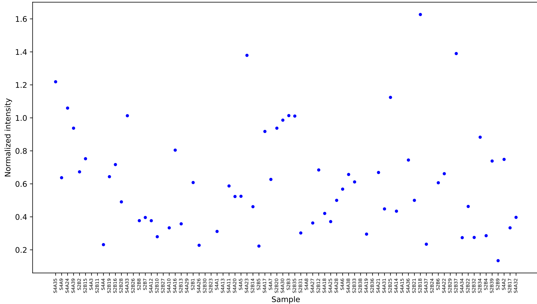
[439958] D-glucose-6-phosphate 2 [21.558] Results
