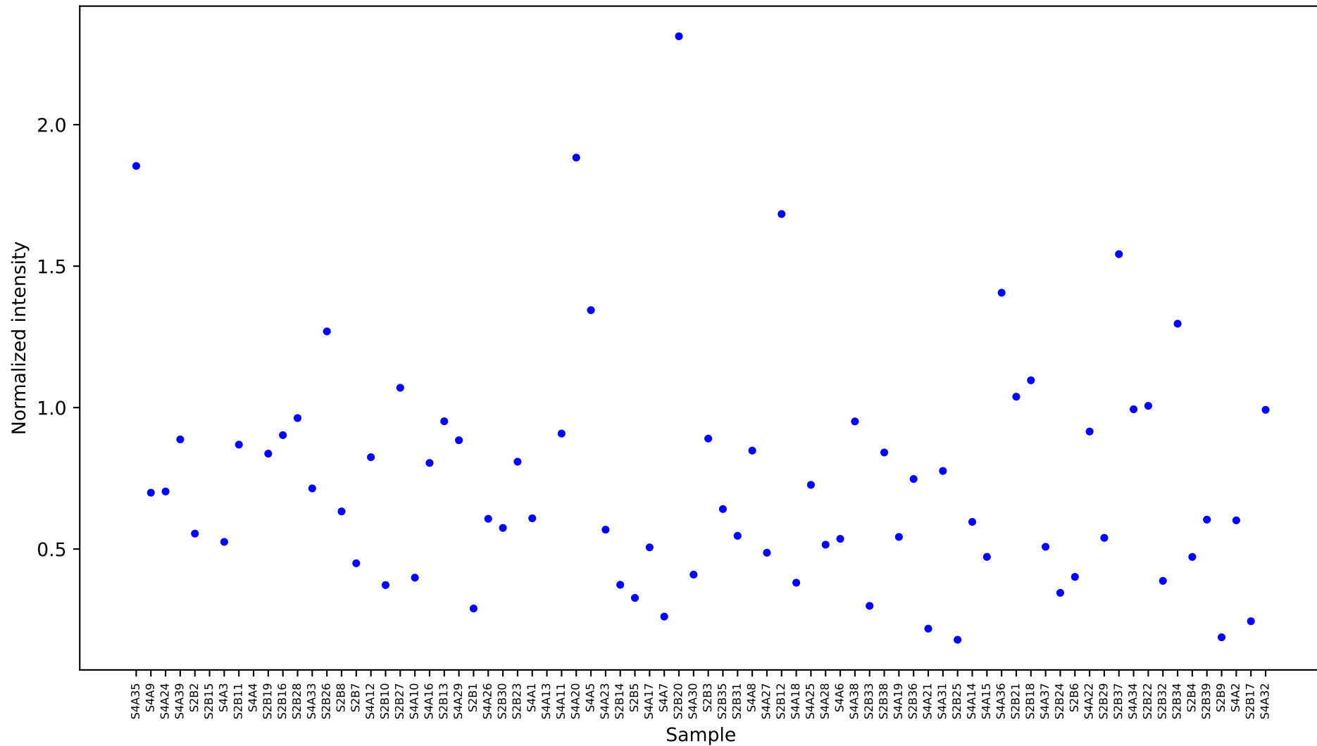
[754] glycerol 1-phosphate [16.056] Results
