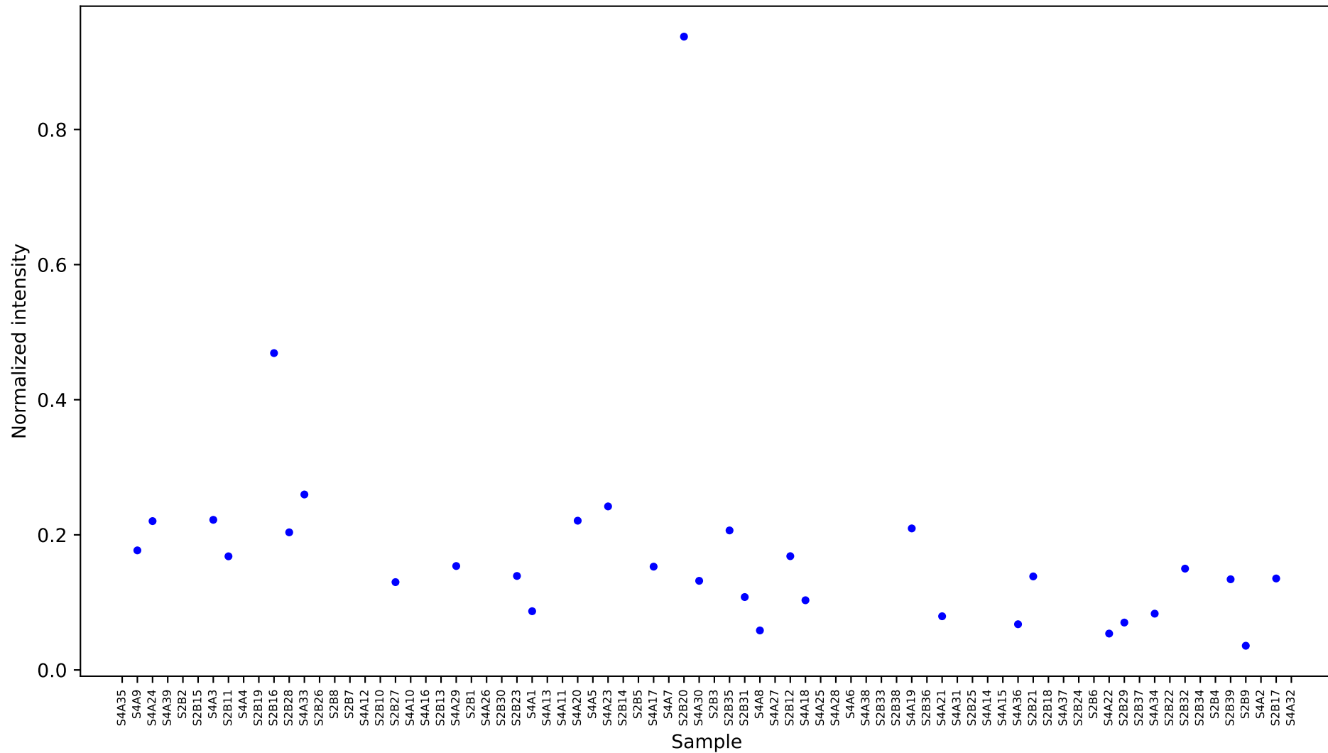
[439742] beta-cyano-L-alanine [11.288] Results
