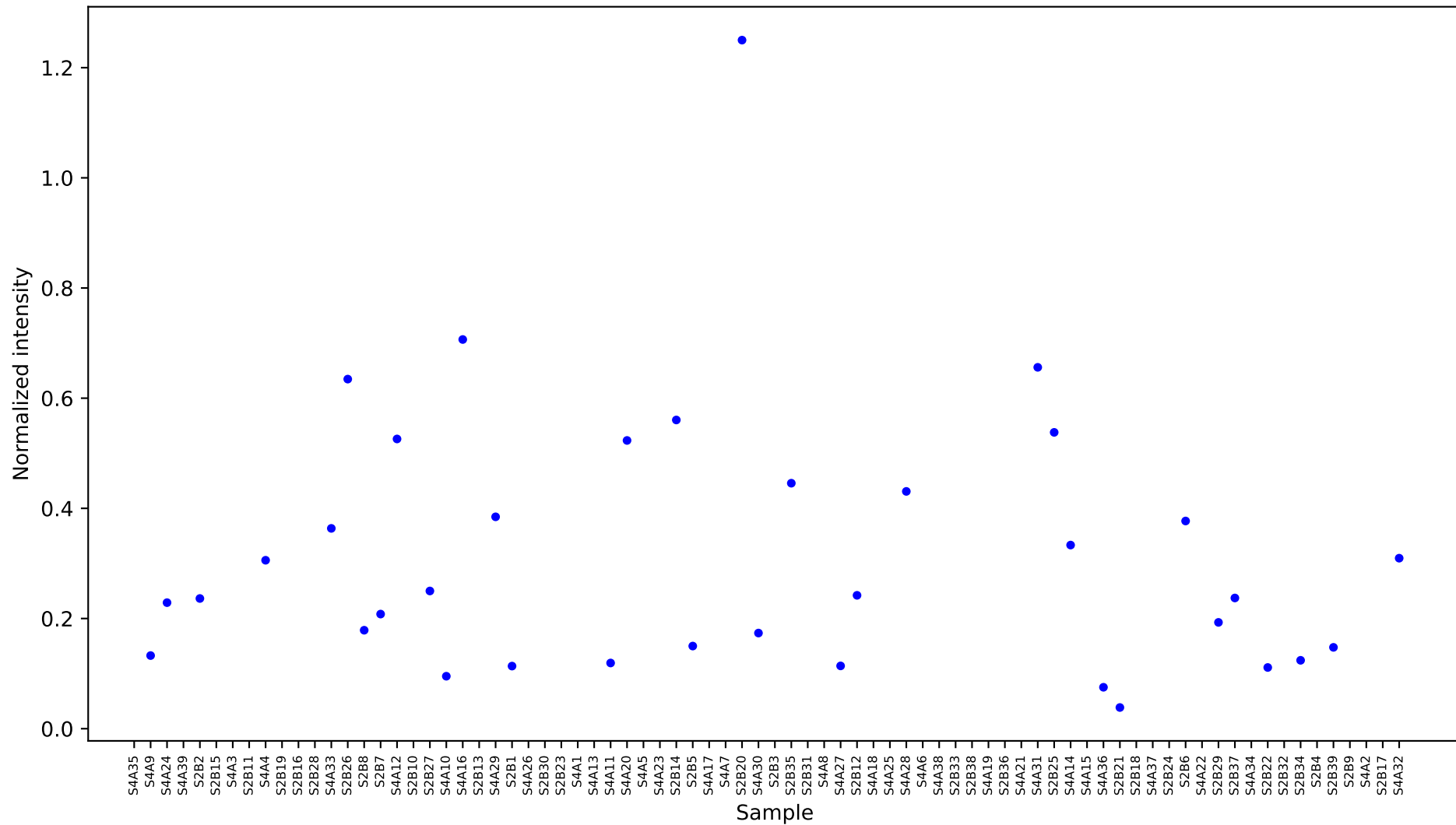
[1110] succinic acid [10.509] Results
