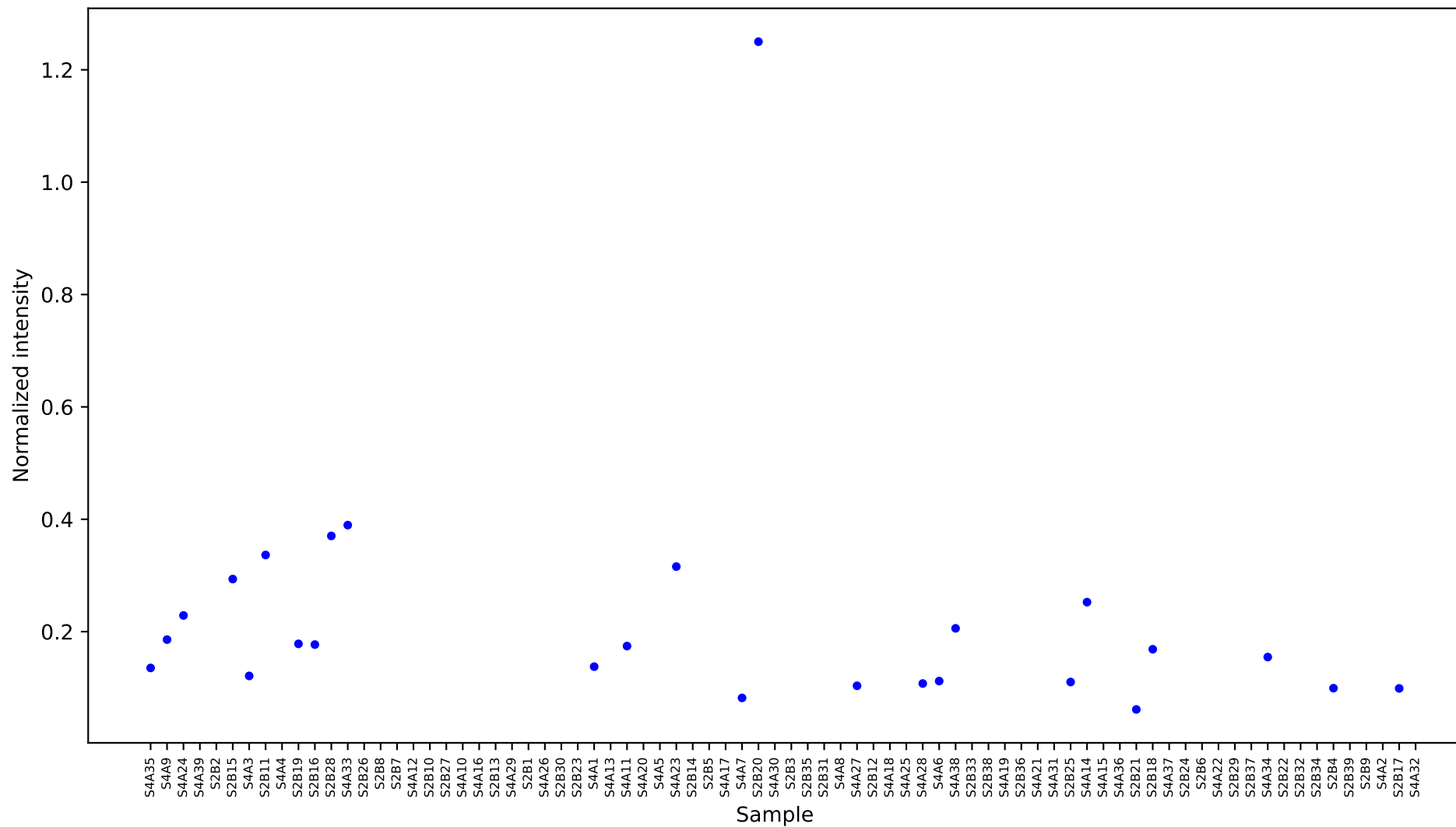
[638129] citraconic acid [10.792] Results
