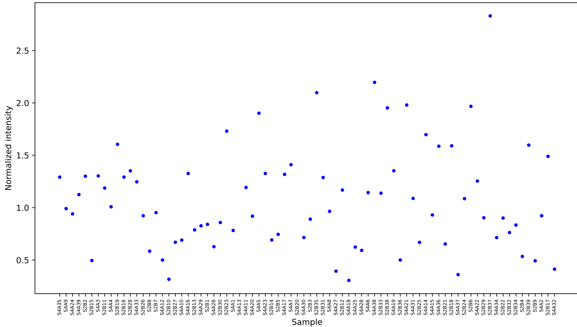
[985] palmitic acid [18.846] Results
