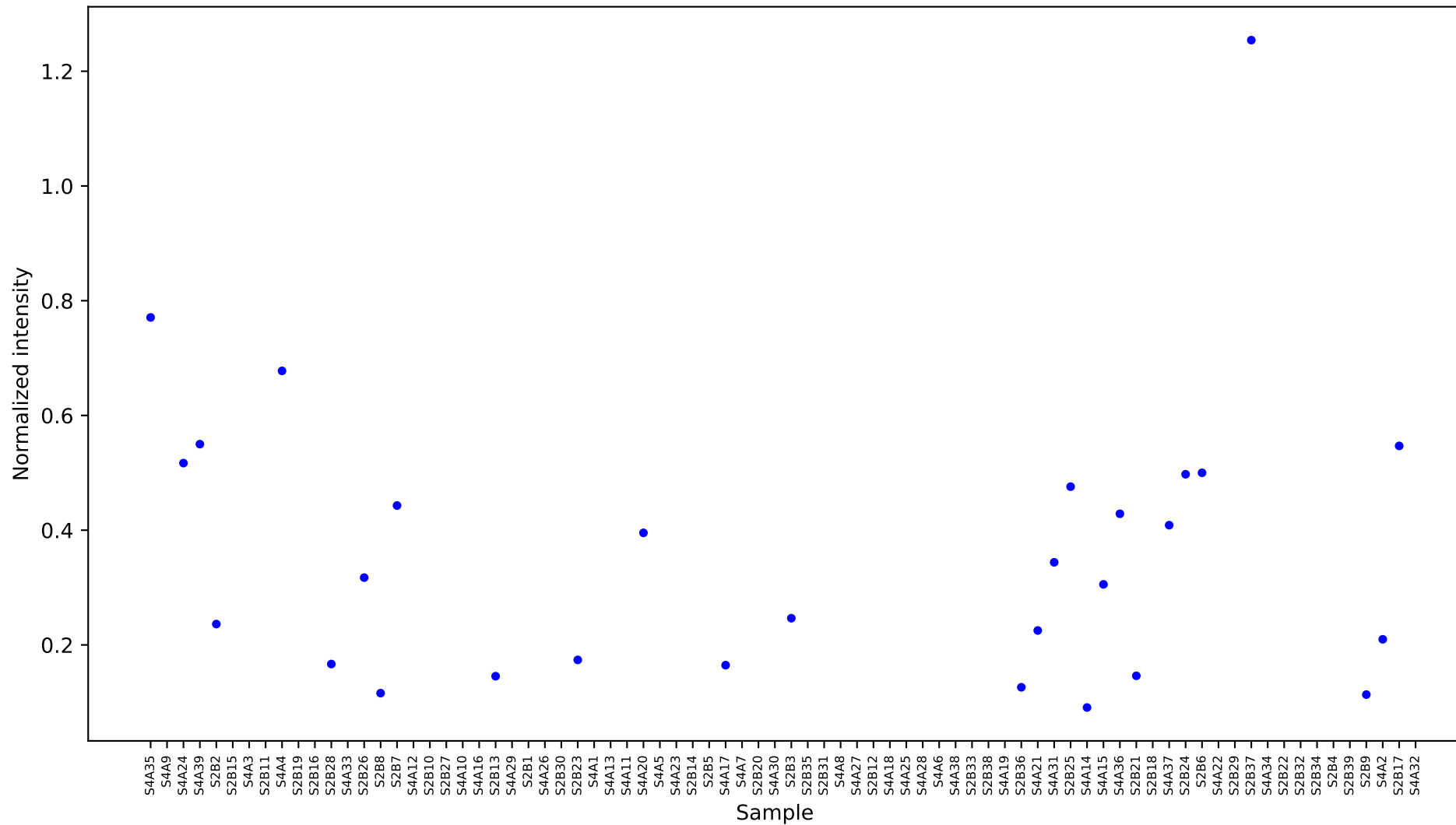
[760] glyoxylic acid [10.813] Results
