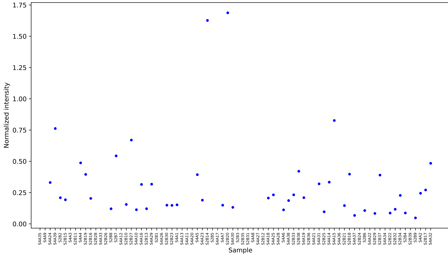
[190] adenine 1 [17.066] Results
