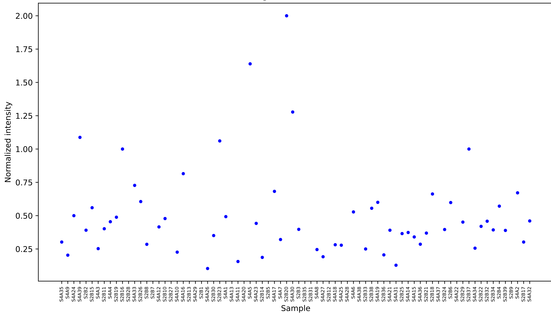
[441422] beta-gentiobiose 2 [25.42] Results
