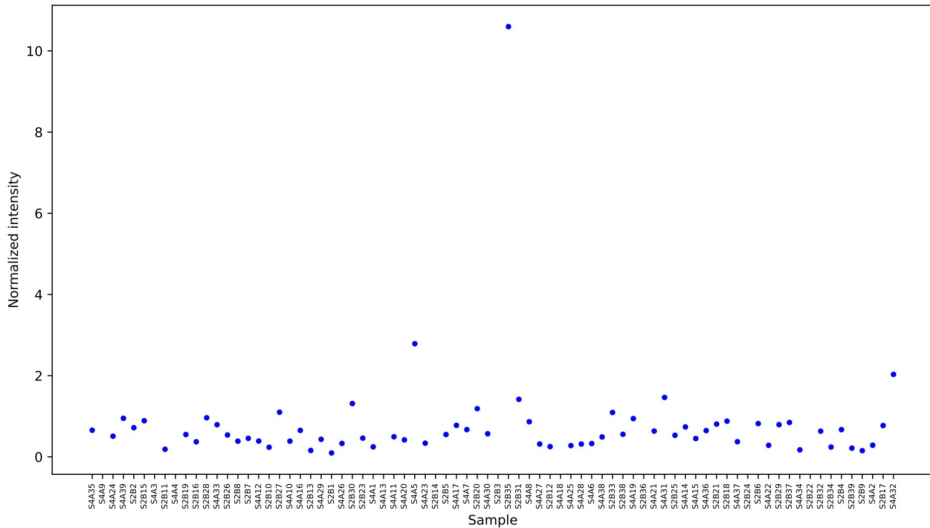
[448388] D-allose 2 [17.521] Results
