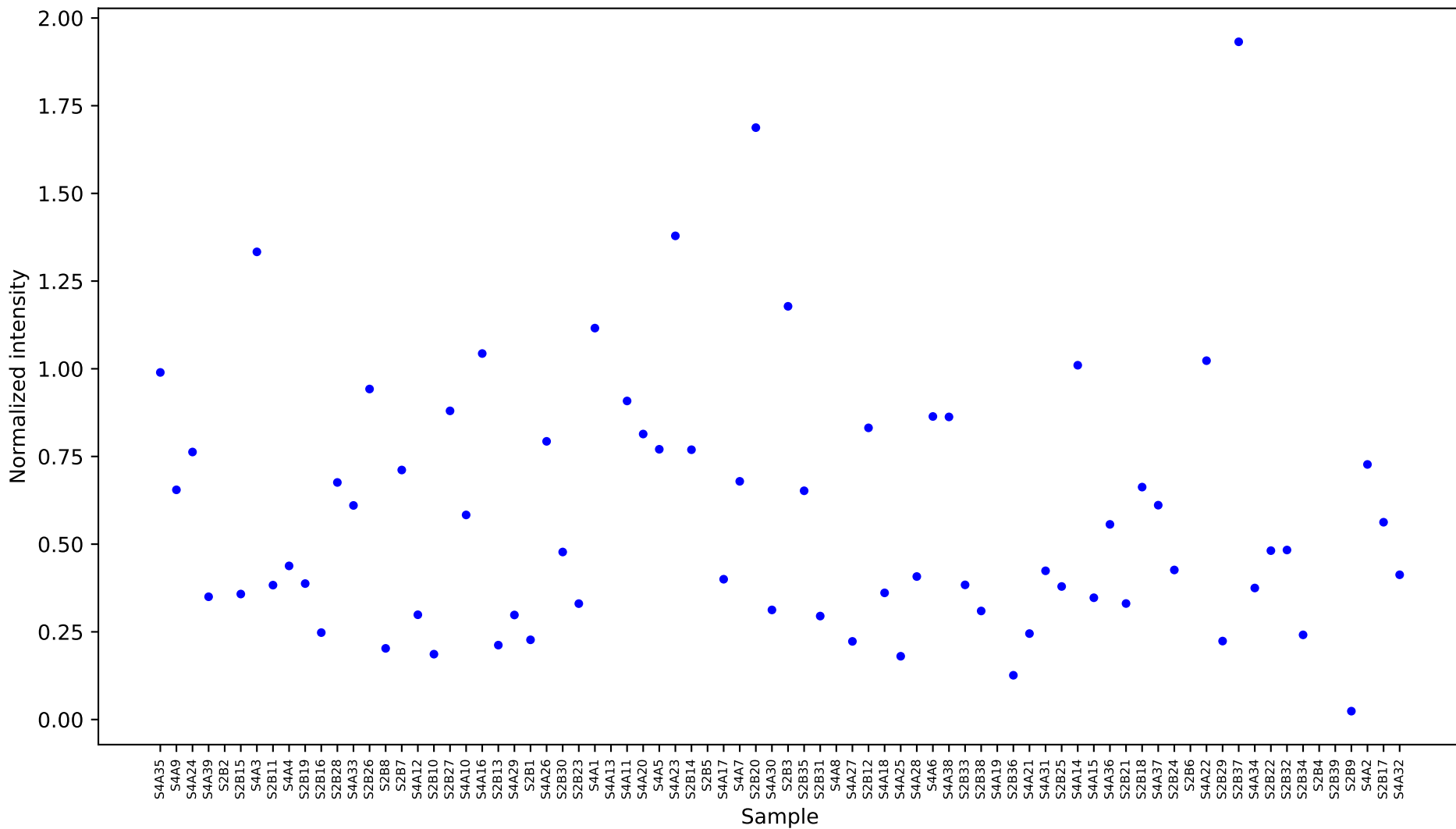
[5460407] threonic acid [13.652] Results
