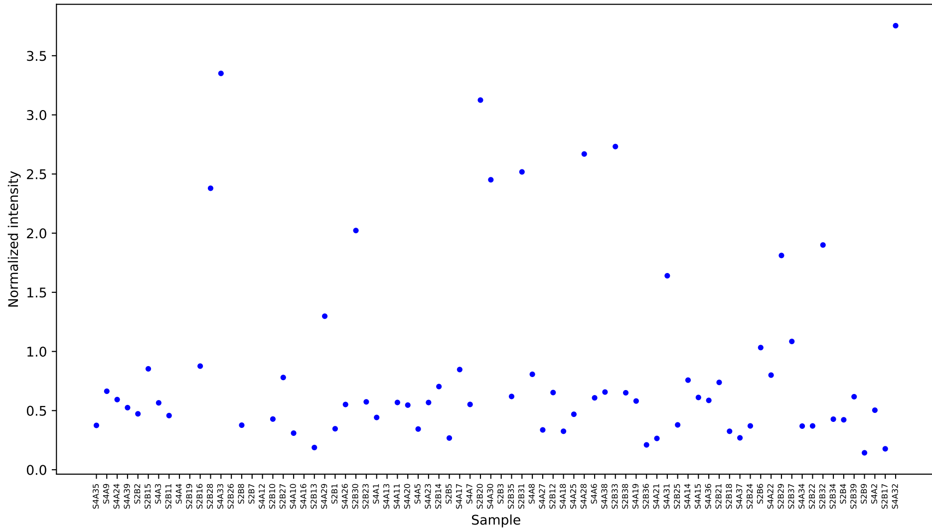
[439451] galactinol 2 [26.479] Results
