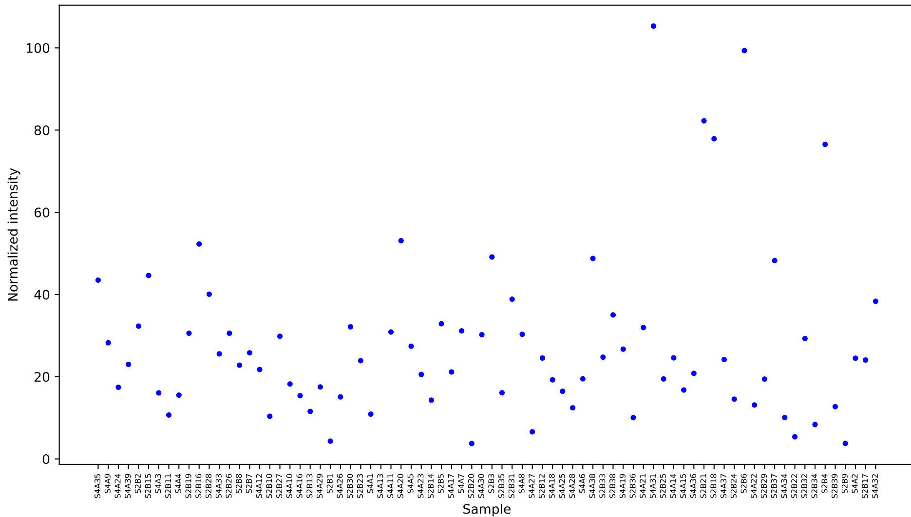
[5988] Sucrose [23.988] Results
