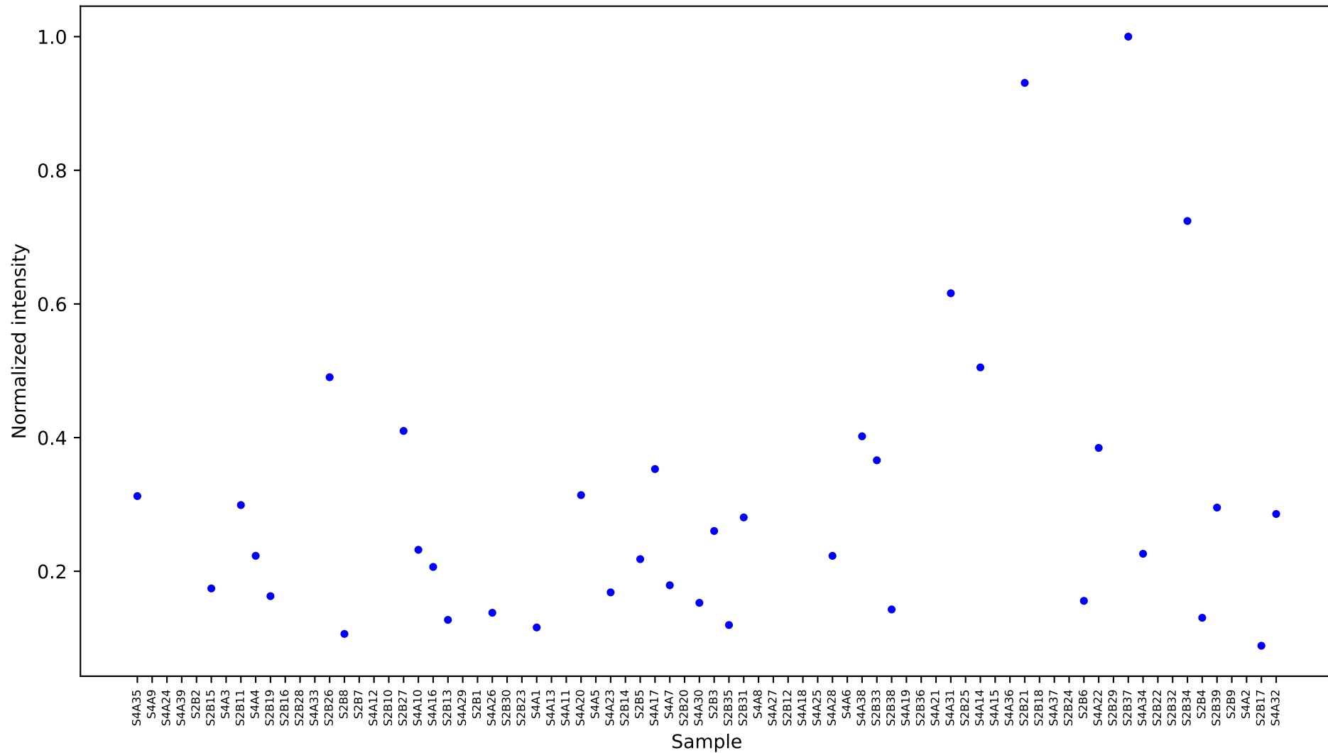
[239] Beta- alanine 1 [12.044] Results
