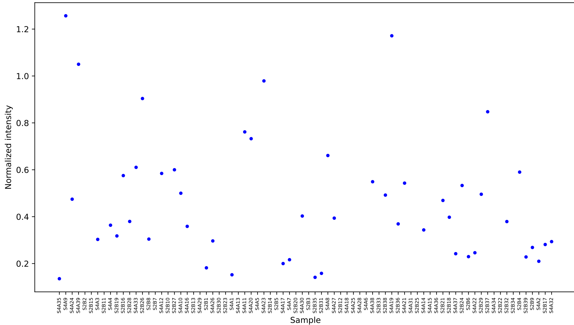
[439194] glyceric acid [10.735] Results
