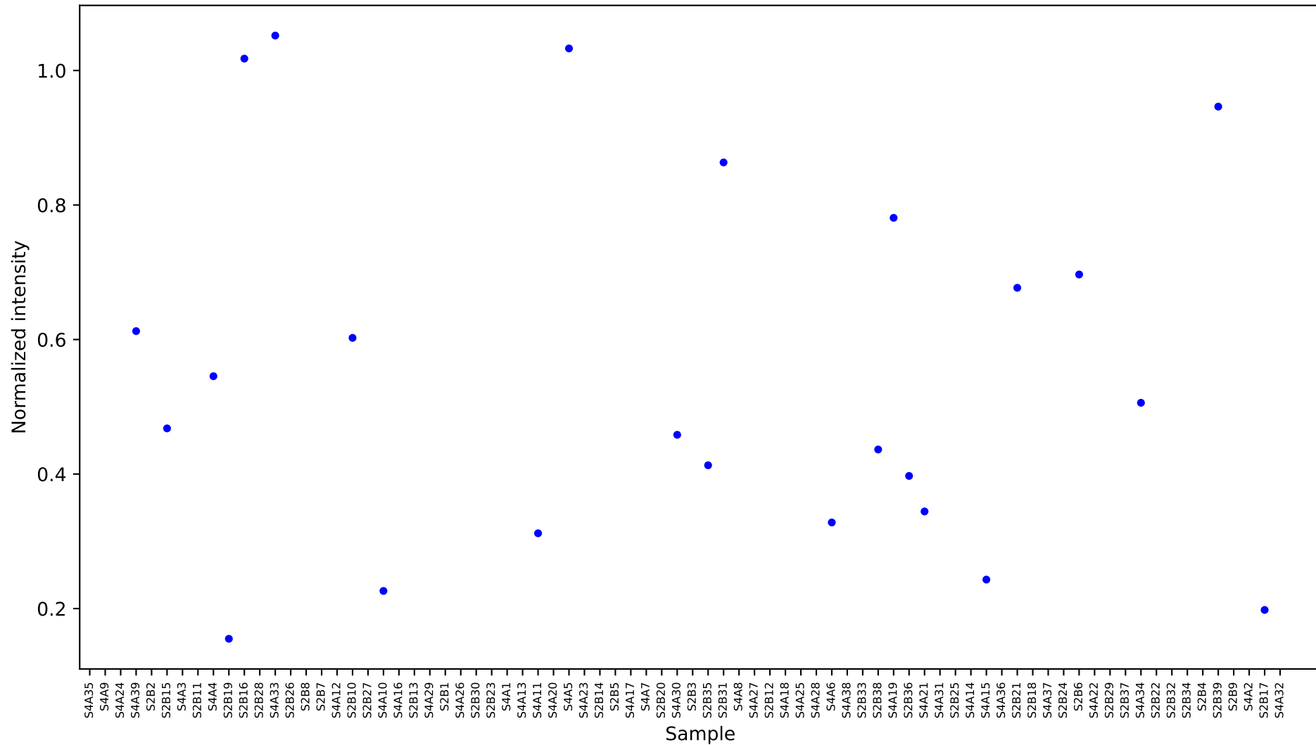
[1004] phosphoric acid [9.966] Results
