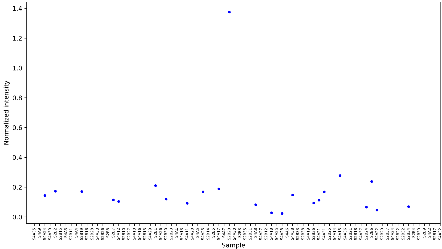
[107689] L-(+) lactic acid [6.851] Results
