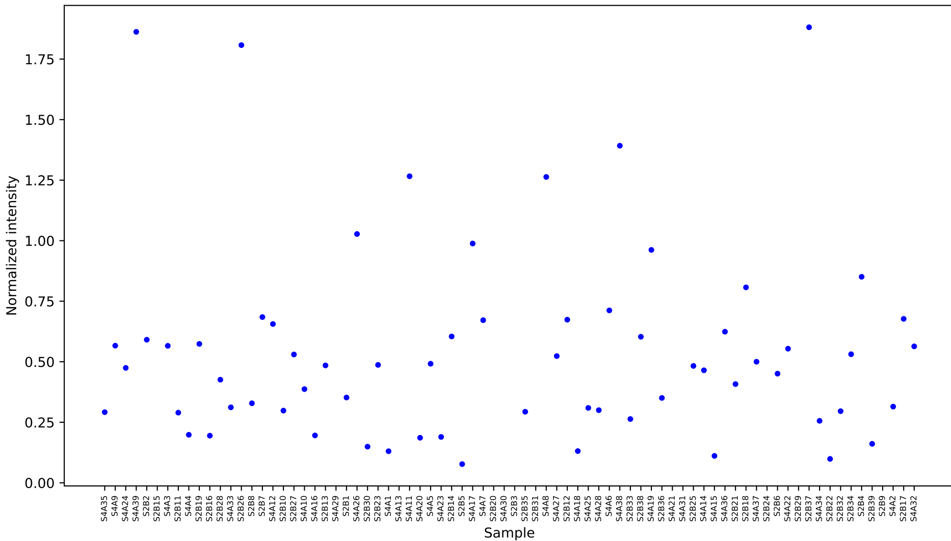
[8742] shikimic acid [16.433] Results
