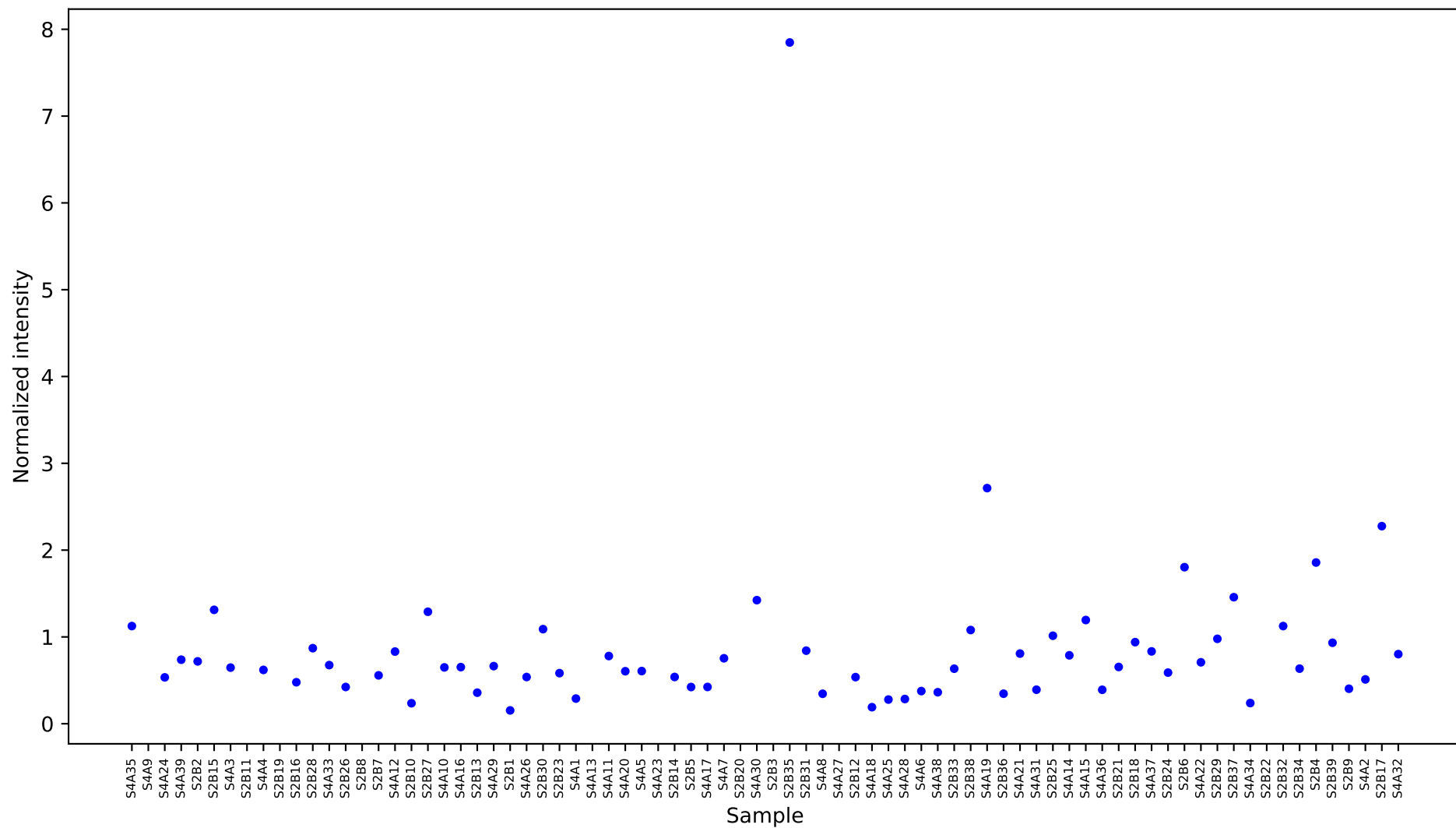
[448388] D-allose 1 [17.278] Results
