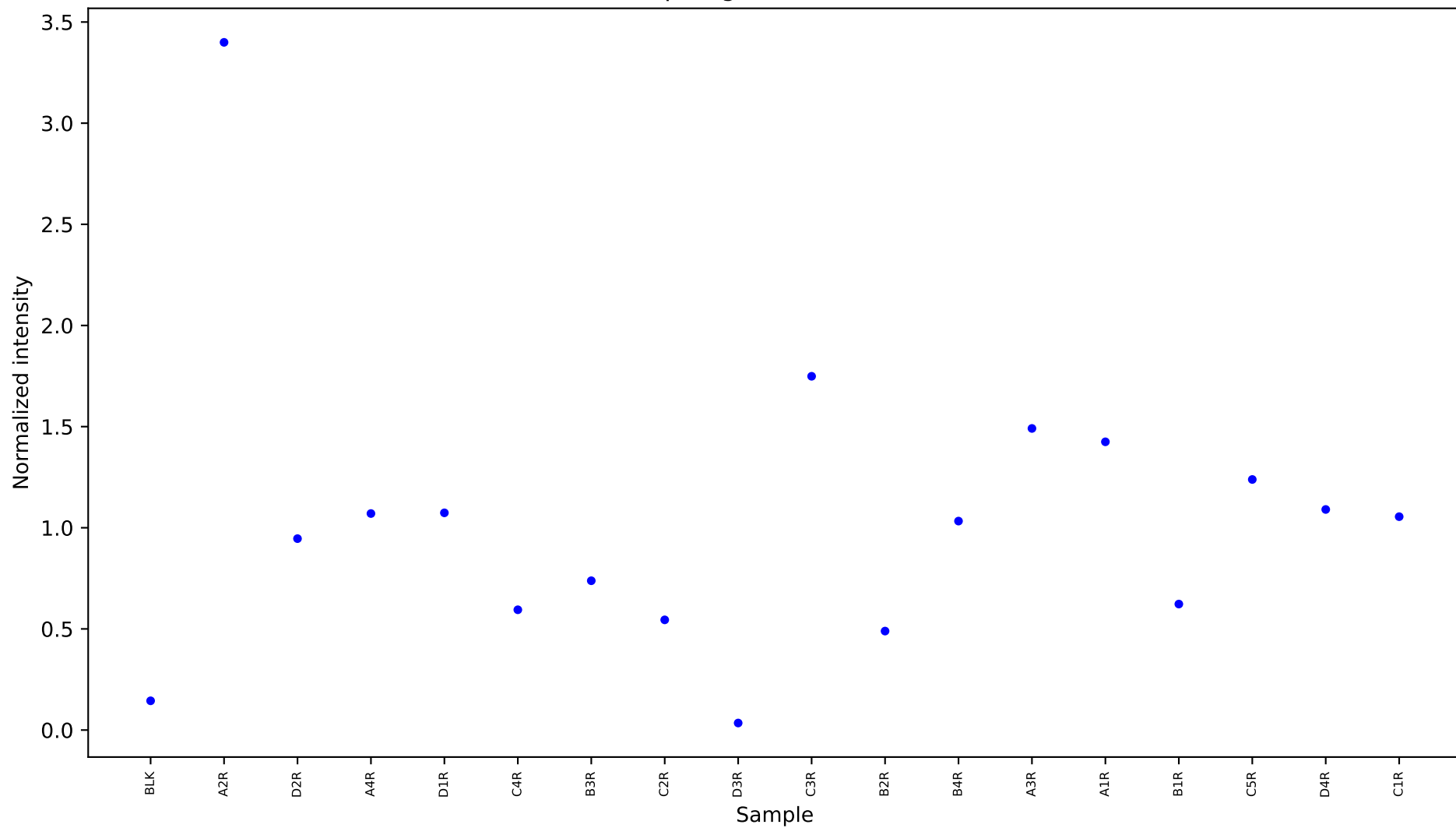
[236] L-asparagine 1 [14.496] Results
