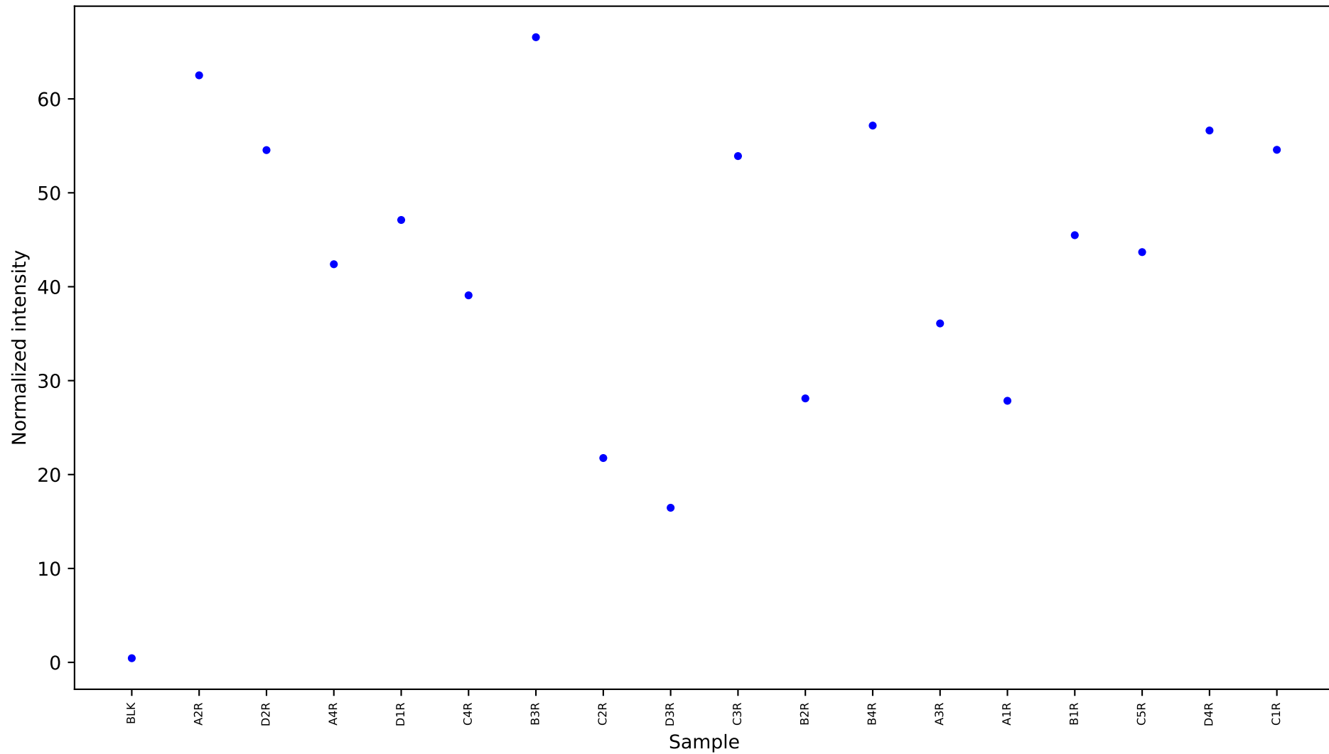
[5984] fructose 1 [17.18] Results
