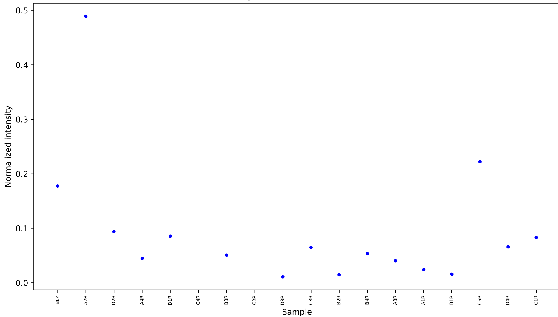
[738] L-glutamine 3 [16.092] Results
