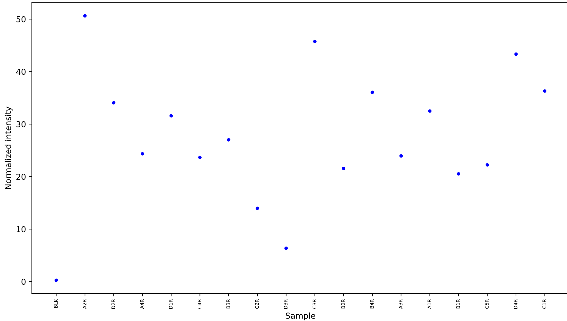
[11333] lactulose 3 [24.431] Results
