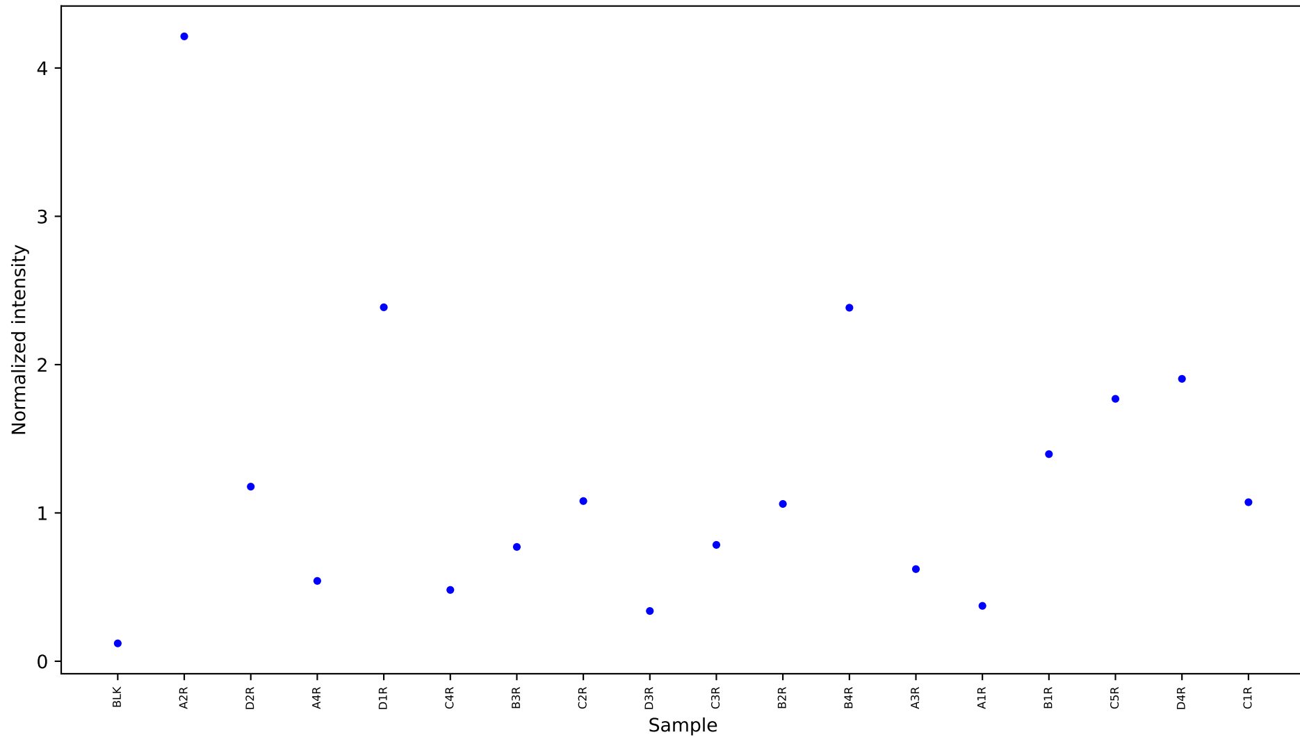
[791] DL-isoleucine 2 [10.225] Results
