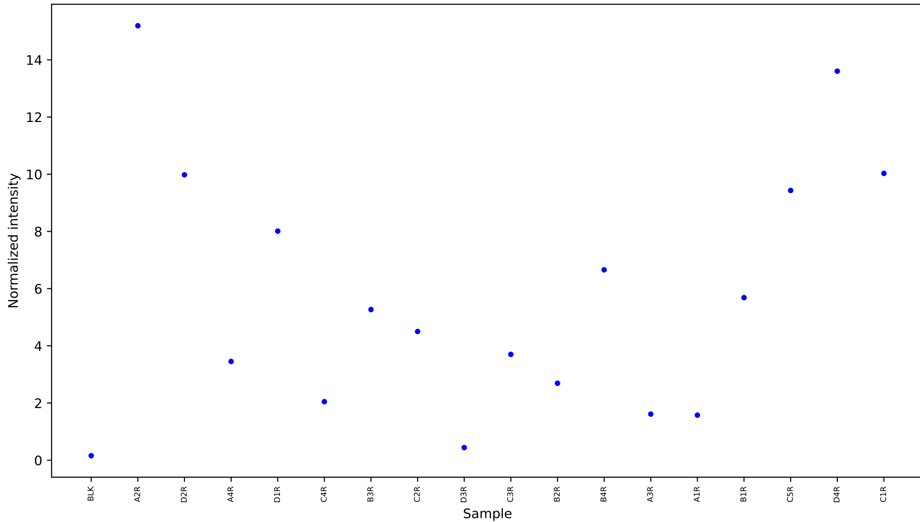
[145742] L-proline 2 [10.321] Results
