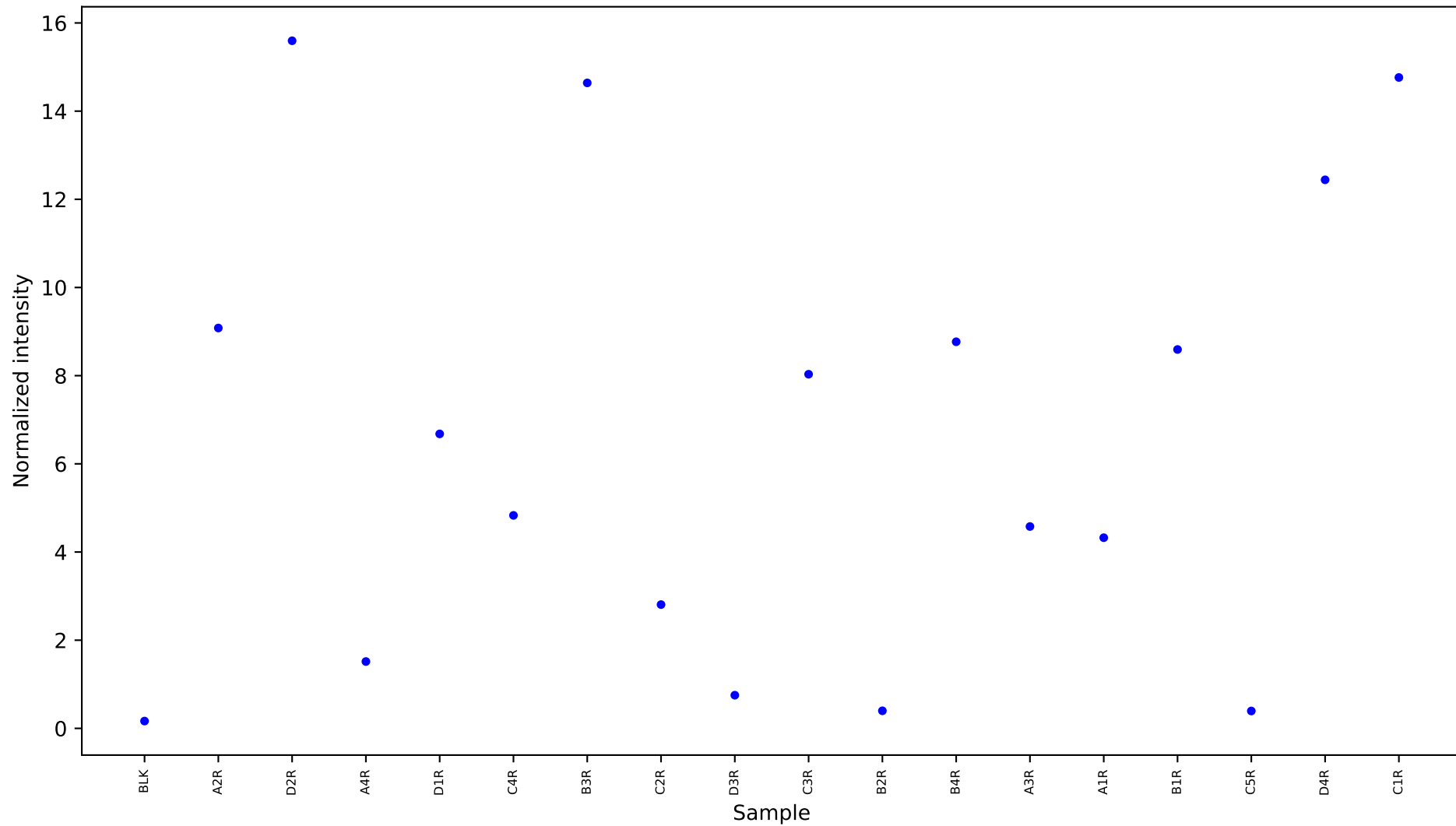
[6251] D-mannitol [17.81] Results
