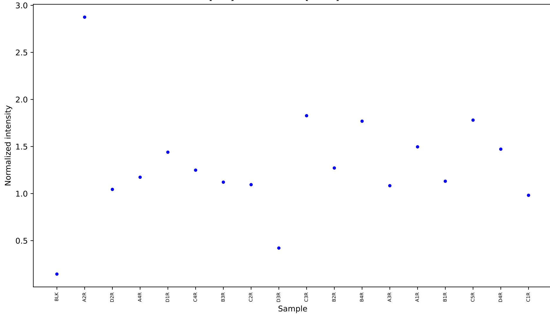
[700] ethanolamine [9.879] Results
