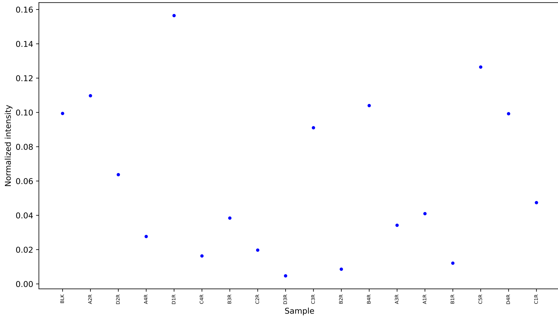
[6305] L-tryptophan 2 [20.466] Results
