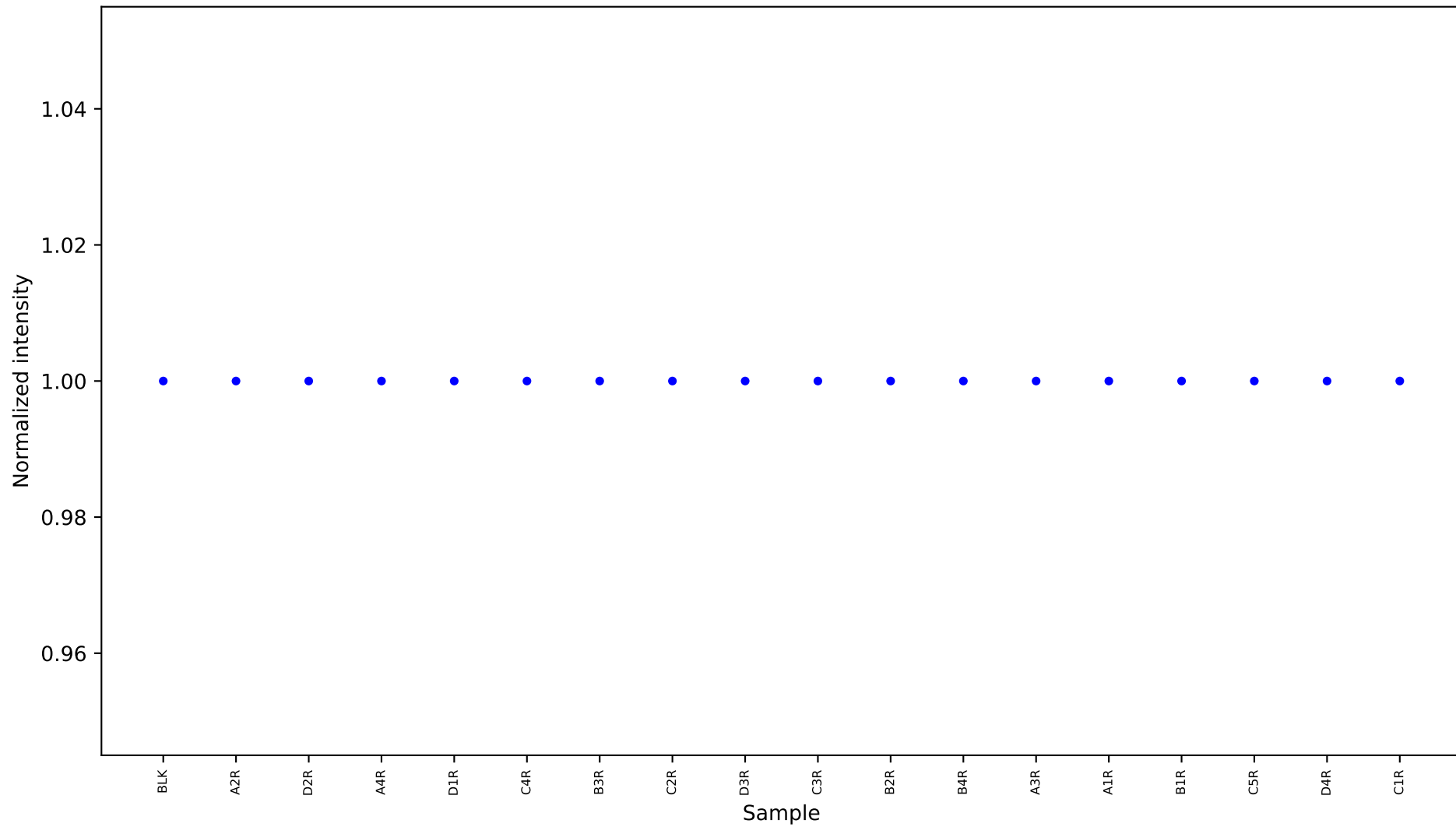
[827] ribitol [15.66] Results
