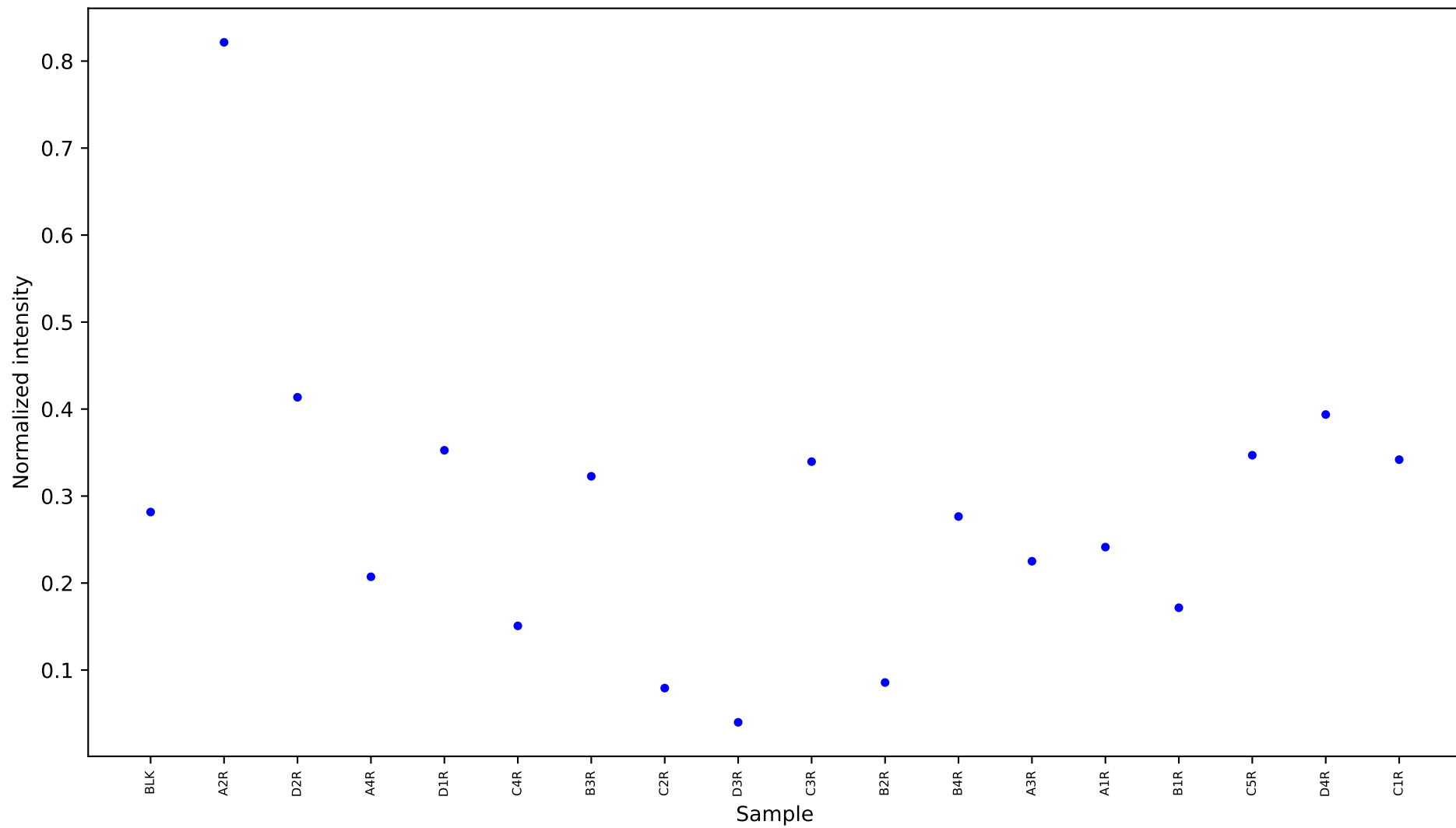
[204] allantoin 1 [17.293] Results
