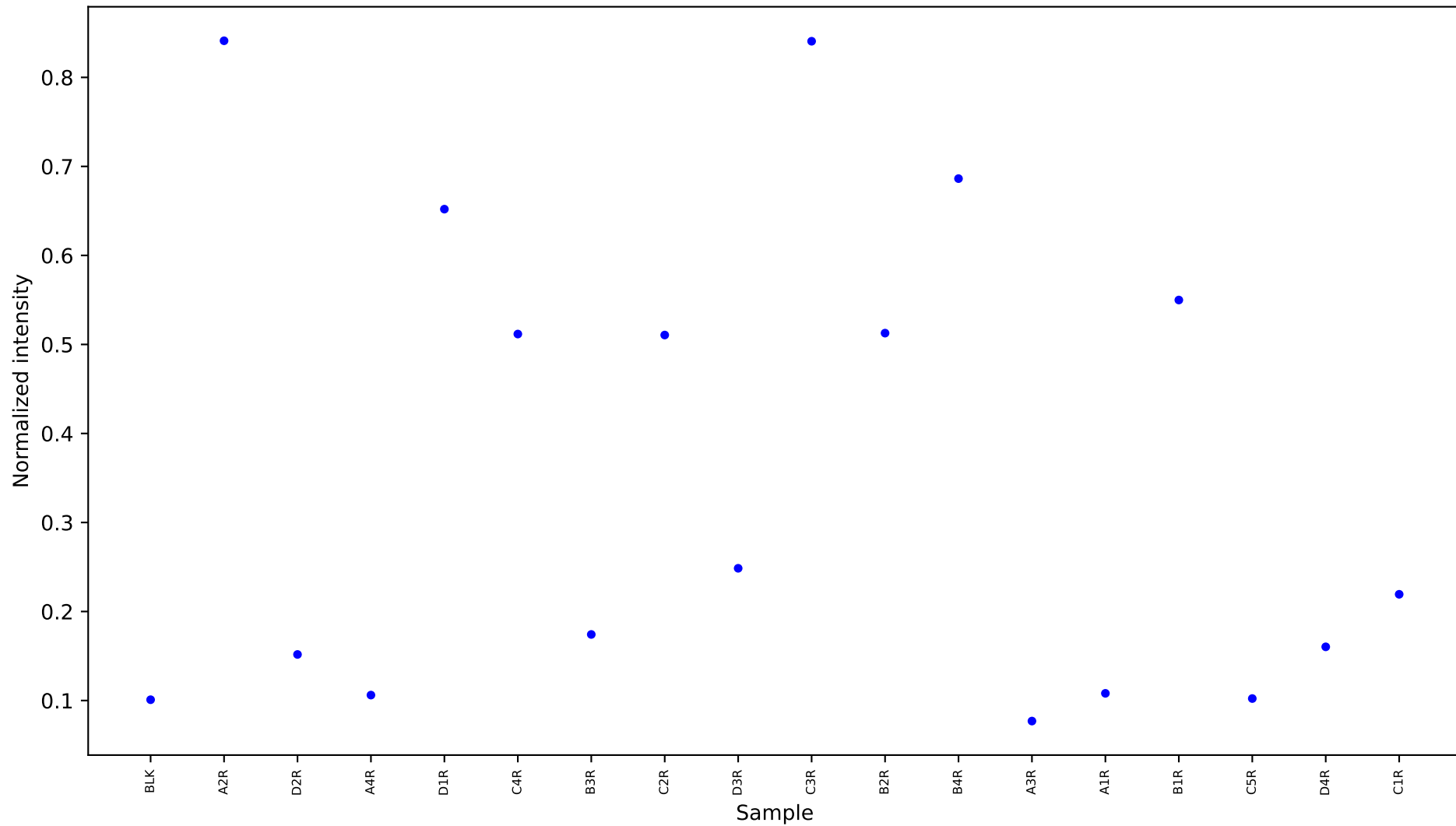
[899] N-acetyl-D-mannosamine 2 [19.339] Results
