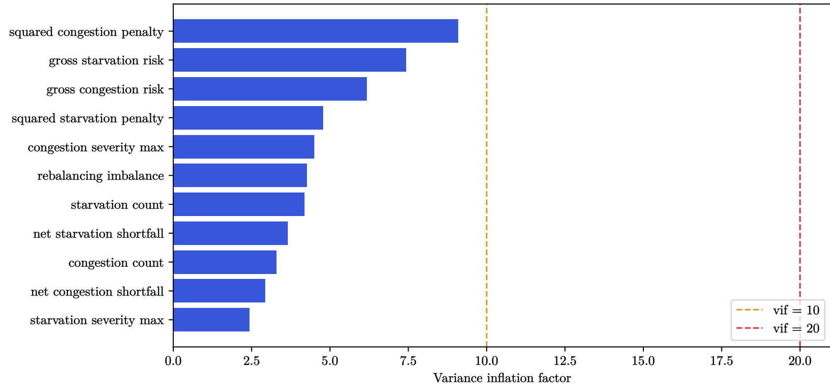
Rebalancing feature multicollinearity
