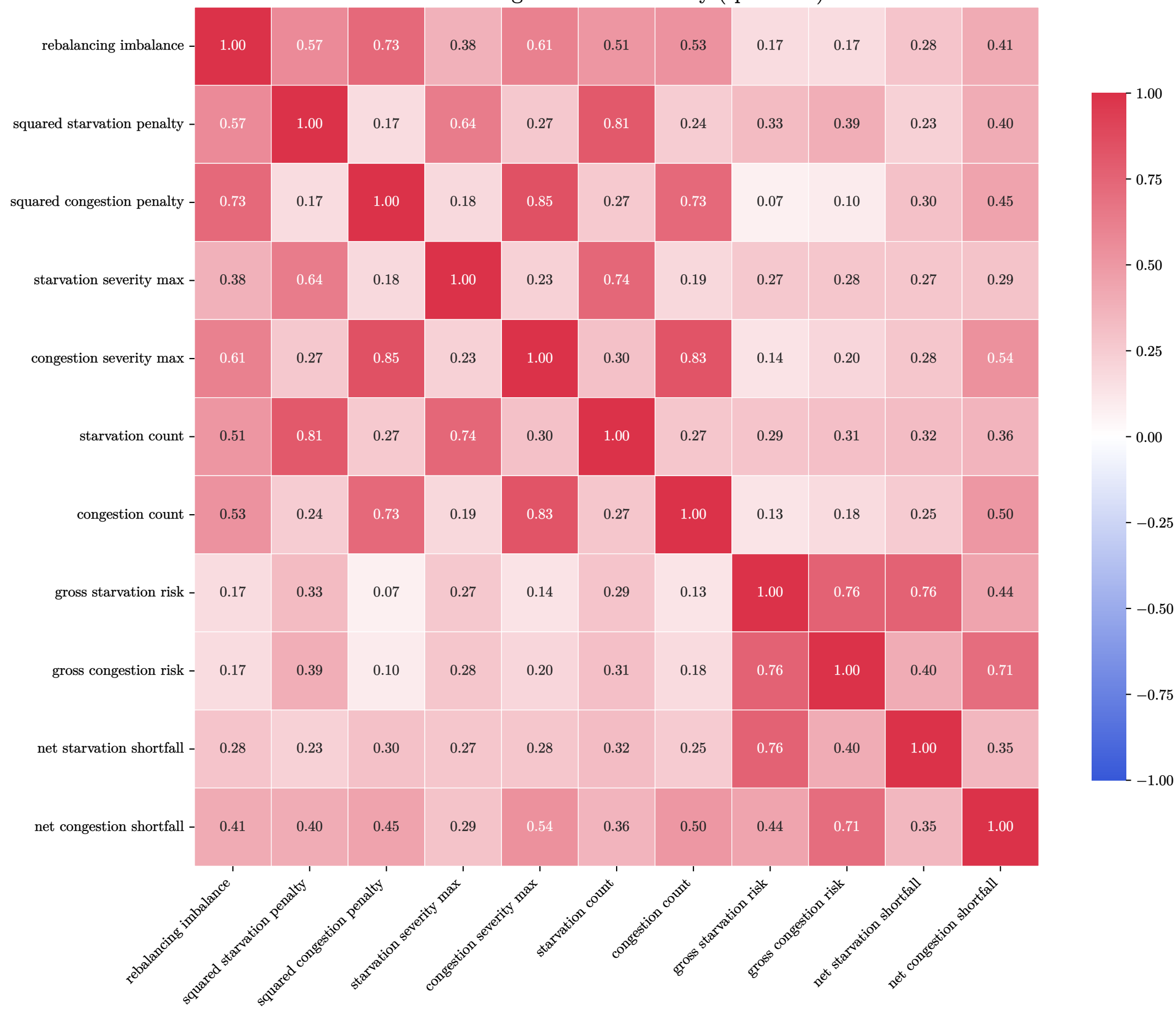
Rebalancing feature redundancy (spearman)
