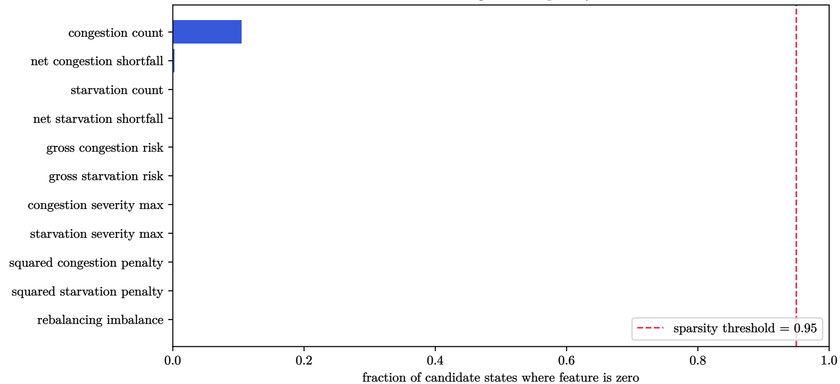
rebalancing feature sparsity
