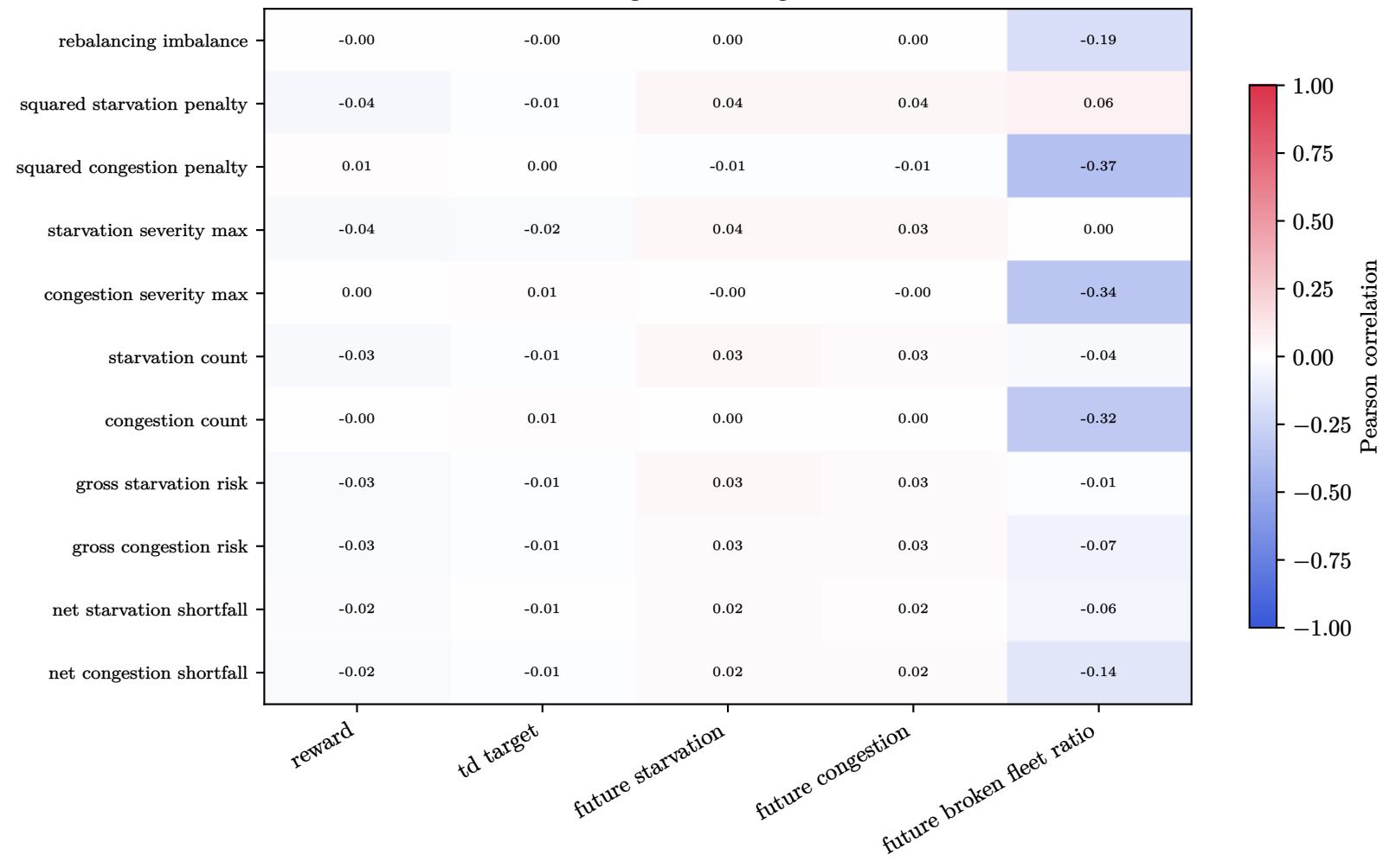
Rebalancing feature-target correlations
