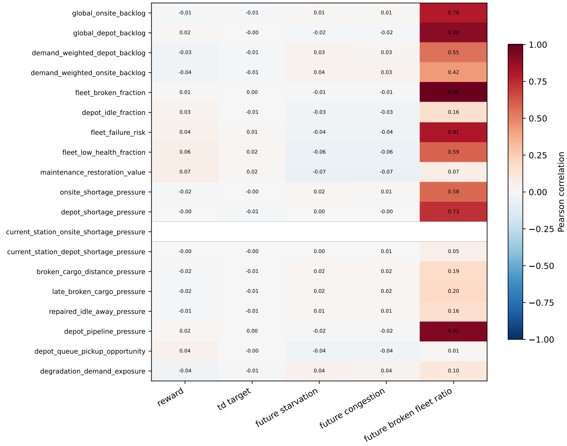
Feature-Target Correlations
